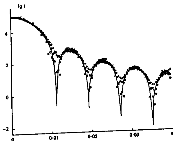
Fig. 1. Restoration of model scattering intensity of homogeneous sphere smeared by slit-width effect: — exact curve; +++ smear curve with statistical noise of 3%; xxx and ooo are desmeared curves according to Taylor & Schmidt (1967) and as obtained by the regularization technique, respectively.
