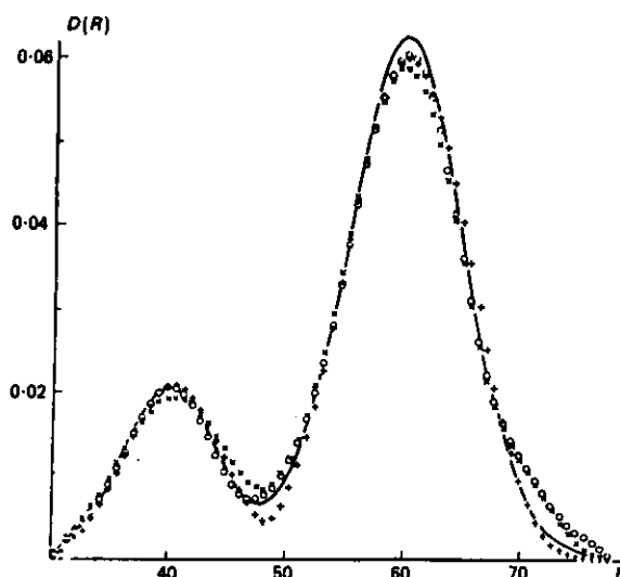
Fig. 3. Restoration of model volume distribution function for a polydisperse system of homogeneous spheres: — exact curve; ○○○ Letscher & Schmidt's (1966) method; ××× Glatter's (1977) method; +++ regularization technique.
