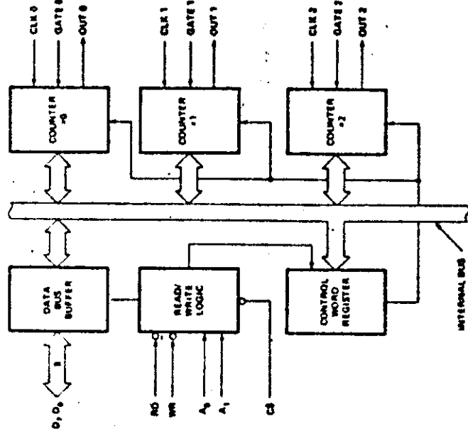
BLOCK DIAGRAM
