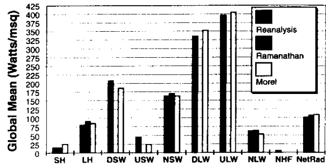
FIG. 4. (a) Global-mean radiative balance at the top of the atmosphere, and (b) surface energy budget for 1985–91 from reanalysis. Here, SH is sensible heat, LH is latent heat, SW is shortwave radiation, LW is longwave radiation, OLR is outgoing longwave radiation, D is downward, U is upward, N is net, HF is heat flux, RF is radiative flux, and Rad is radiation. Values from reanalysis are compared to two climatological estimates: Ramanathan et al. (1989) and Morel (1994).
