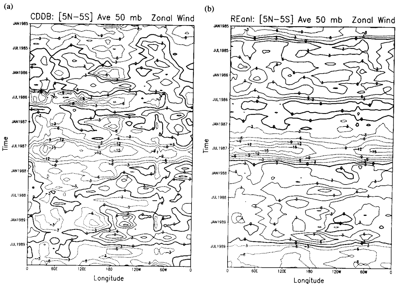
FIG. 9. a) Hovmoeller diagram (longitude–time) for the zonal wind component at 50 hPa at the equator ( 5^{\circ}\text{N} – 5^{\circ}\text{S} ), in the operational NCEP Global Data Assimilation System (from the climate diagnostics database). (b) As in (a) but for the reanalysis zonal winds.
