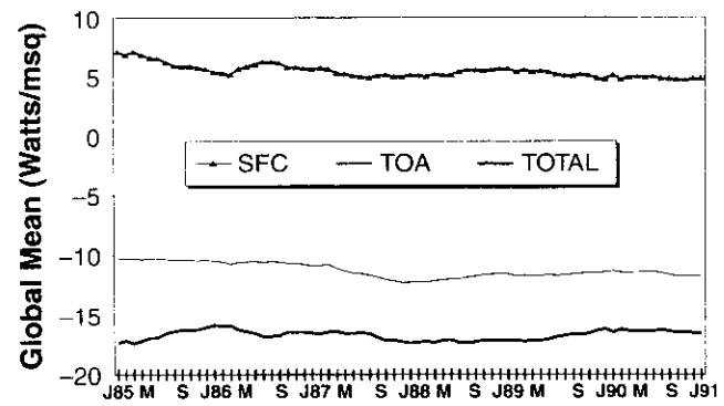
FIG. 5. (a) Monthly mean globally averaged precipitation (P) and evaporation (E), and their difference; (b) 12-mon running means of the net surface heat flux (SFC), net radiative flux at the top of the atmosphere (TOA), and the net flux out of the atmosphere (TOTAL) for 1985–91 from reanalysis.
