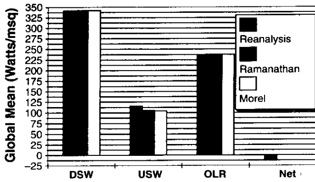
FIG. 4. (a) Global-mean radiative balance at the top of the atmosphere, and (b) surface energy budget for 1985–91 from reanalysis. Here, SH is sensible heat, LH is latent heat, SW is shortwave radiation, LW is longwave radiation, OLR is outgoing longwave radiation, D is downward, U is upward, N is net, HF is heat flux, RF is radiative flux, and Rad is radiation. Values from reanalysis are compared to two climatological estimates: Ramanathan et al. (1989) and Morel (1994).
