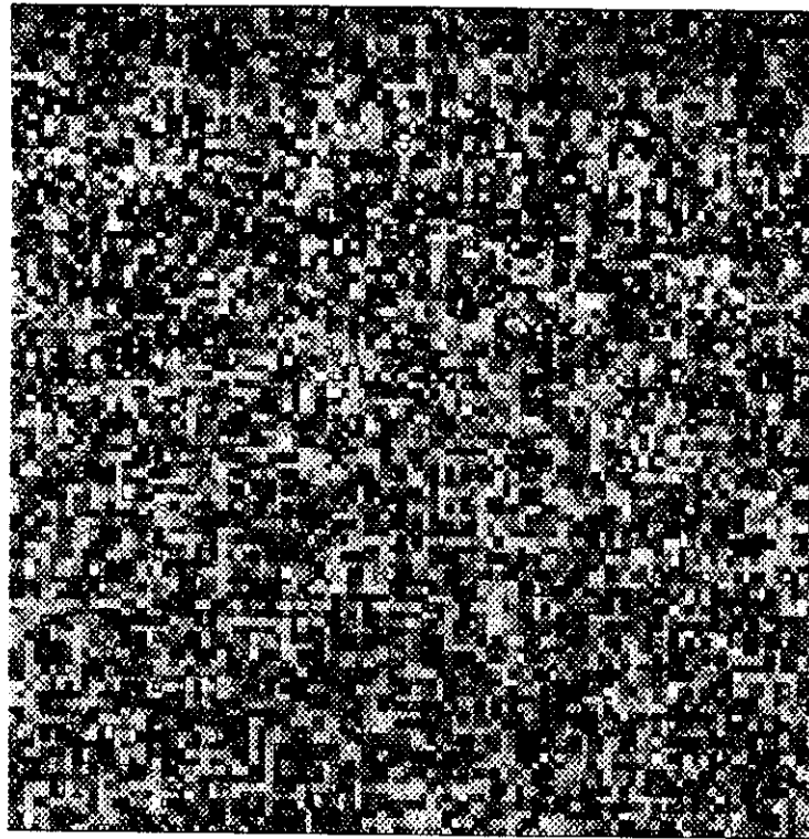
FIG. 13. Sample output from grassland simulation; snapshot of distribution of Plantago erecta . Colors denote population levels (see key).
