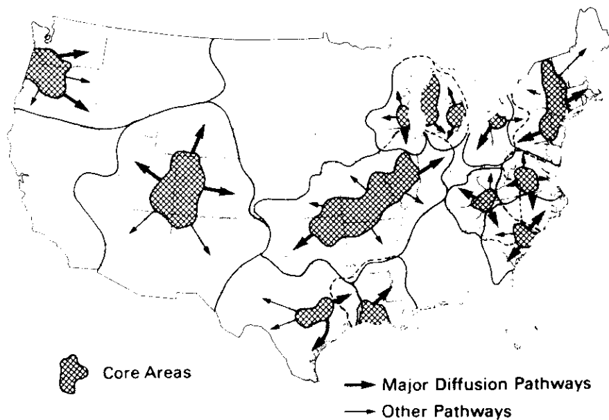
FIG. 10. Patterns of two-level spread of influenza during start of 1967-1968 season (from G. F. Pyle 1982).
