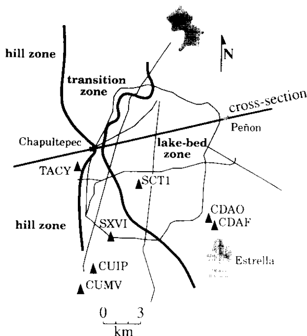
Figure 2. Map of the area of Mexico City. On the map, the locations of the strong-motion accelerometer stations are shown; these stations were operating during the 1985 Michoacan event. The locations of stations CU01 and CUIP are the same. The solid line indicates the cross section, for which 2D modeling has been performed.
