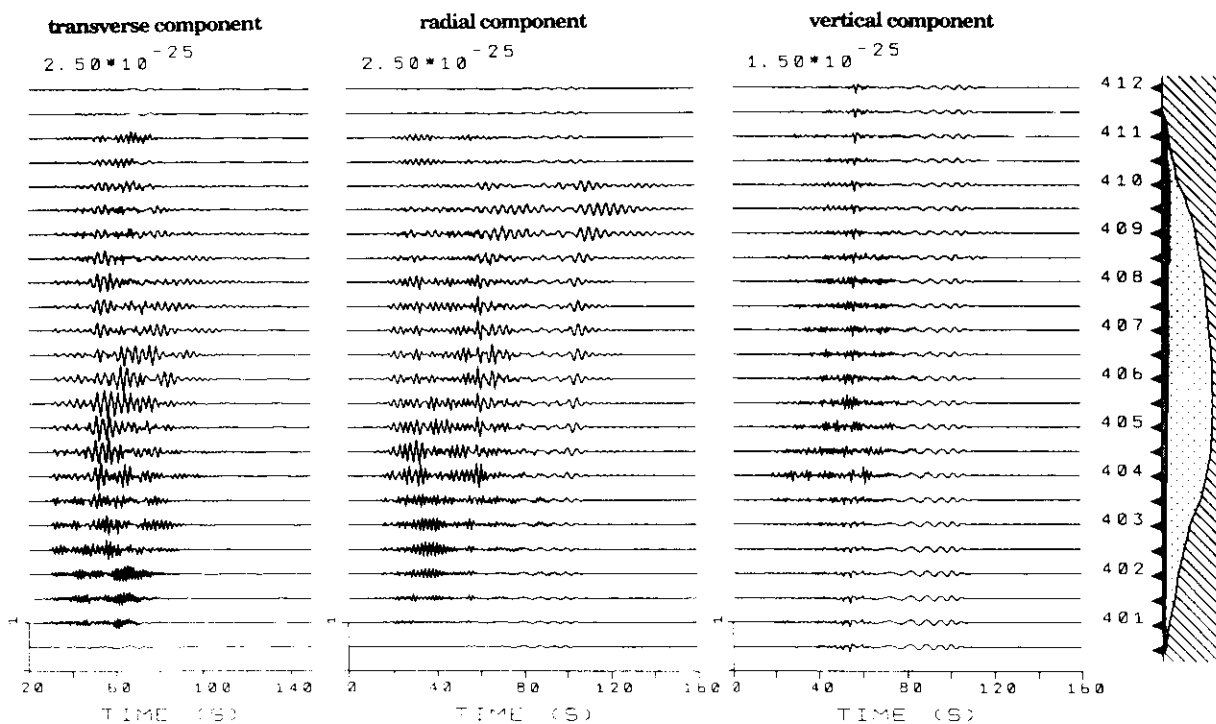
Figure 12. The same as in Figure 9 for the displacement time series, for cross section Chapultepec-Peñon shown in Figure 11. The normalization factor of the time series is different from the one used in Figure 9.
