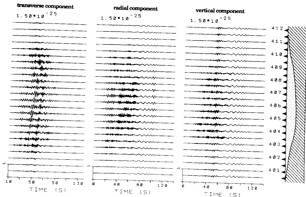
Figure 9. Displacement time series for P -SV and SH waves at an array of receivers over cross section Chapultepec-Peñon. All amplitudes are related to a source (see text) with seismic moment of 10^7 N-m. In each column, the signals are normalized to the same peak displacement. The peak displacement is indicated in units of centimeters. The time scale is shifted by 90 sec from the origin time (0 sec in the figure is in fact 90 sec from the origin time).
