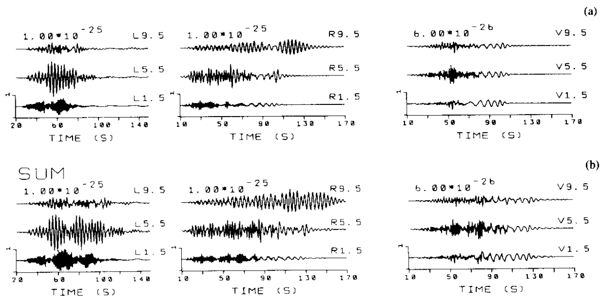
Figure 14. Transverse (left column), radial (middle column), and vertical displacements (right column) obtained at three receivers within the sedimentary basin: at the western edge of the basin, 401.5 km from the source; in the center of the basin, 405.5 km from the source; and at the eastern edge of the basin, 409.5 km from the source. The results of two computations are shown:
