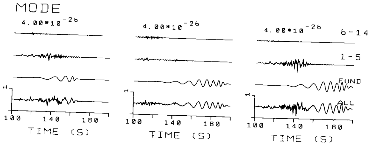
Figure 4. Transverse (left column), radial (middle column), and vertical displacements (right column) obtained for a point source (see text) in a 1D structural model (Table 1) at a distance of 400 km. All amplitudes are related to a source with seismic moment of 10^{-7} N-m. The signals are normalized to the same peak displacement. The peak displacement is in units of centimeters. Each component is decomposed into different sets of modes (upper three traces for each component: modes 6 to 14, modes 1 to 5, fundamental mode FUND).
