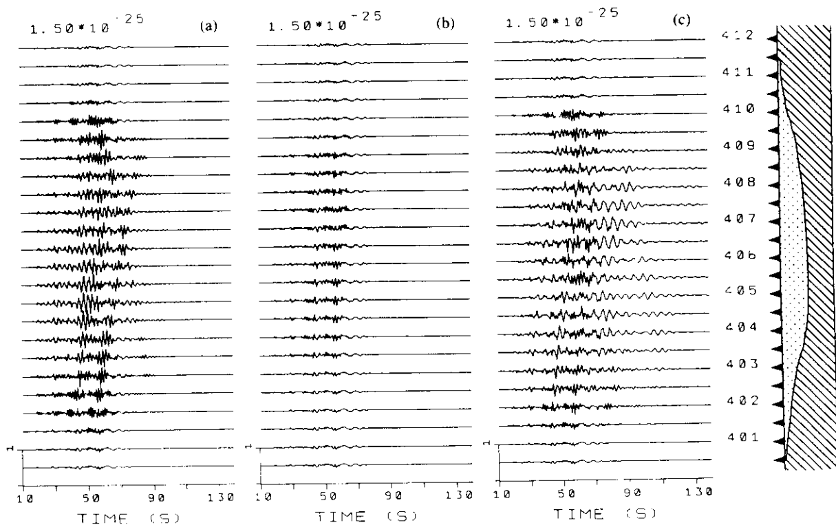
Figure 10. The same as in Figure 9 for the displacement time series for SH waves, assuming:
