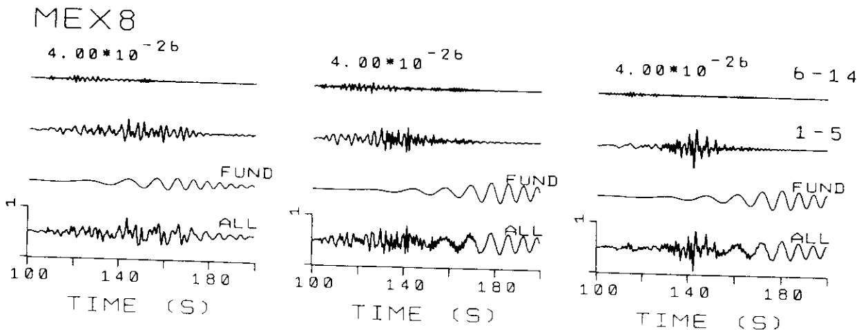
Figure 5. The same as in Figure 4, but replacing the first 400 m of the layered model (Table 1) with a surficial sedimentary layer, which represents the deep sediments (400-m thickness, \rho = 2.0 g/cm 3 , \alpha = 2.0 km/sec, \beta = 0.6 km/sec, Q_\alpha = 100 , and Q_\beta = 50 ).
