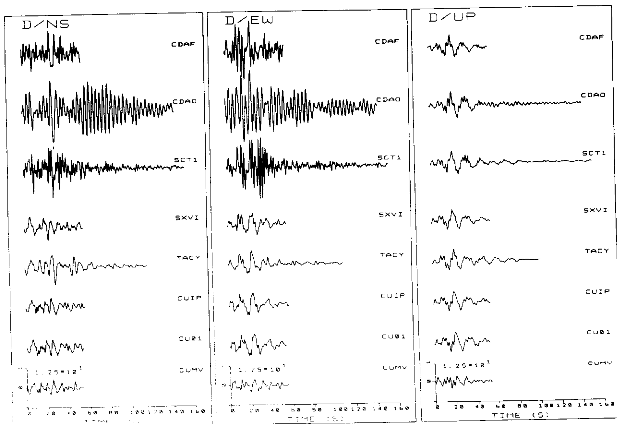
Figure 3. Horizontal and vertical components of displacement recorded in the valley of Mexico City (Mena et al. , 1986). The N-S component of motion is denoted by D/NS, the E-W component by D/EW, and the vertical component by D/UP. In each column, the signals are normalized to the same peak displacement. The peak displacement is indicated in units of centimeters.
