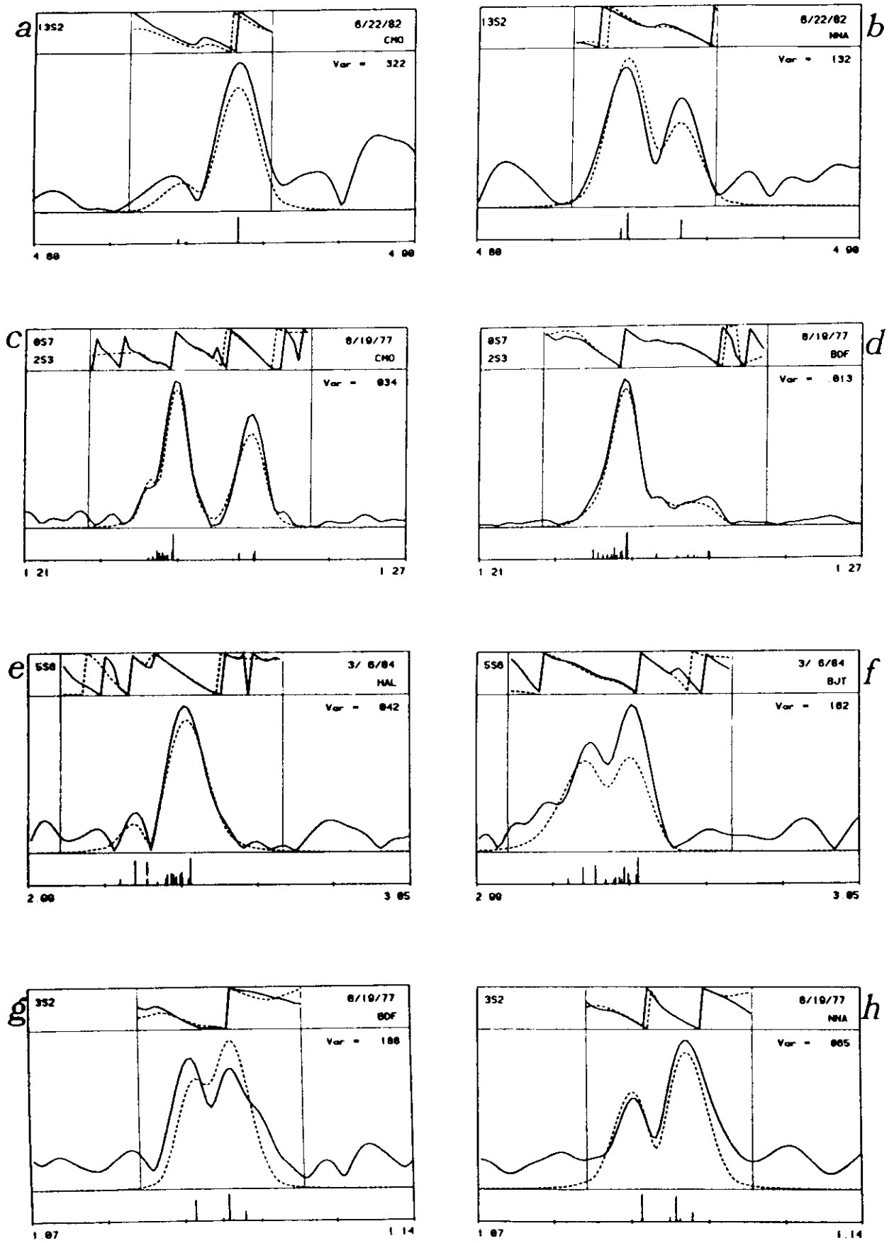
Data (solid lines) and synthetic spectra (dashed lines), as in Figure 1, but with the synthetic spectra obtained using the splitting functions of Table 4. See caption to Figure 1.
