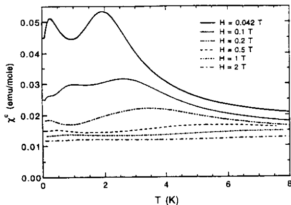
FIG. 2. ac susceptibility for H \parallel \hat{c} of copper benzoate. Note suppression of low-field paramagnetic signal with increasing field.
