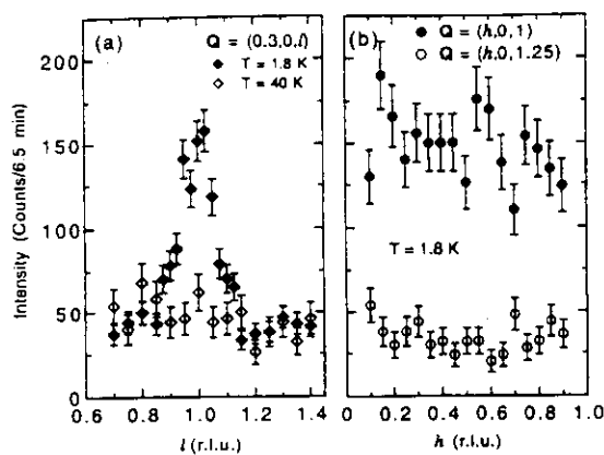
FIG. 4. Wave vector dependence of inelastic neutron scattering at \hbar\omega = 0.4 meV (a) for Q = (0.3, 0, l) varying only along the chain direction at T = 1.8 K (solid symbols) and T = 40 K (open symbols), and (b) for Q = (h, 0, 1) and Q = (h, 0, 1.25) varying only perpendicular to the chain direction at T = 1.8 K.
