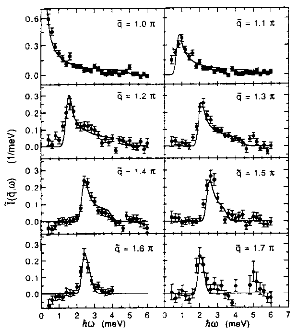
FIG. 7. Constant \bar{q} cuts through the magnetic neutron scattering data shown in Fig. 6. Solid lines are a one-parameter fit of the theory of Müller et al. (Refs. 5,6) to the entire data set.
