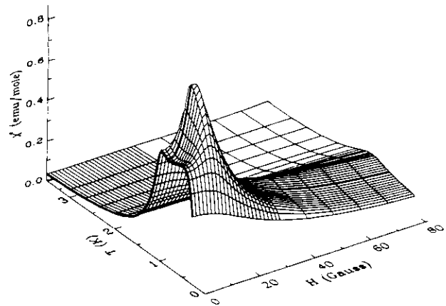
FIG. 1. ac susceptibility for H \parallel \hat{c} of copper benzoate at low field. The intersections of the grid correspond to measured points. The bold curve highlights the zero-field response.
