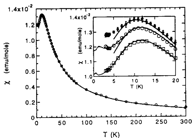
FIG. 3. High-field susceptibility of copper benzoate for H = 2 T \parallel \hat{c} . Inset: open squares, \chi^a at H = 2 T; open circles, \chi^c at H = 2 T; solid circles, \chi^c at H = 5 T. Dashed lines: low temperature susceptibility \chi^a and \chi^c at H = 2 T. Solid lines: fit with J = 1.57 meV as described in the text.
