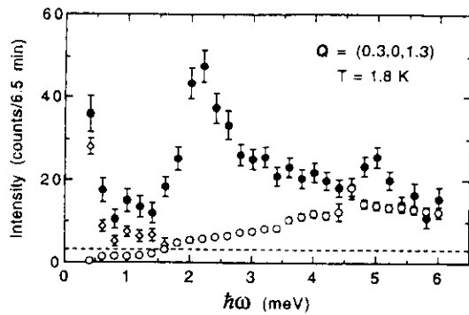
FIG. 5. Solid symbols show raw inelastic neutron scattering intensity versus energy for copper benzoate at T = 1.8 K and \mathbf{Q} = (0.3, 0, 1.3) corresponding to \bar{q} = 1.3\pi . The asymmetric peak at \hbar\omega \approx 2 meV is magnetic. The dashed line shows the average detector count rate after extracting the sample from the cryostat. Open symbols show the background contributions from incompletely resolved elastic nuclear scattering (diamonds) and from inelastic nuclear scattering (open circles) as determined by the procedures described in the text.
