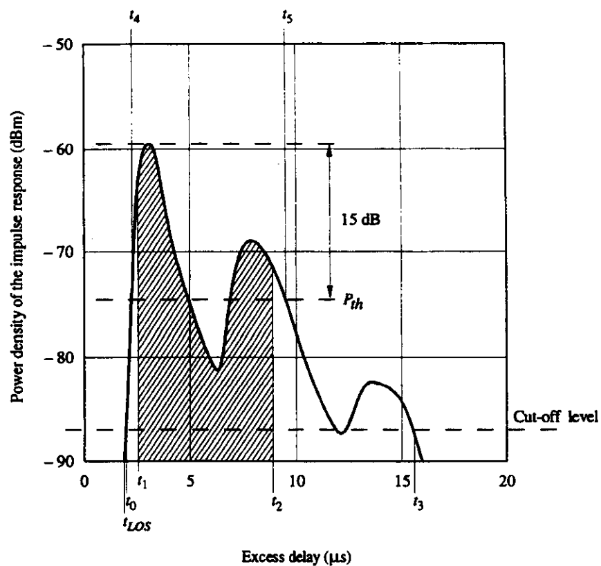
FIGURE 1 Example of an averaged delay power profile
