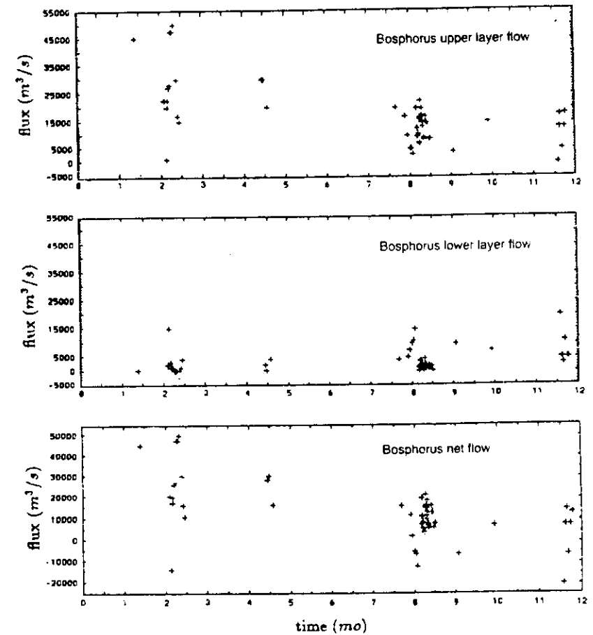
Figure 2 – 1991-1995 ADCP-based direct volume flux measurements in the Bosphorus plotted on a seasonal basis (after ÖZSOY et al. , 1994; GREGG, 1995).
