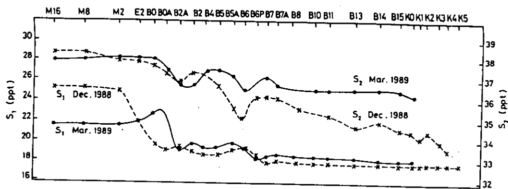
FIG. 8. Average salinities in the upper layer ( S_1 ) and in the lower layer ( S_2 ) in the Bosphorus Strait for December 1988 (x) and March 1989 (•).
