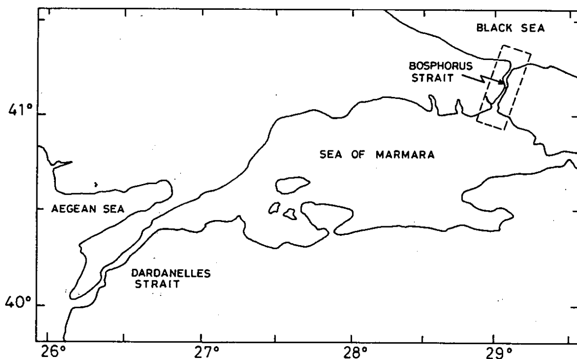
FIG. 1a. The location map for the components of the Turkish Strait System with the rectangular box showing the region under consideration in the present study.
