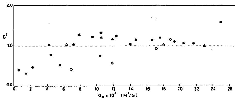
FIG. 6. Composite Froude number versus the net barotropic flow at grid point 32 for different values of friction coefficients with C_b = 0.0023 and (a): C_i = 0.0005 (○), (b): C_i = 0.0003 (■), (c): C_i = 0.0001 (●) and with (d): C_b = 0.0010 , C_i = 0.0001 (▽).
