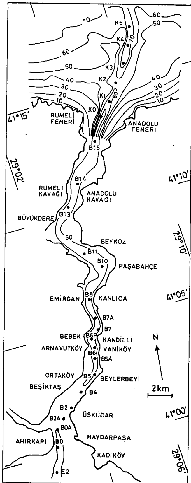
FIG. 1b. Plan view of the Bosphorus geometry and locations of the hydrographic stations.
