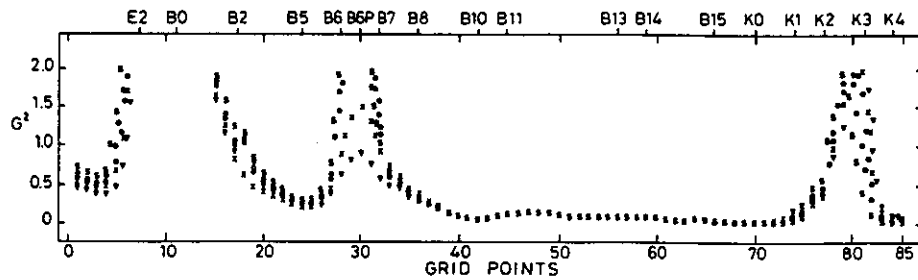
FIG. 5a. Computed variations of the composite Froude number for various values of q_0 : 4380 \text{ m}^3 \text{ s}^{-1} ( \nabla ), 10\,500 \text{ m}^3 \text{ s}^{-1} ( \times ), 12\,350 \text{ m}^3 \text{ s}^{-1} ( \bullet ), 16\,600 \text{ m}^3 \text{ s}^{-1} ( \circ ) and 21\,765 \text{ m}^3 \text{ s}^{-1} (s).
