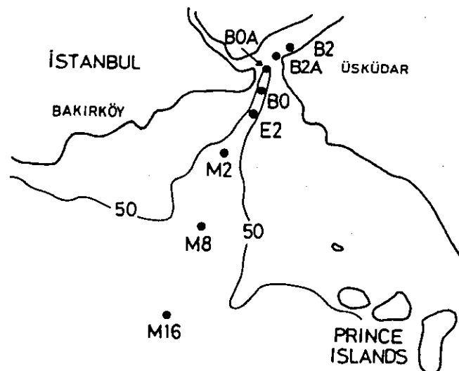
FIG. 1c. Plan view of the Marmara exit region of the Bosphorus Strait and locations of the hydrographic stations referred to in the text.
