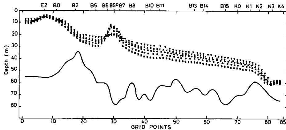
FIG. 5b. Computed variations of the interface depth for various values of q_0 : 4380 \text{ m}^3 \text{ s}^{-1} ( \nabla ), 10\,500 \text{ m}^3 \text{ s}^{-1} ( \times ), 12\,350 \text{ m}^3 \text{ s}^{-1} ( \bullet ), 16\,600 \text{ m}^3 \text{ s}^{-1} ( \circ ) and 21\,765 \text{ m}^3 \text{ s}^{-1} (s).
