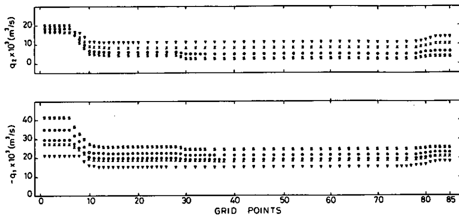
FIG. 7a. Computed variations of the upper and lower layer transports for values of q_0 : 4380 \text{ m}^3 \text{ s}^{-1} ( \nabla ), 10\,500 \text{ m}^3 \text{ s}^{-1} ( \times ), 16\,600 \text{ m}^3 \text{ s}^{-1} ( \circ ) and 21\,765 \text{ m}^3 \text{ s}^{-1} (s).
