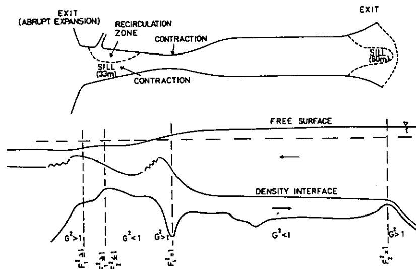
FIG. 11. Schematic picture of the Bosphorus internal hydraulics.
