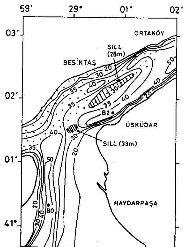
FIG. 2. Bathymetry of the southern exit region of the Bosphorus Strait.
