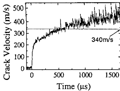
FIG. 3. A typical measurement of the velocity of a crack tip as a function of time. After an initial jump to about 150 m/s, the crack accelerates smoothly up to the critical velocity of v_c = 340 m/s. Above v_c strong oscillations in the velocity of the crack are observed.
