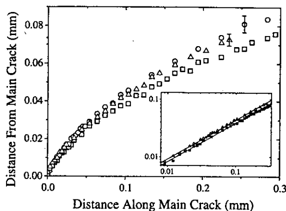
FIG. 12. The mean profile of microbranches obtained for different propagation velocities: 374 m/s (squares), 407 m/s (triangles) and 470 m/s (circles). As the velocity increases, the 0.7 exponent remains, while the coefficient of the mean profile increases (0.18 at 374 m/s, 0.2 at 470 m/s). This is demonstrated in the inset for v = 374 m/s (squares) and 470 m/s (triangles) on a log-log scale. In addition, the scatter, as indicated by the error bars, increases with the mean propagation velocity.
