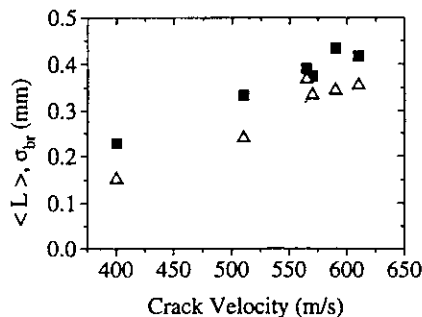
FIG. 10. The mean, \langle L \rangle (squares), and standard deviation, \sigma_L (triangles), of the branch length distribution as a function of the crack velocity. Both increase linearly with the crack velocity and have the same slope. Thus, the entire distribution scales linearly with the velocity.
