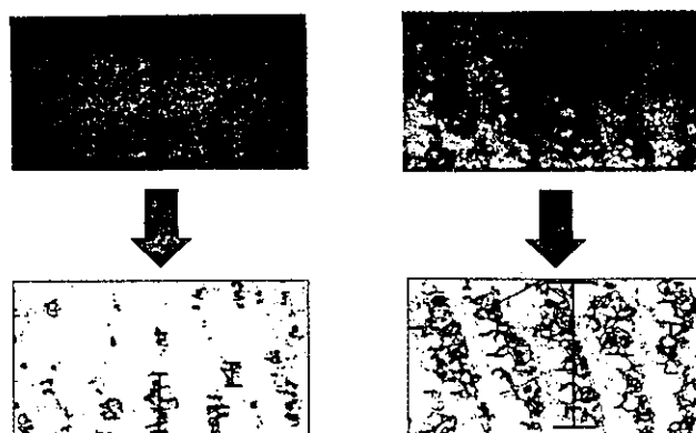
FIG. 18. A photograph of a typical fracture surface (top) and the same pictures after image processing (bottom). The clear difference between the morphology of the "cleavage zones" and the rest of the surface, provides a simple way of measuring their width, as demonstrated on the processed pictures. The random spread of the "cleaved islands" apparent at v \sim v_c (left) turns into a periodic pattern at higher velocities (right), as the width of the "cleavage zones" increases to of the order of the plate's thickness.
