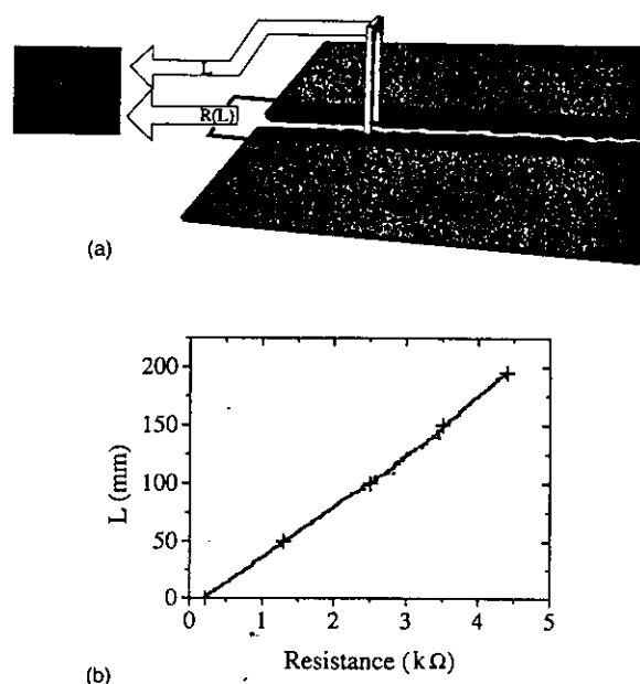
FIG. 2. (a) Resistance calibration system. An electric contact connecting opposing points of the conductive layer which were separated by the crack, is pulled quasistatically along the crack's path. The resistance, R of the conductive strip is thus measured as a function of the location of the electric contact ( L ). Inhomogeneities in the conductive layer, as well as deviations of the crack from a straight line, will cause a nonlinear R(L) profile. This profile is used to calibrate the dynamic fracture measurement (see Fig. 1). (b) A typical calibration measurement. The resistance measurements (squares) are fitted by a fifth-order polynomial (solid line). The crosses shown are calibration points obtained by the use of discrete conductive strips, located on the opposite face of the plate, and cut by the crack as it progresses across the plate.
