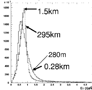
Neutrino spectra at diff. dist
