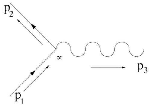
FIG. 12: pair annihilation
