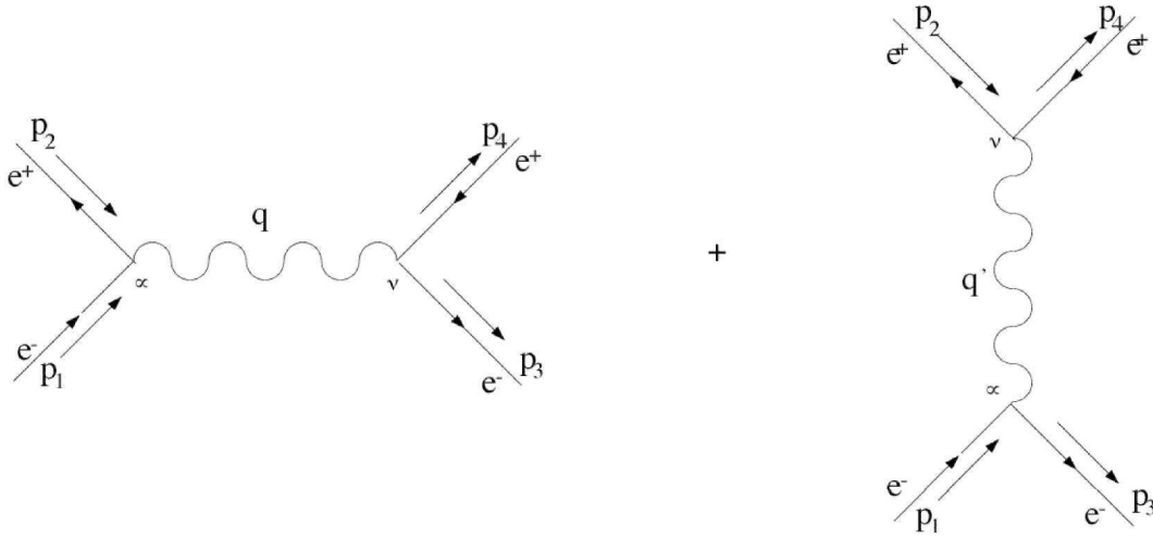
FIG. 1: Bhabha scattering
