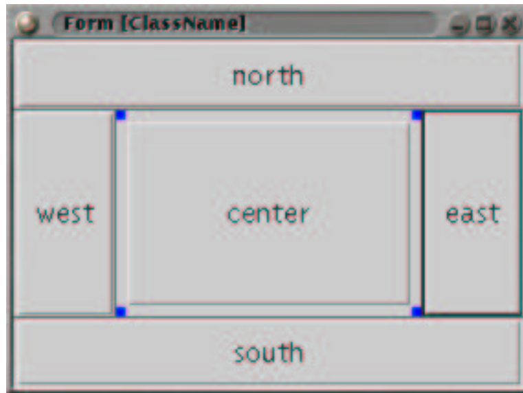
Figure 16: The BorderLayout
