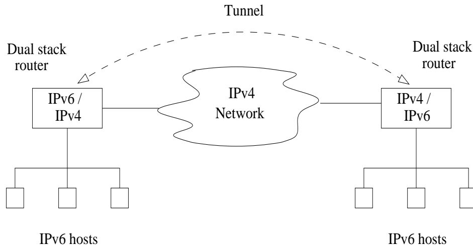
Figure 30: IPv6 Tunnelling over a IPv4 Network
