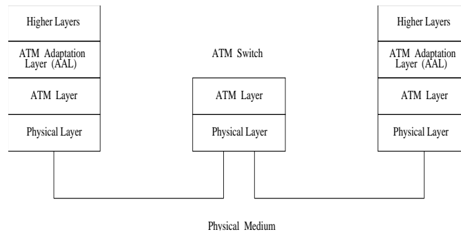
Figure 34: ATM Protocol Architecture
