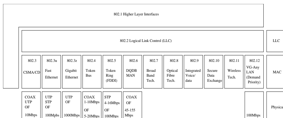
Figure 6: The Architecture of IEEE 802 LAN/MAN Standards
