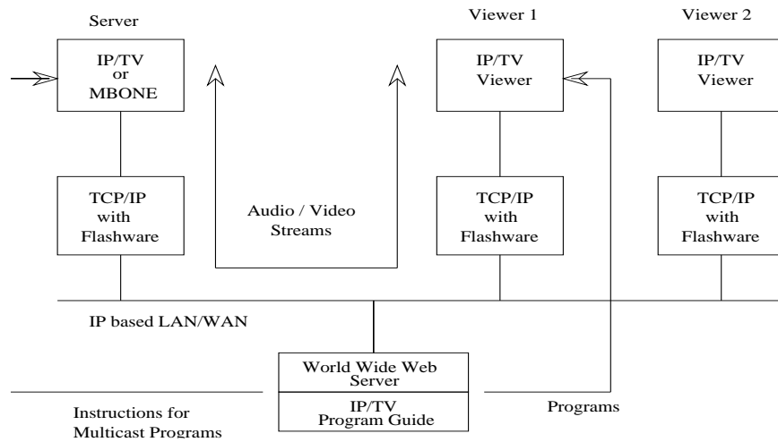
Figure 37: Real Time Audio/Video Over IP based LAN/WANs
