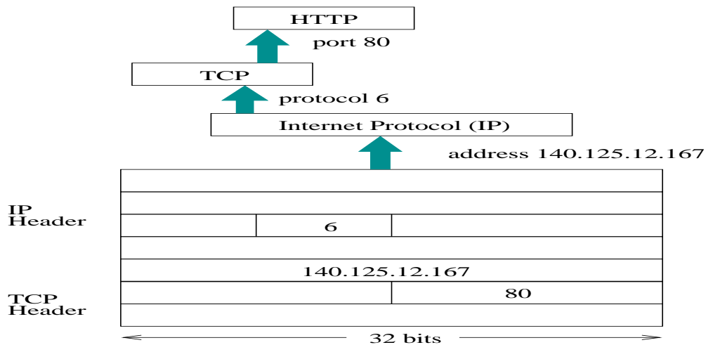
Figure 22: Mapping of Protocol and Port Numbers
