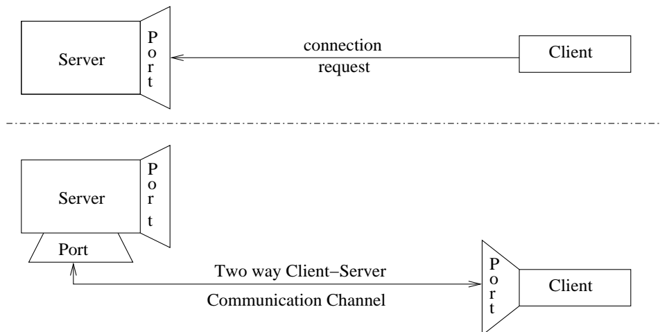
Figure 23: Socket Creation
