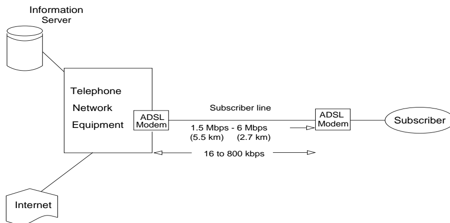
Figure 40: ADSL Channels
