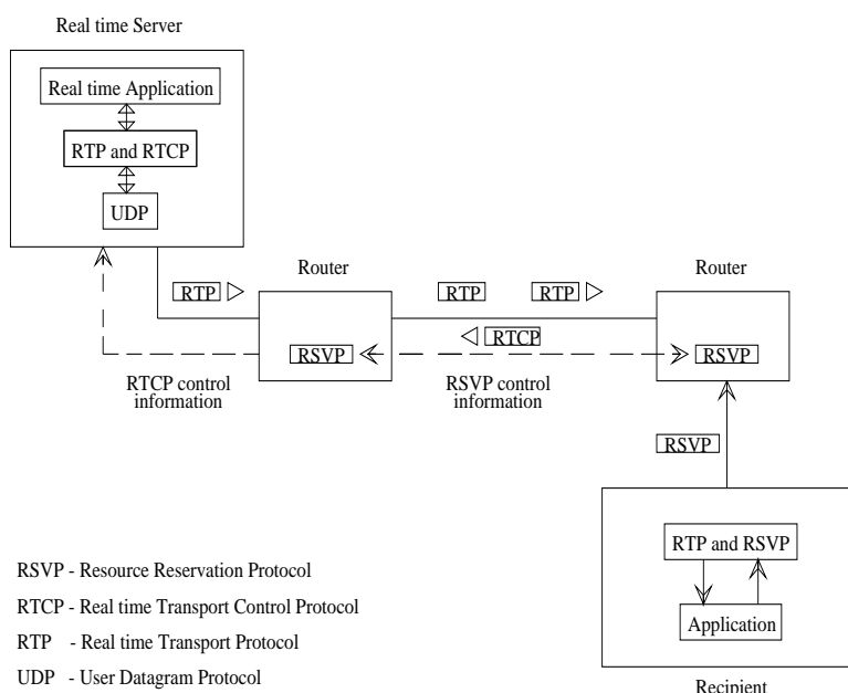
Figure 31: Real Time Application running RTP on top of UDP
