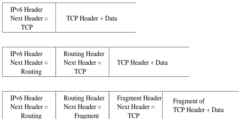
Figure 26: Chaining of IPv6 Headers
