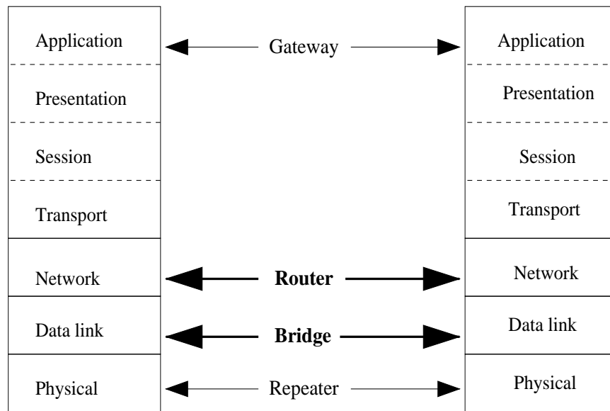
Figure 9: Interconnection Components
