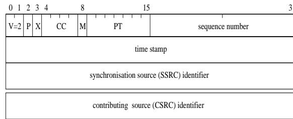
Figure 32: RTP Header Format
