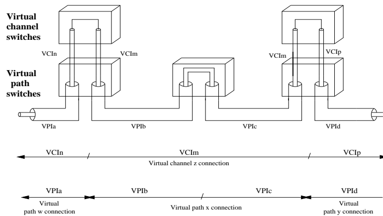
Figure 35: VC/VP Switching in ATM
