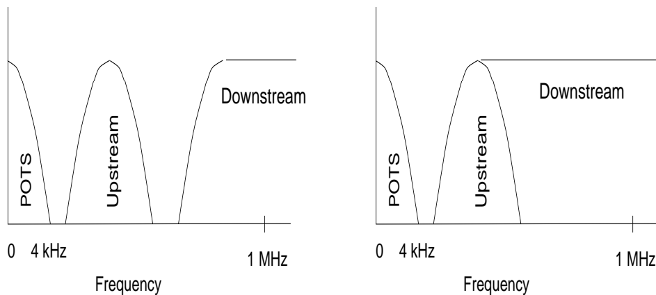
Figure 41: Creating ADSL Channels by (i) FDM and (ii) Echo Cancellation
