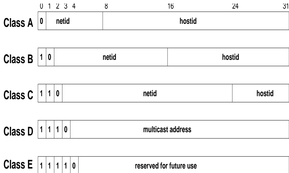
Figure 14: IP Addresses
