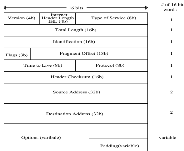
Figure 18: IP Datagram Format
