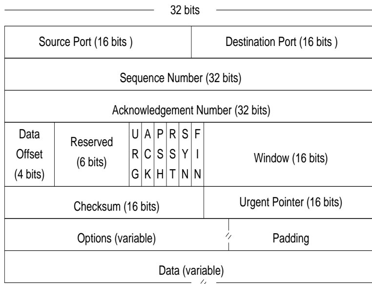
Figure 19: TCP Segment Format
