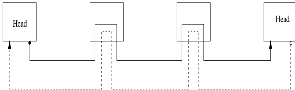
Figure 7: Open Bus DQDB Network
