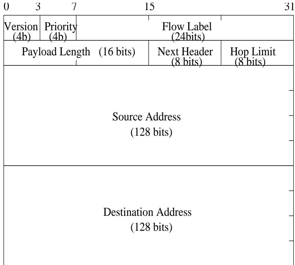
Figure 25: The IPv6 Header Format
