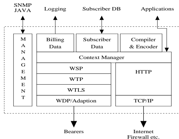
Figure 42: Layered Architecture of the WAP Gateway
