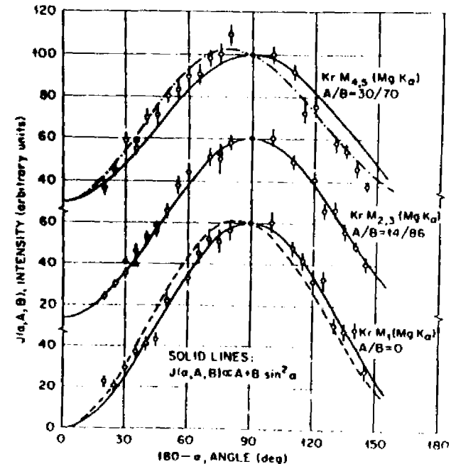
Fig. 10. Experimental angular distributions of 3s ( -M_1 ), 3p ( -M_2, 3 ), and 3d ( -M_1, 5 ) photoelectrons excited from gaseous Kr with MgK \alpha x-rays. The curves represent least-squares fits to the data points of a relationship of the form of Eq. (93), in which A and B were treated as empirical constants. (From Krause, ref. 142.)
