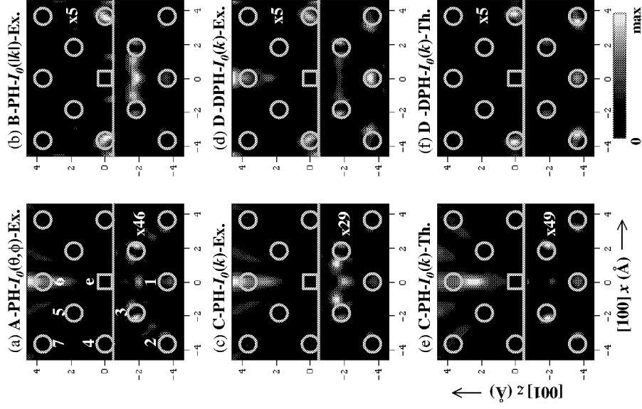
Figure 3. Atomic images in the vertical (100) plane of Cu(001) reconstructed from Cu 3p holograms obtained by normal photoelectron holography (PH, methods A–C) and differential photoelectron holography (DPH, method D), as described in the text. The emitter and scatterer positions are indicated by squares and circles, respectively, and various near-neighbour atoms are numbered. Image intensities above or below z_c = -0.5 \text{ \AA} have been rescaled by the factor shown in each panel, with this factor being determined so as to make the maximum intensities above and below z_c equal. Experimental images: (a) image obtained by method A; normal holography via equation (1) with I_0 determined by fitting its angular variation at each k value. (b) Image obtained by method B; normal holography with I_0 determined by fitting its k variation along each direction. (c) Image obtained by method C; normal holography with I_0 determined by fitting both its angular and k variations. (d) Image obtained by method D; differential holography with I_0 determined by fitting both its angular and k variations. Theoretical images: (e) as (c) but theoretical. (f) As (d) but theoretical.
