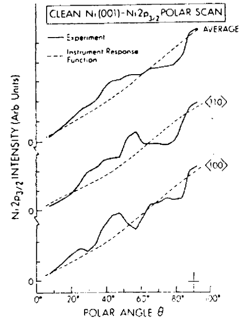
Fig. 17. Polar-scans of \text{Ni}2p_{3/2} intensities above a (001) Ni surface. Shown are two scans along the symmetry-inequivalent azimuths ( 100 ) and ( 110 ), together with an average of these two scans. Before averaging strong diffraction features are evident. Also shown is the instrument response function (cf. Fig. 11). (From ref. (33).)
