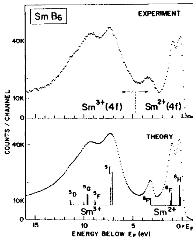
Fig. 35. Experimental and theoretical 4f valence spectra from \text{SmB}_6 , a "mixed-valence" metallic compound believed to contain both \text{Sm}^{2+}4f^6 and \text{Sm}^{3+}4f^5 . The intensities of the various final-state multiplets for \text{Sm}^{2+} \rightarrow \text{Sm}^{2+} and \text{Sm}^{3+} \rightarrow \text{Sm}^{3+} were computed using fractional parentage coefficients and are indicated as vertical bars. These calculations were broadened by an empirically-derived function of the form of Eq. (158) to generate the final theoretical curve. Monochromatized AlK \alpha was used for excitation. (From Chazalviel et al. , ref. 266.)
