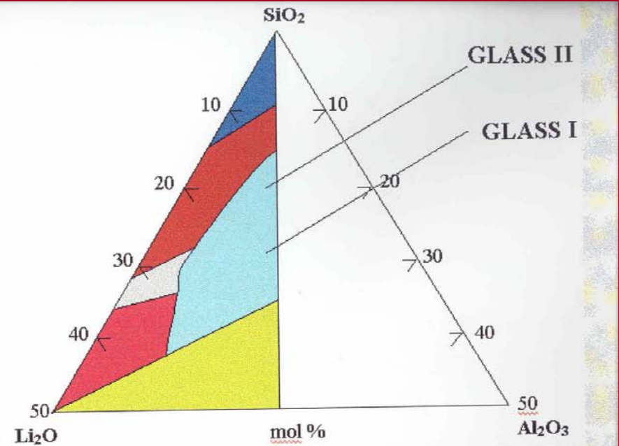
TERNARY PHASE DIAGRAM AND EQUILIBRIUM STRUCTURES
