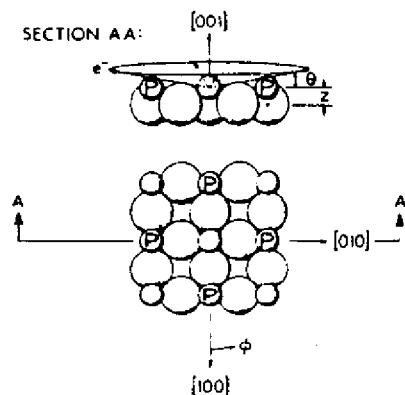
Fig. 43. General atomic geometry for c(2 \times 2) and p(2 \times 2) adsorbate overlayers on a {001} surface of an fcc metal, assuming that adsorption is in fourfold-hollow sites. In c(2 \times 2) , all sites are occupied; in p(2 \times 2) only those denoted by "P".
