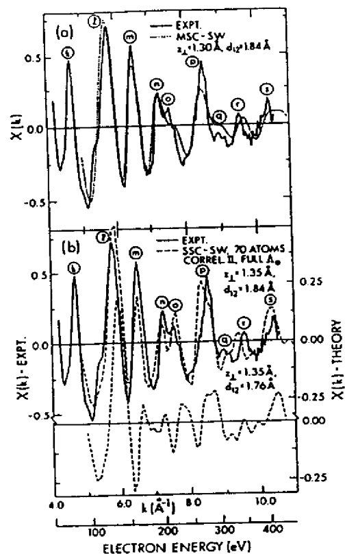
FIGURE 19. Comparison of scanned-energy S 1s data for c(2 \times 2) S on Ni (001), \theta_{\text{inc}} = 70^\circ , \theta_{\text{em}} = 0^\circ (From Ref. 8) with: (a) a multiple-scattering cluster spherical-wave (MSC-SW) calculation due to Barton and Shirley (From Ref. 25), and (b) single-scattering cluster spherical wave (SSC-SW) calculations due to Sagurton et al. (From Ref. 21). Both the sulfur vertical distance z and the first Ni-Ni interplanar distance d_{12} are specified. (Fig. from Ref. 21.)
