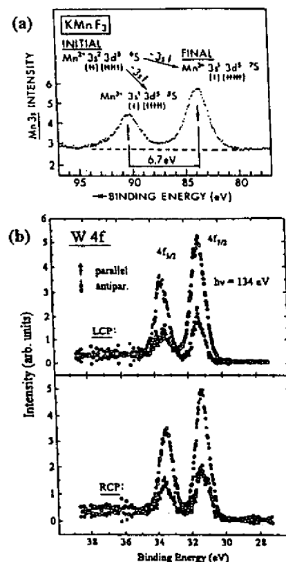
Fig. 11. Spin-polarized core photoelectron spectra: (a) a Mn3s spectrum from \text{KMnF}_3 , with the electronic states and spin polarizations relative to the emitting \text{Mn}^{2+} ion indicated (from Ref. [9e]); (b) a W4f spectrum from W(110), excited by LCP light (top panel) and by RCP light (bottom panel). In (b), the spin-resolved intensities as measured parallel or antiparallel to the light incidence direction \theta are indicated. (From Ref. [39].)
