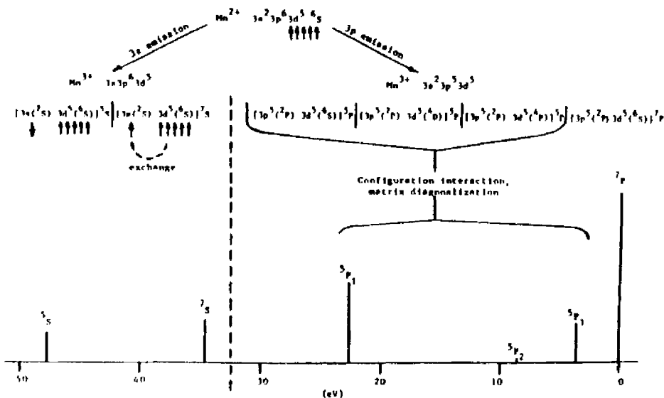
Fig. 30. The various final state L, S multiplets arising from 3s and 3p photoemission from a Mn 2+ ion. Within the S and P manifolds, separations and relative intensities have been computed using simple atomic multiplet theory as discussed in the text. The separation and relative intensity of the 7 S and 7 P peaks were fixed at the values observed for 3s(1) and 3p(1) in the MnF 2 spectrum of Fig. 31 to facilitate comparison with experiment. (From Fadley, ref. 262.)
