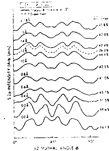
Fig. 48. As Fig. 47, but for c(2 \times 2) S in 4-fold coordination on Ni(001) and a broader range of z values; \beta = 1.0 for all curves. (From Connelly, ref. (33).)
