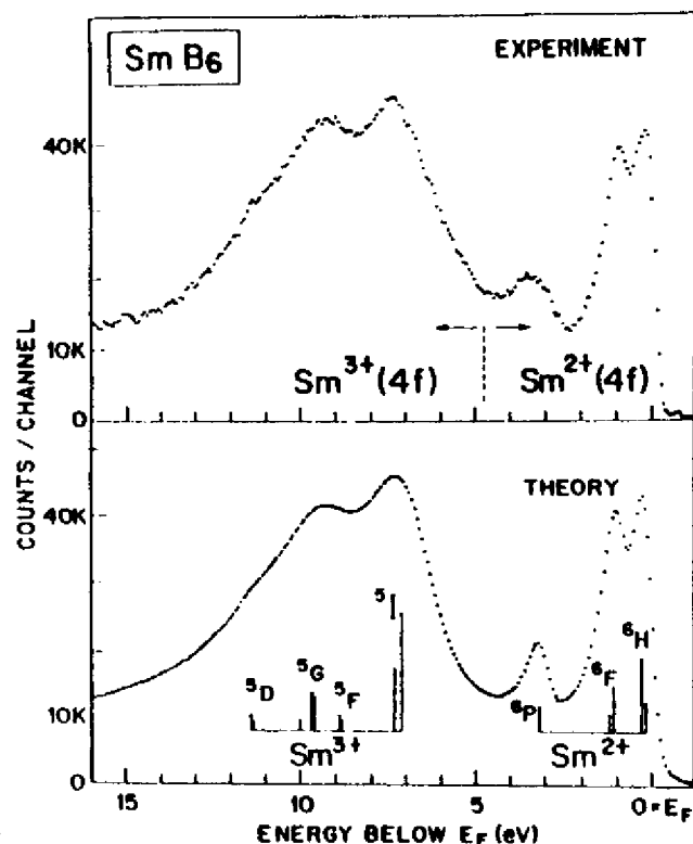
Fig. 35. Experimental and theoretical 4f valence spectra from SmB 6 , a "mixed-valence" metallic compound believed to contain both Sm 12 4f 6 and Sm 13 4f 5 . The intensities of the various final-state multiplets for Sm 12 → Sm 13 and Sm 13 → Sm 14 were computed using fractional parentage coefficients and are indicated as vertical bars. These calculations were broadened by an empirically-derived function of the form of Eq. (158) to generate the final theoretical curve. Monochromatized AlK \alpha was used for excitation. (From Chazalviel et al. , ref. 266.)
