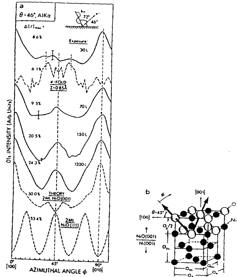
FIGURE 13. (a) O 1s azimuthal XPD data from oxygen on Ni (001) at four exposures from the c(2 \times 2) regime (30 L) to saturated oxide (1200 L). The kinetic energy is 945 eV. The polar angle of 45^\circ involves scanning very close to the \langle 110 \rangle directions at \theta = 45^\circ and \phi = 0^\circ and 90^\circ . Also shown are SSC-SW calculations for fourfold c(2 \times 2) oxygen at z = 0.85 \text{ \AA} and fully ordered 2 ML overlayers of NiO with both (001) and (111) orientations. (b) An approximate representation of the structure of the dominant Ni (001) formed at high exposures, indicating the oxide lattice expansion and strain involved. Also shown as arrows are the directions of the strong forward-scattering peaks observed at \phi = 0^\circ, 90^\circ in (a). (From Ref. 26)
