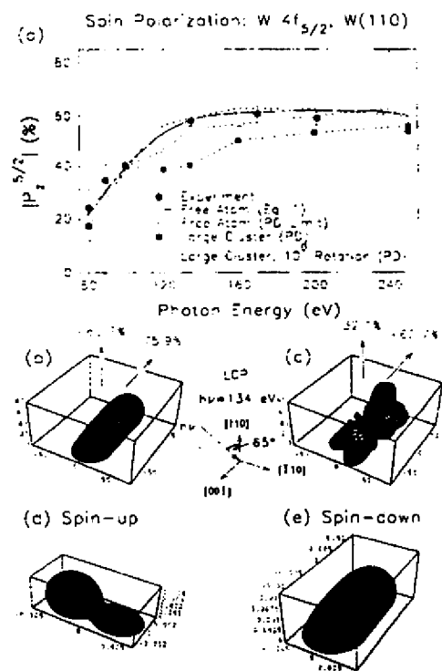
Fig. 20. Spin-polarization in W 4f spectra excited by circular-polarized light from W(110): (a) the absolute value of the 4f 5/2 polarization as a function of photon energy, with experiment compared to both free-atom and MS cluster PD calculations; (b) the three-dimensional spin polarization for a free atom in the experimental geometry shown in the inset and with an excitation energy of 134 eV; (c) as (b), but for a MS cluster PD calculation in a 5-atom cluster (an emitter below 4 surface scatterers); (d),(e) the separate spin-up and spin-down intensities excited in a free-atom. [From ref. 48.]
