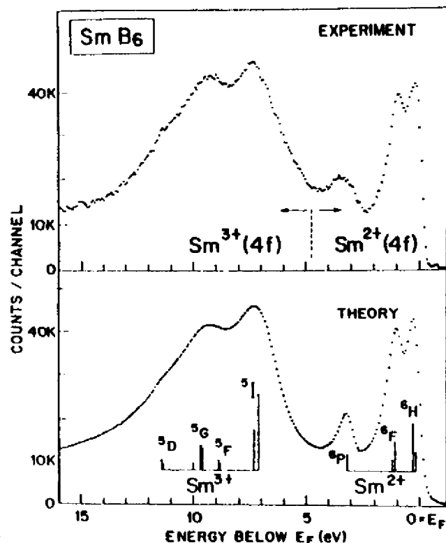
Fig. 35. Experimental and theoretical 4f valence spectra from \text{SmB}_6 , a "mixed-valence" metallic compound believed to contain both \text{Sm}^{1/2}4f^6 and \text{Sm}^{2/3}4f^5 . The intensities of the various final-state multiplets for \text{Sm}^{1/2} \rightarrow \text{Sm}^{3/2} and \text{Sm}^{2/3} \rightarrow \text{Sm}^{5/3} were computed using fractional parentage coefficients and are indicated as vertical bars. These calculations were broadened by an empirically-derived function of the form of Eq. (158) to generate the final theoretical curve. Monochromatized \text{AlK}\alpha was used for excitation. (From Chazalviel et al. , ref. 266.)
