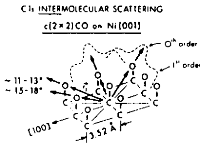
Fig. 41. Schematic illustration of the mechanism by which intermolecular scattering produces azimuthal anisotropy in C1s emission from c(2x2)CO on Ni(001). (From Orders and Fadley, ref. (81).)
