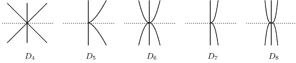
FIGURE 2.4. Real pictures of one-dimensional D_k -singularities
