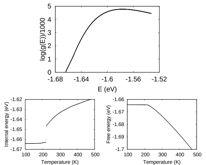
FIG. 9: Top panel: Calculated logarithm of the density of configuration states, g(E) , for Na on Al(100) at a coverage of 0.2 monolayers. Lower panels: Internal and free energy of this system as derived from g(E) (from Borg et al. , 2004).
