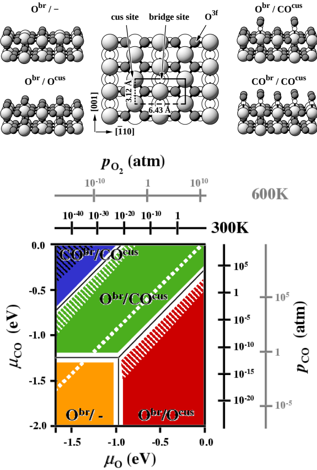
FIG. 5: Top panel: Top view of the RuO 2 (110) oxide surface explaining the location of the two prominent adsorption sites (coordinatively unsaturated, cus, and bridge, br). Also shown are side views of the four stable phases present in the phase diagram shown below (Ru = light large spheres, O = dark medium spheres, C = white small spheres). Bottom panel: Surface phase diagram for RuO 2 (110) in “constrained equilibrium” with an oxygen and CO environment. Depending on the gas-phase chemical potentials ( \mu_{\text{O}} , \mu_{\text{CO}} ), br and cus sites are either occupied by O or CO, or empty (-), yielding a total of four different surface phases. For T = 300 K and T = 600 K, this dependence is also given in the corresponding pressure scales. Regions that are expected to be particularly strongly affected by phase coexistence or kinetics are marked by white hatching (see text). Note that conditions representative for technological CO oxidation catalysis (ambient pressures, 300-600 K) fall exactly into one of these ranges (from Reuter and Scheffler, 2003a,b).
