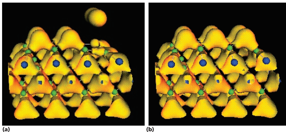
Figure 2. DFT electronic-structure calculation for the adsorption of an \text{As}_2 molecule on the GaAs(001) surface. In (a), the \text{As}_2 molecule hovers above the surface (yellow balls in the upper part of the picture). In (b), the molecule has adsorbed onto the surface and established chemical bonds with the surface Ga atoms. The closed yellow surfaces represent contours of constant electron density. The blue dots represent the As nuclei; the green dots, the Ga atoms.
