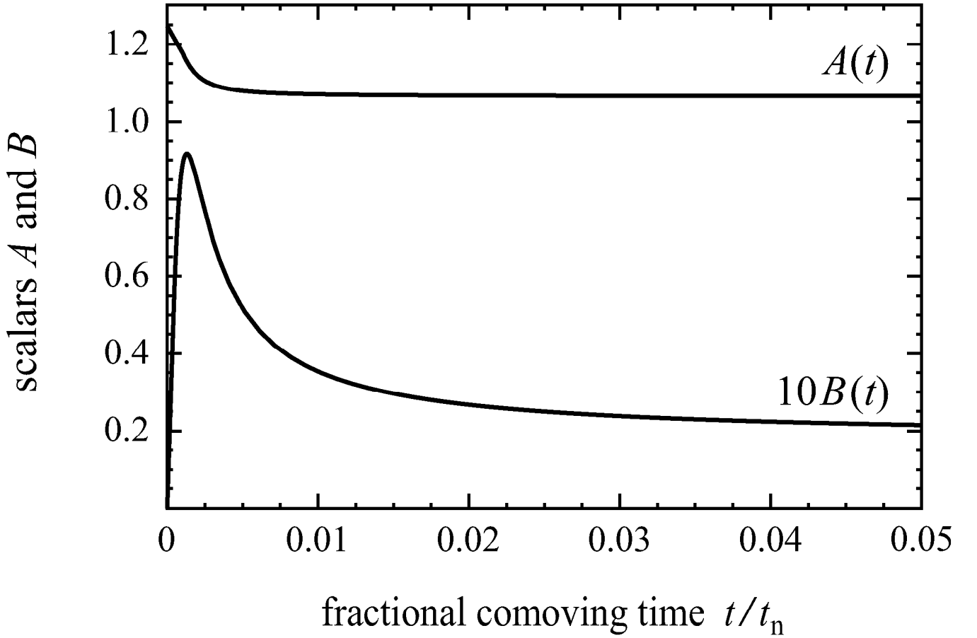
Figure 3: Time evolution of the scalars A(t) and B(t) at early cosmological times. In the recent past of our model universe, which is not shown here, A(t) and B(t) are essentially constant.
