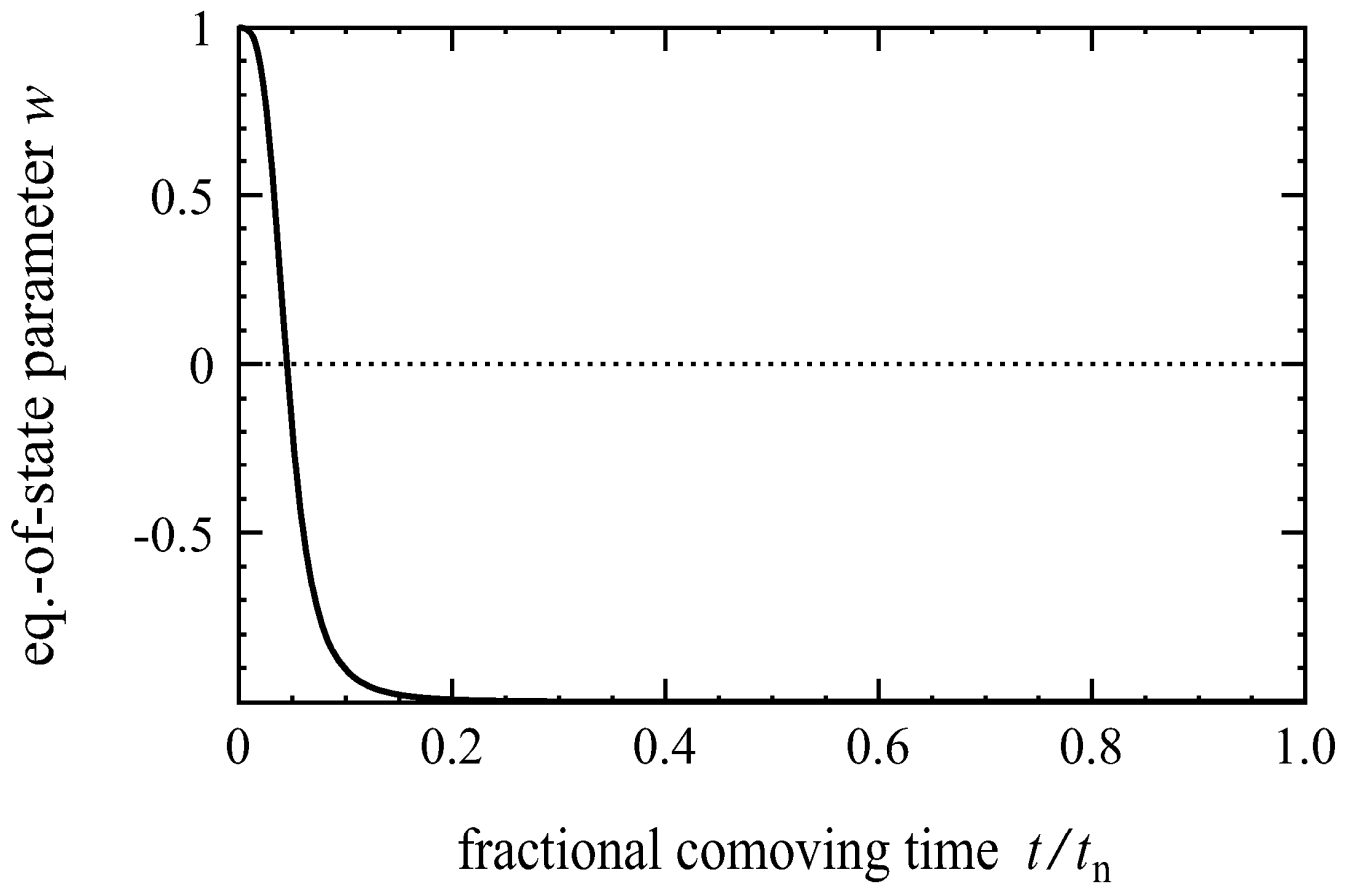
Figure 4: Time evolution of the equation-of state parameter w . At late times, w \rightarrow -1 , so that the scalars essentially obey the cosmological-constant equation of state.
