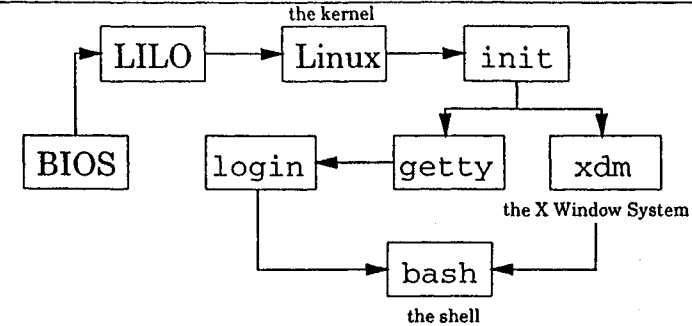
Figure 3.1 The path an Intel PC takes to get to a shell prompt. init may or may not start the X Window System. If it does, xdm runs. Otherwise, getty runs.
