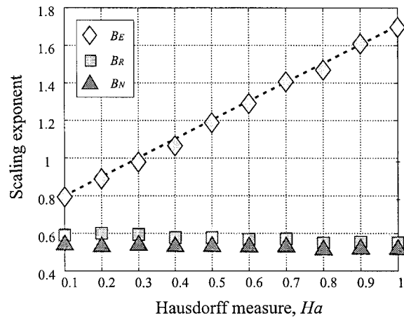
Figure 13: Dependence of scaling exponents B_{E,R,N} (Eq. (10)) on the Hausdorff measure Ha of FBWs. Dashed line is B = 0.7 + Ha .
