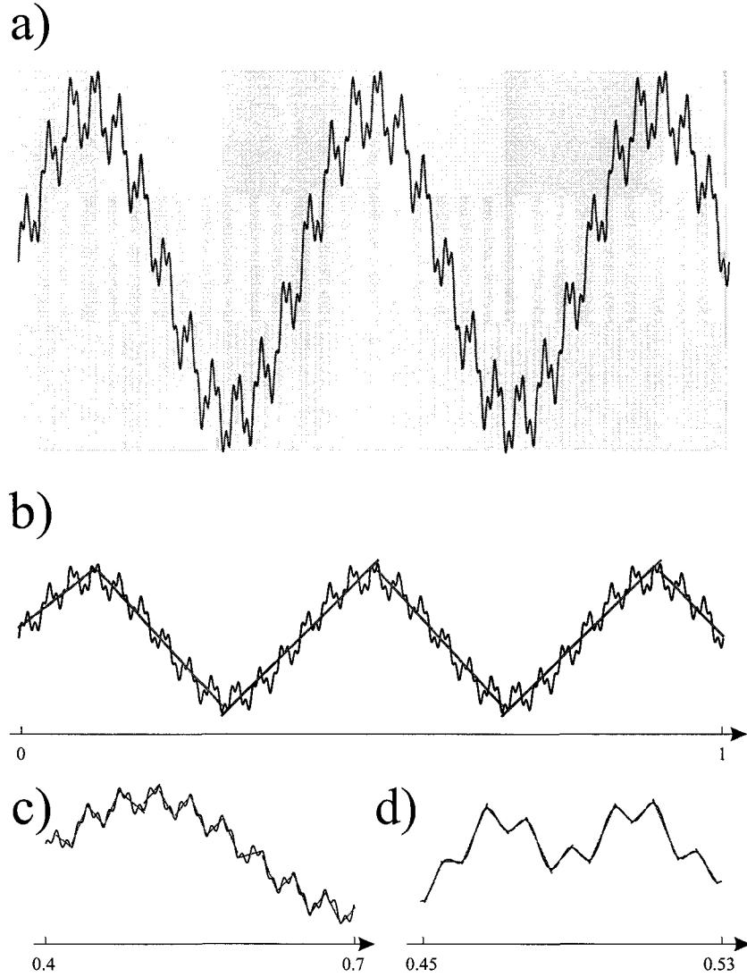
Figure 4: Decomposition of the sum of three sinusoids, X(t) = \sin(5\pi t) + \frac{1}{5}\sin(60\pi t) + \frac{1}{10}\sin(200\pi t) . a) X(t) on the background of three levels from its decomposition. b) Piecewise linear approximation corresponding to the top level of the decomposition shown in panel a). c) Fragment corresponding to the middle level of a). d) Fragment corresponding to the bottom level of a).
