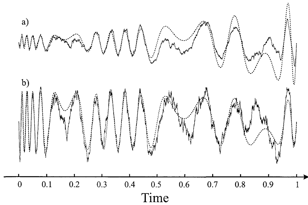
Figure 19: Reconstruction (solid lines) of the coupling parts A_i(t) \cdot X(t) (dashed lines).
