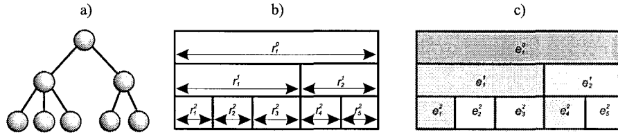
Figure 12: Three levels of detail in MTA description of a time series. a) Topological. b) r-metric, based on the interval partition. c) e-metric, based on local linear fit of the series. See details in Sect. 4.
