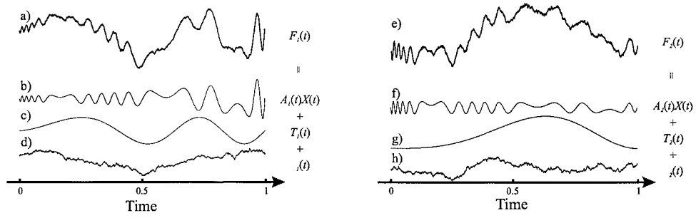
Figure 18: Structure of the signals F_i(t) , i = 1, 2 shown in Fig. 15. a),e) Original signals F_i(t) . b),f) Coupling parts A_i(t) \cdot X(t) . c),g) Non-linear deterministic trends. d),h) Random drifts.
