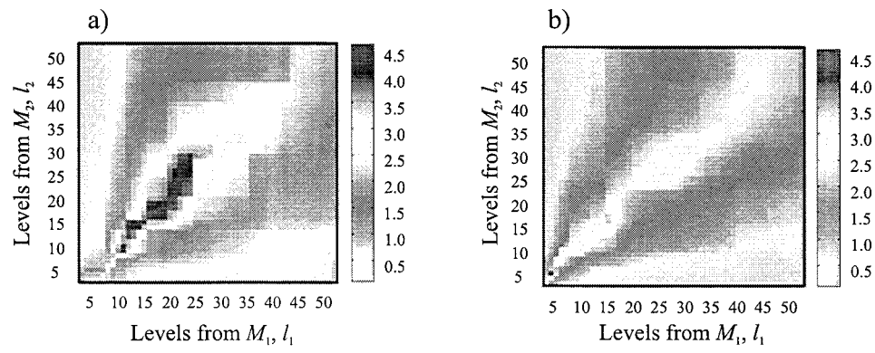
Figure 16: Correlation (reciprocal distance) \mu (17) between two signals shown in Fig. 15 (panel a) and two independent Brownian walks (panel b).
