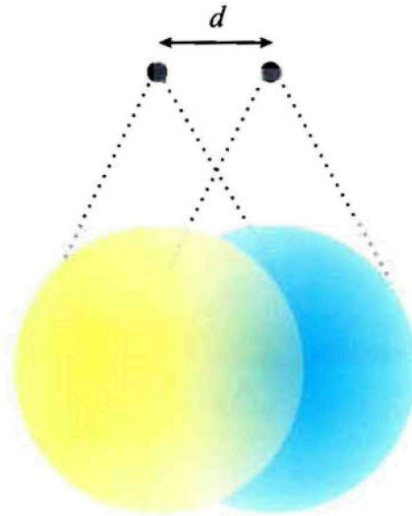
Fig. 3. – A schematic representation of the fluorescence spots from two single molecules with a separation d .
