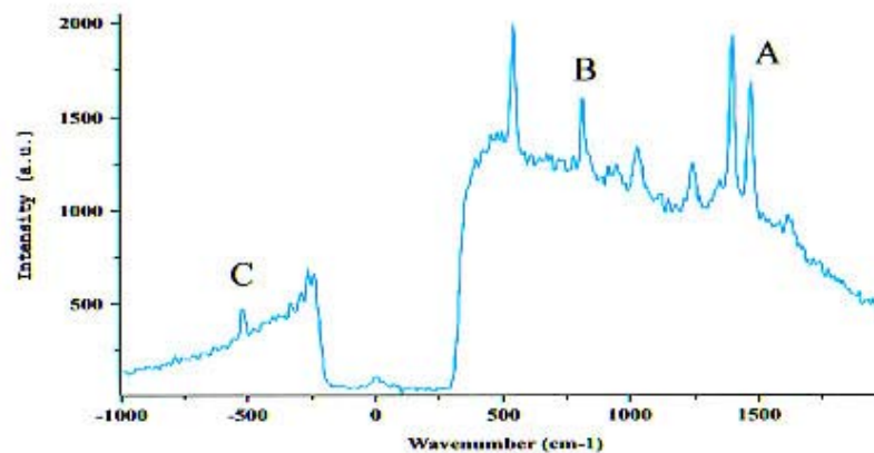
Near-field Phthalazine Raman spectrum
