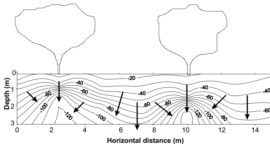
Figure 17 – Isolines of total soil water potential head beneath two rubber trees and water flow directions.
