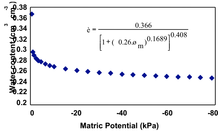
Figure 13 – Average soil water retention curve measured in field soils of several countries (IAEA, 1984)
