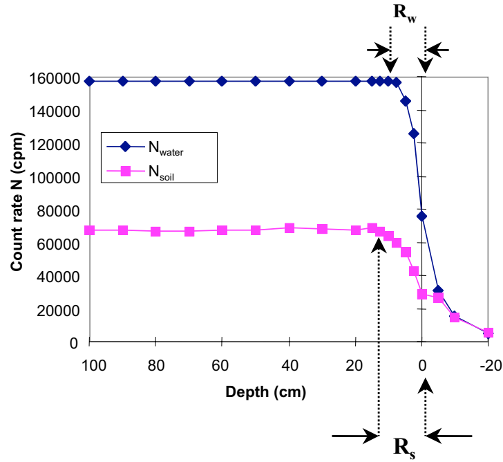
Figure 4 – Spheres of influence in soil and water.
