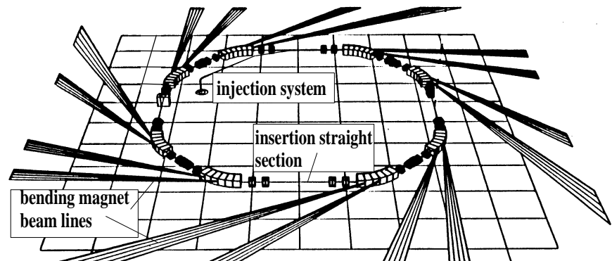
Figure 1: Schematic layout of a synchrotron light source
