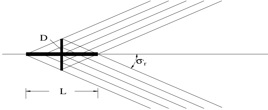
Figure 22: Apparent photon beam source size
