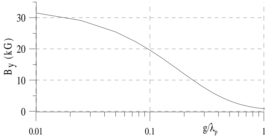
Figure 18: On axis field strength in a Vanadium Permendur hybrid wiggler magnet as a function of gap-aperture
