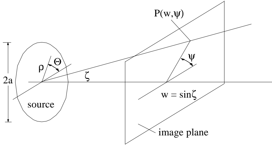
Figure 20: Diffraction geometry
