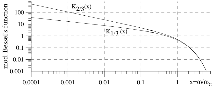
Figure 5: Functions K_{1/3}(\xi) and K_{2/3}(\xi)
