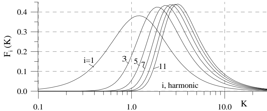
Figure 16: Function f_i(K) = \frac{i^2 K^2 [JJ]}{(1+\frac{1}{2}K^2)^2}
