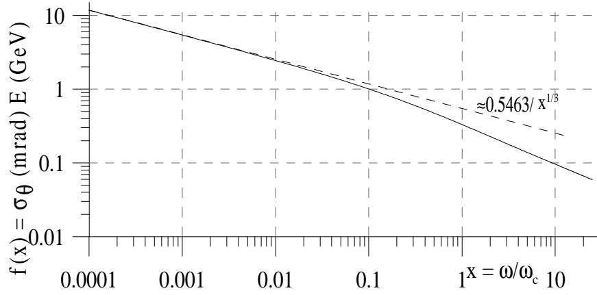
Figure 7: Vertical opening angle: f(x) = \sigma_\theta E
