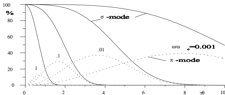
Figure 10: Relative magnitude of \sigma - (solid) and \pi -mode (dash) radiation
