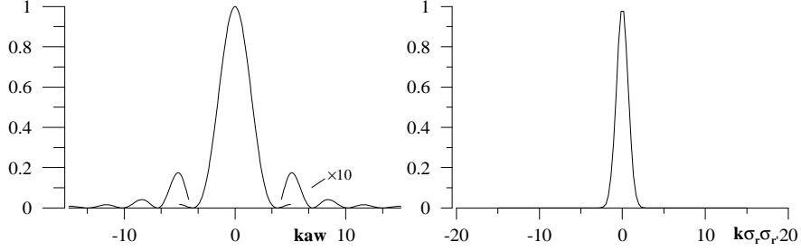
Figure 21: Fraunhofer diffraction for a circular light source illuminated uniformly (left) and with a gaussian illumination (right)
