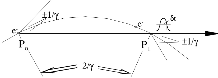
Figure 4: Time structure of synchrotron radiation
