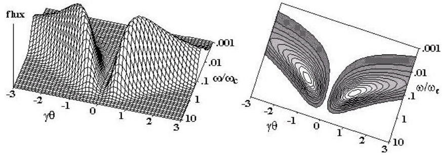
Figure 8: Spatial and spectral distribution for \sigma -mode radiation
