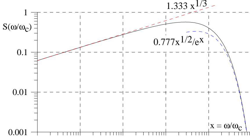
Figure 6: Universal function
