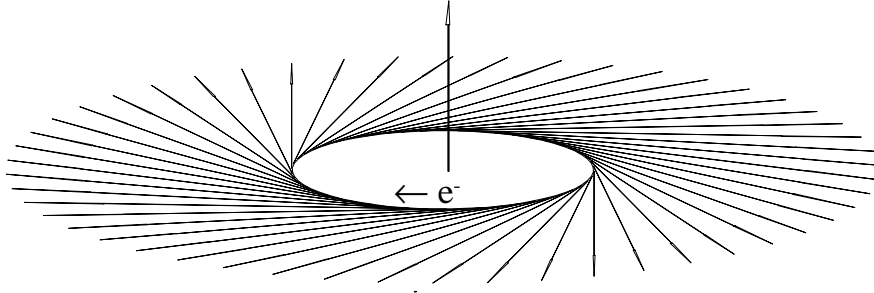
Figure 3: Synchrotron radiation swath
