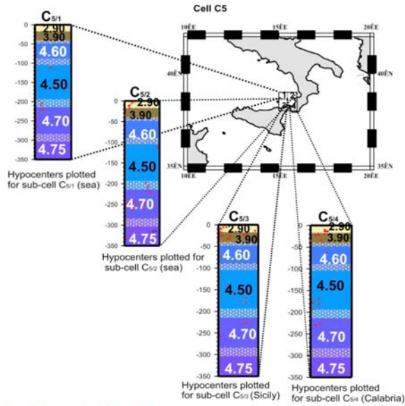
Hypocenters of the earthquakes with M_s \geq 2.0 rewied by ISC
