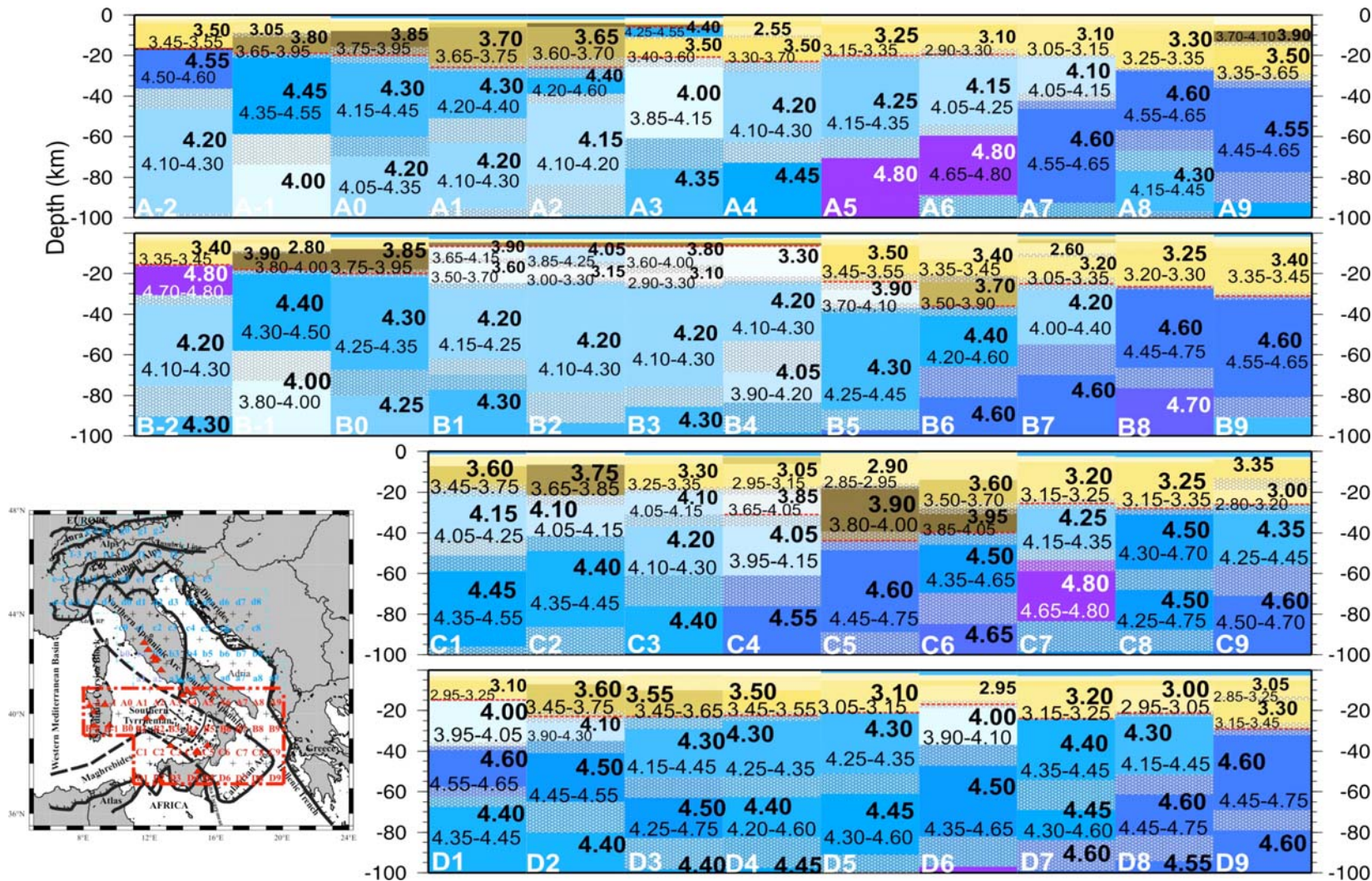
Fig. II f: Structural models of the chosen solution, indicated by red line in Fig. 3.13a. For each cell of the study area, indicated by the red dashed line in the insert, the velocity value and its range of variability is specified for the crust and upper mantle layers down to 100 km. The thickness range of variability is marked by the shadowed area.
