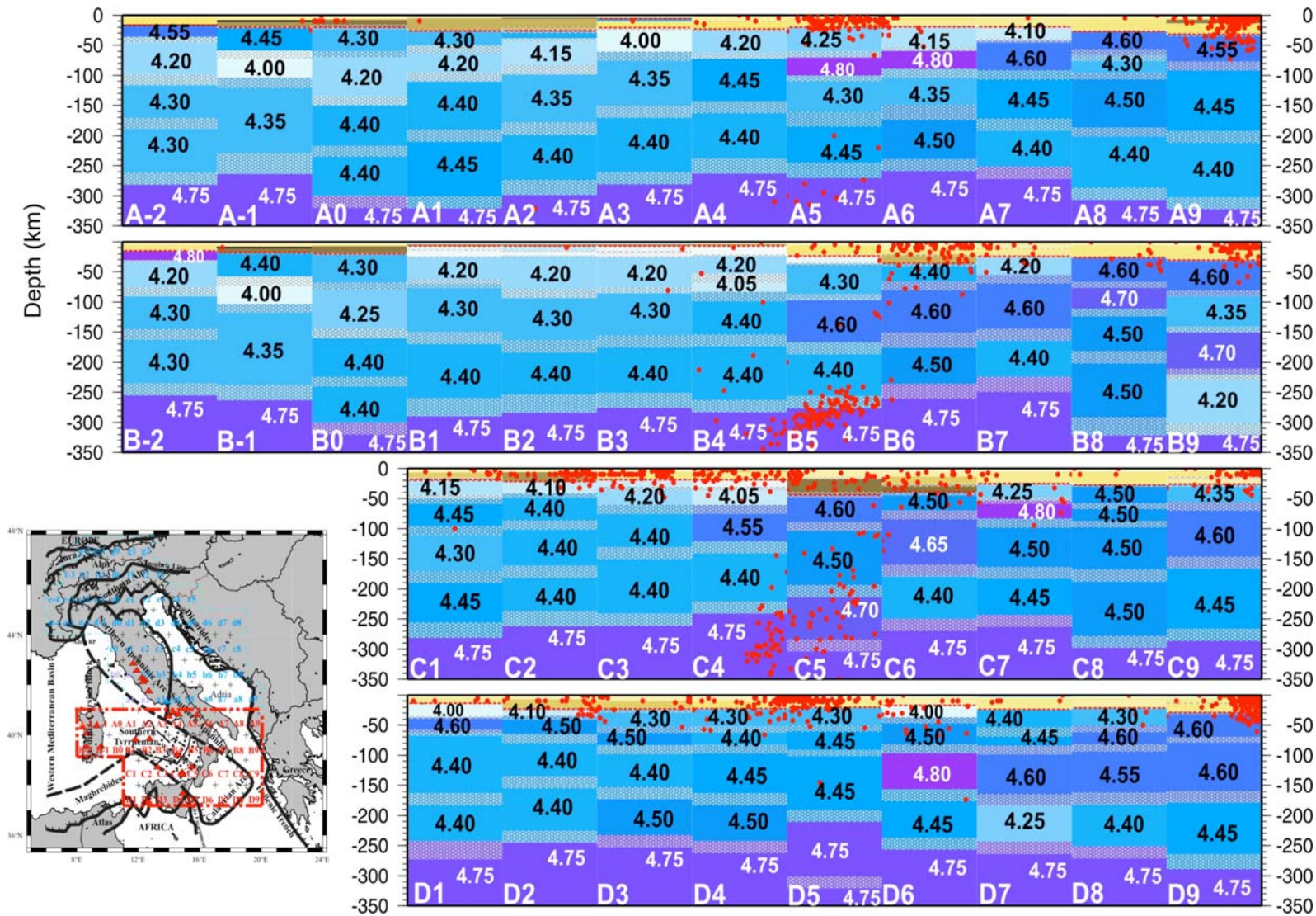
Fig. 11.14 e: Structural models, chosen by LSO, for each cell of the area marked with a red line in the insert. The models are represented in the depth range 0-350 km and the range of variability of the inverted layers' thickness is shown as shadowed area; in each cell the Moho is marked by a red dashed line. The distribution of hypocentres of the events with magnitude greater than 3, collected from ISC on-line bulletin for the period 1904-2004, is shown for each cell.
