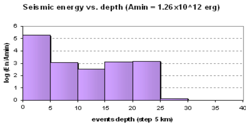
Fig. 13.4: Seismic energy distribution in cell a2, represented as \log(E_n/A_{min}) vs. depth: A_{min}(\text{erg})=1.26 \times 10^{12} erg is the min energy, registered in the depth interval 30-35 km.
