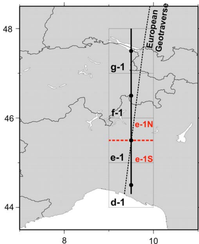
Fig. 13.7: Plot of the studied profile (solid line) through the Central Alps, the Po Plain and the Ligurian Apennines. Each dot corresponds to the centre of the 1^\circ \times 1^\circ cell. A part of the European Geotraverse (dashed line) is also shown.
