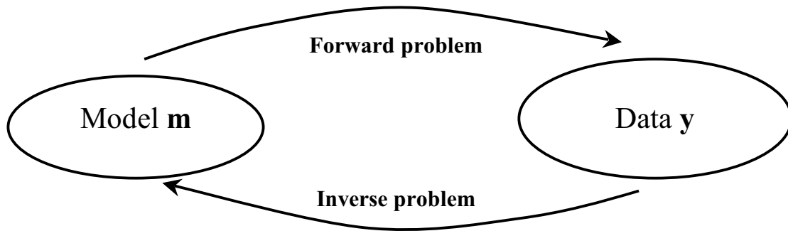
Fig. 1.1: Forward and inverse problem
