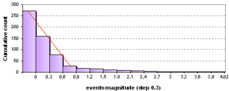
Fig. 13.3: Cumulative count of seismic events collected in cell a2 by the ISC online bulletin (1904-2004) and grouped every 0.3 M_s interval.
