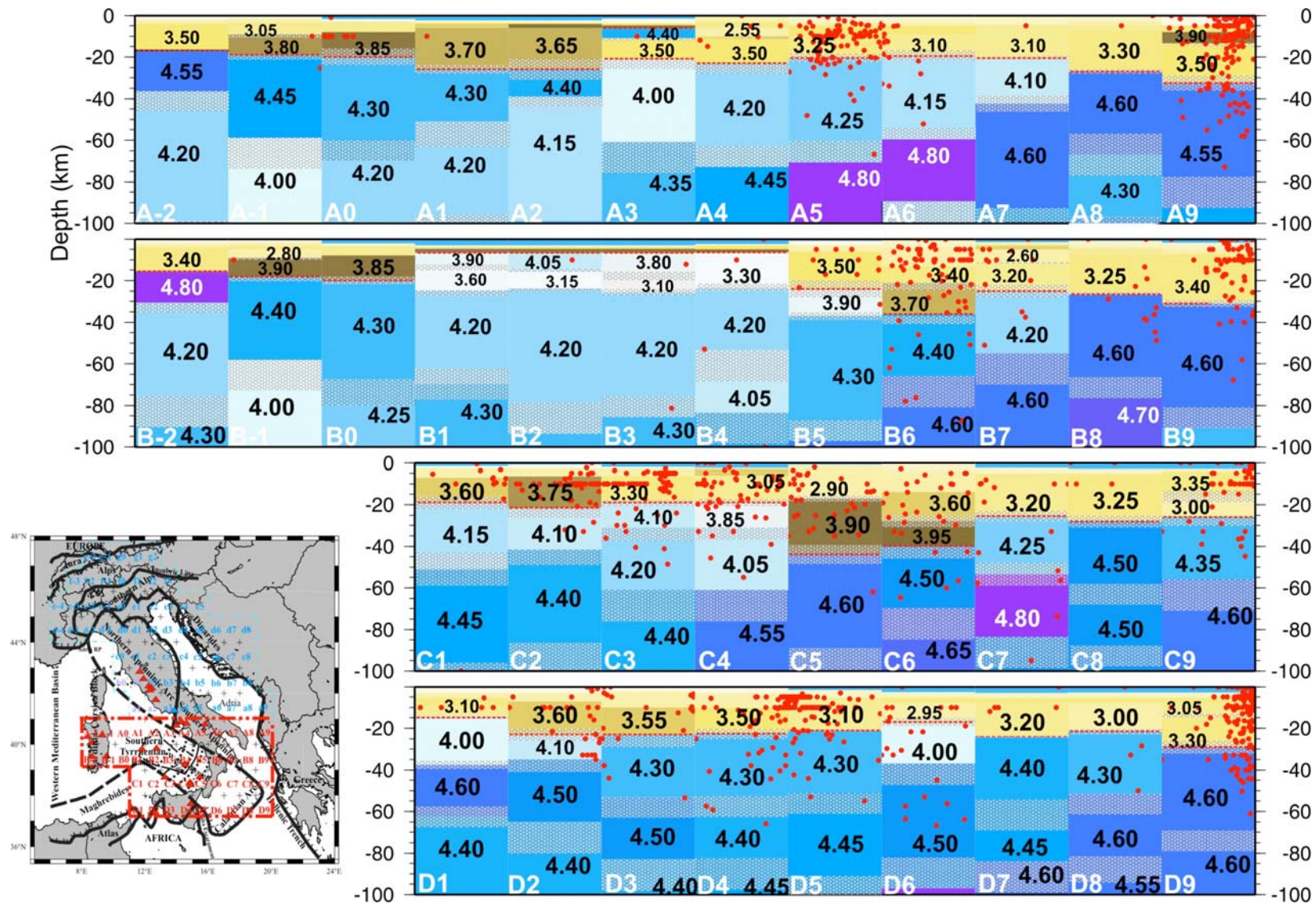
Fig. 11.14 f: Zoom of Fig. 11.14 e in the depth range 0-100 km.
