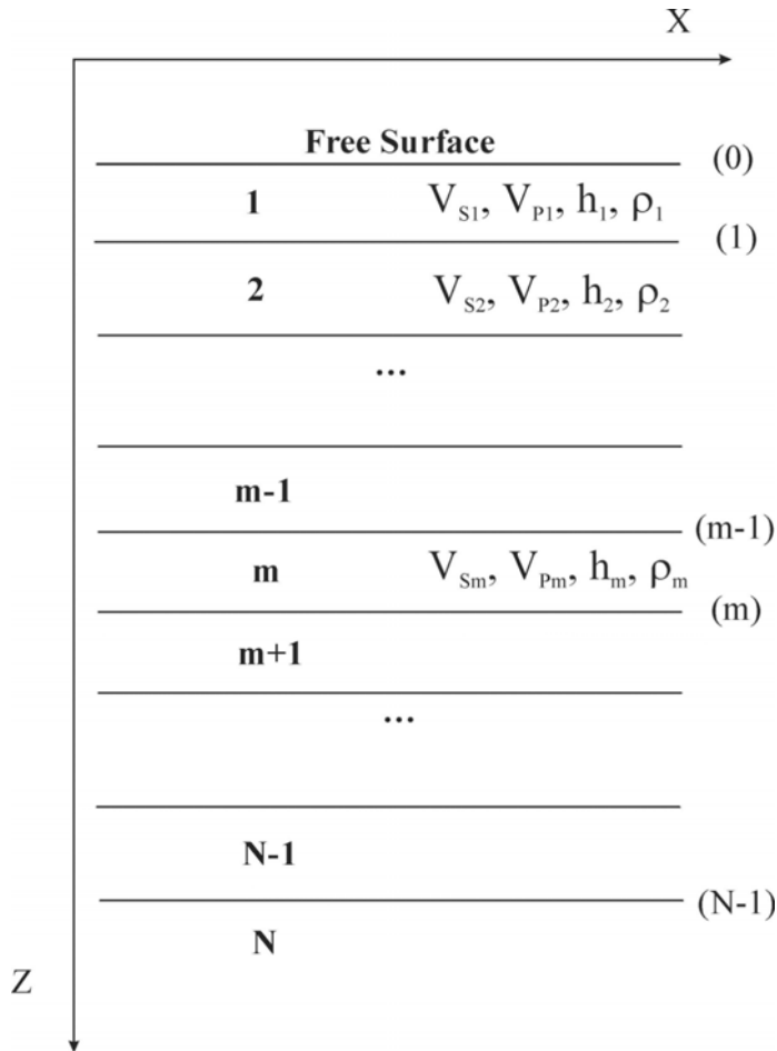
Fig. 3.1: Structural model is modeled as a stack of N homogeneous isotropic layers, each one defined by compressional ( V_p ) and shear ( V_s ) wave velocities, thickness ( h ) and density ( \rho ). Boundaries between two layers are indicated with (m).
