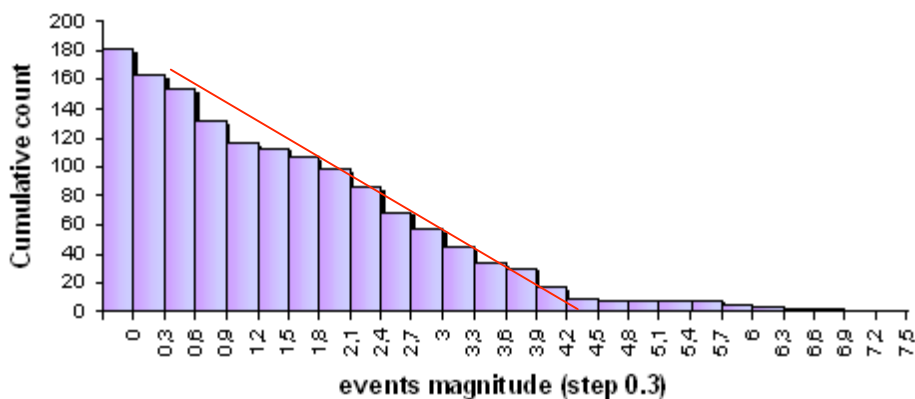
Fig. 13.5: Cumulative count of seismic events collected in cell C5 by the ISC online bulletin (1904-2004) and grouped every 0.3 M_s interval.
