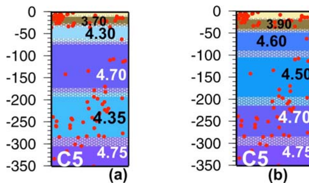
Fig 11. 10: Hypocenter distribution versus depth for the earthquakes falling in cell C5. (a) Seismic velocities (km/s) are given for the LSO solution; (b) seismic velocities (km/s) are given for the solution more consistent with seismicity distribution.
