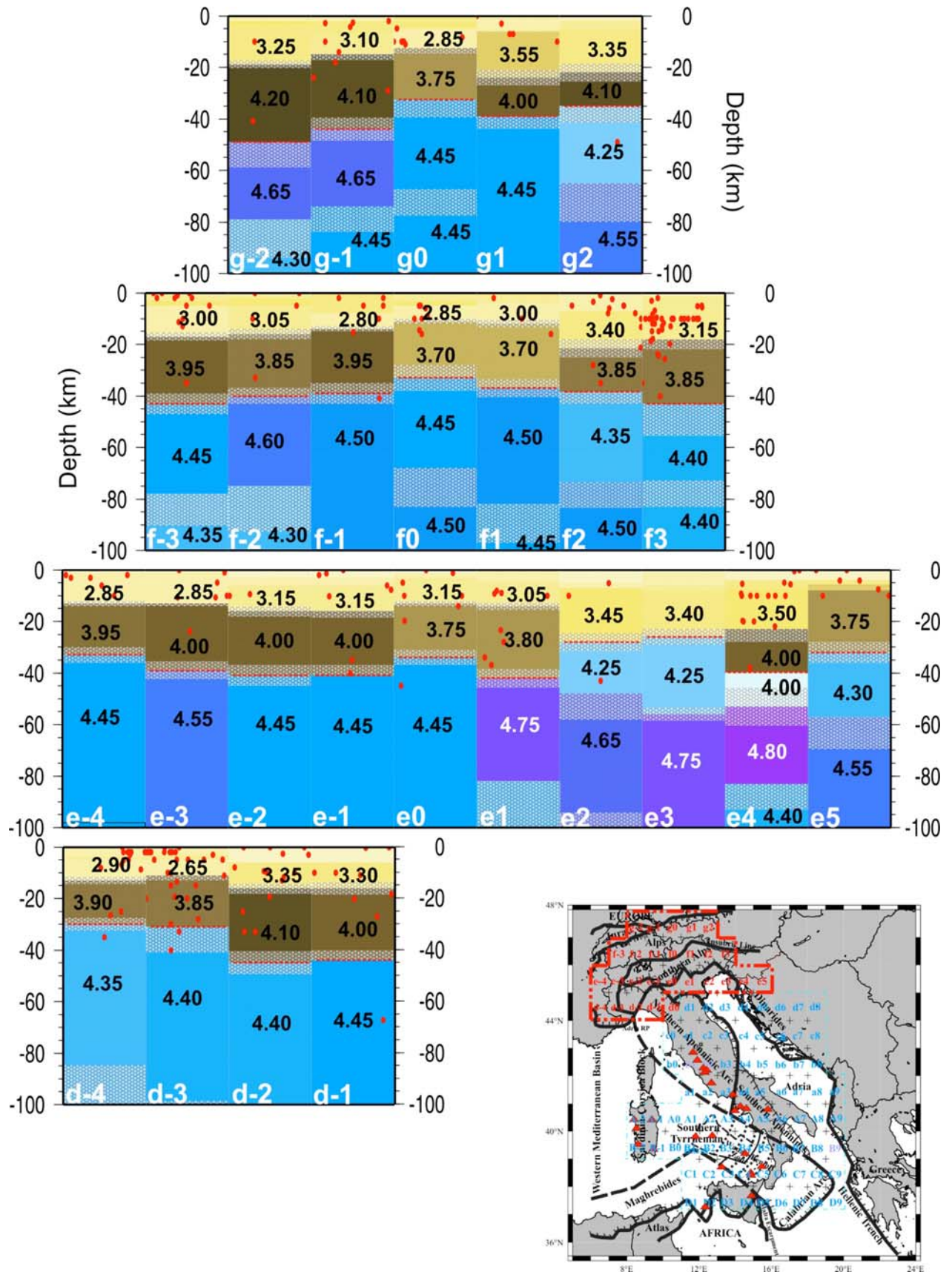
Fig. 11.14 b: Zoom of Fig. 11.14 a in the depth range 0-100 km.
