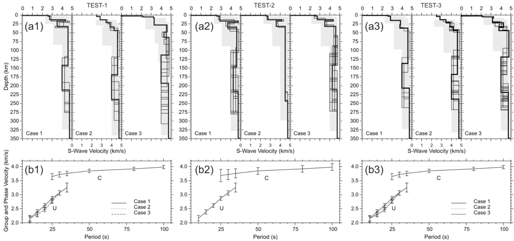
Fig. 4.1: Results of tests 1, 2 and 3. (a1, a2, a3) Sets of solutions (thin lines) obtained through the non-linear inversion of the dispersion relations shown in (b1, b2, b3). The investigated parameter's spaces (grey zones) and the chosen solutions (bold lines) are shown as well. The parameterization used in the inversion is given in Tab. 4. (b1, b2, b3) Group (U) and phase (C) velocity curves used in the tests (see Tab. 3).
