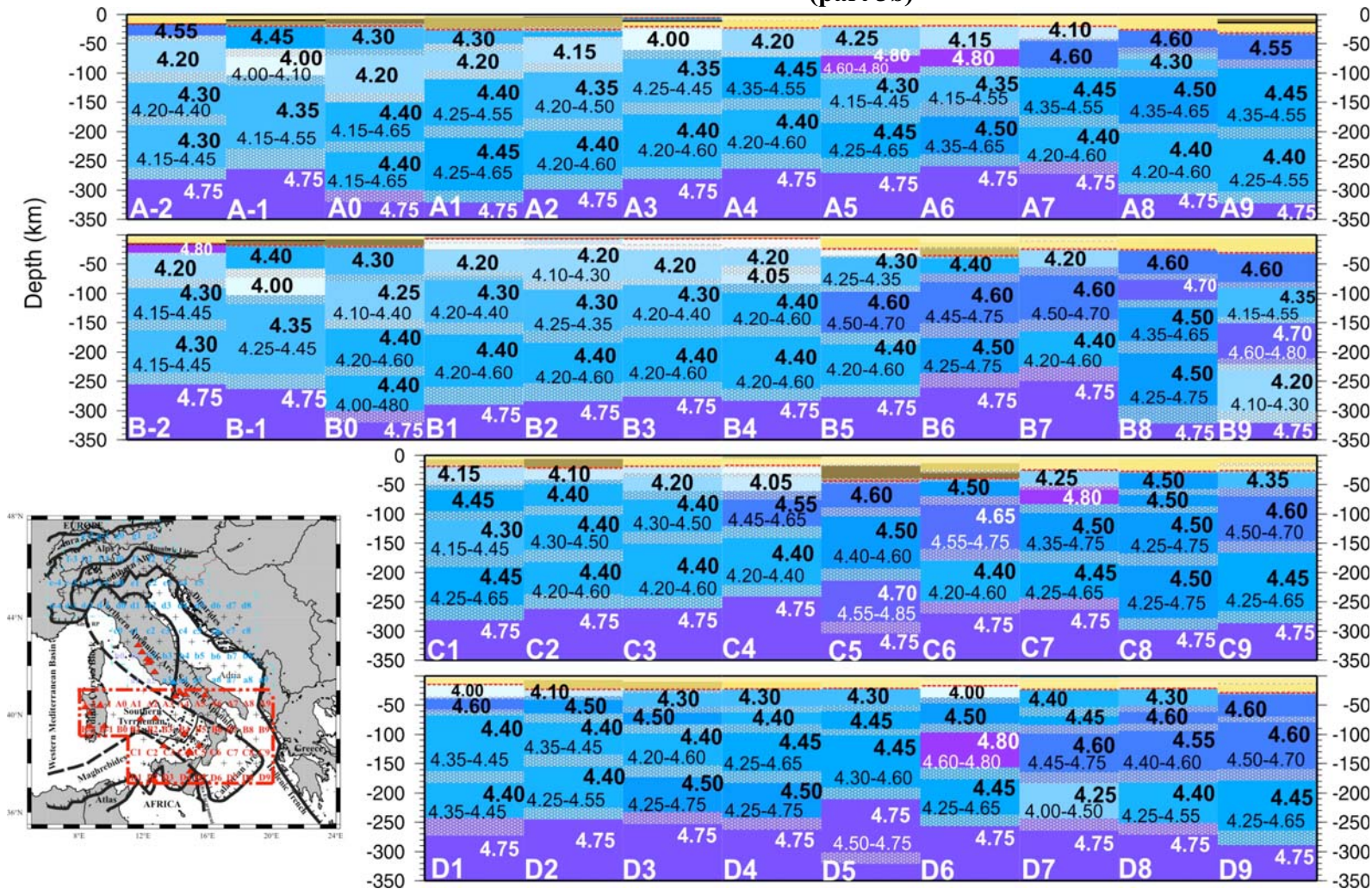
Fig. II e: Structural models of the chosen solution, indicated by red line in Fig. 3.13a. For each cell of the study area, indicated by the red dashed line in the insert, the velocity value and its range of variability is specified for the mantle layers down to the investigated 350 km. The thickness range of variability is marked by the shadowed area.
