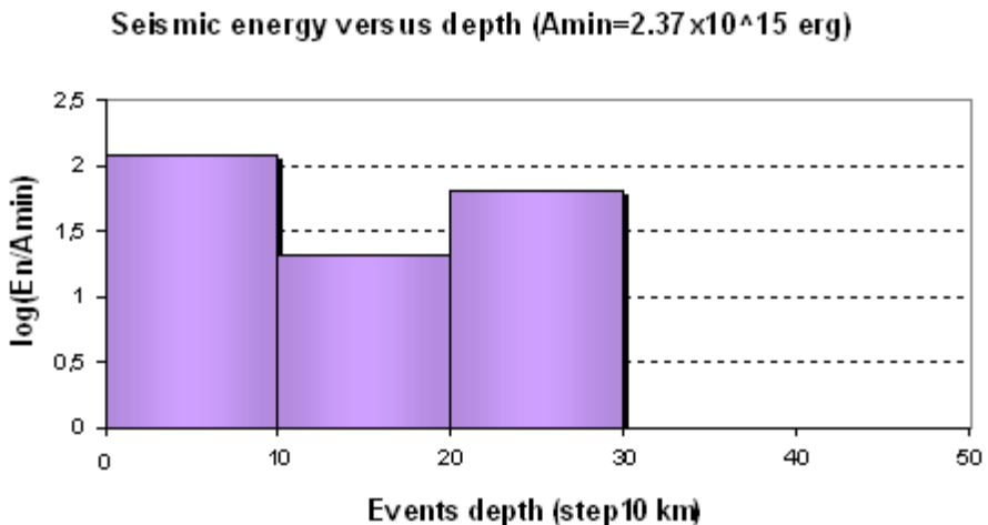
Fig. 13.2: Seismic energy distribution in cell e4, represented as \log(E_n/A_{\min}) vs. depth: A_{\min}(\text{erg})=2.37 \times 10^{15} erg is the minim energy, registered in the depth interval 30-40 km.
