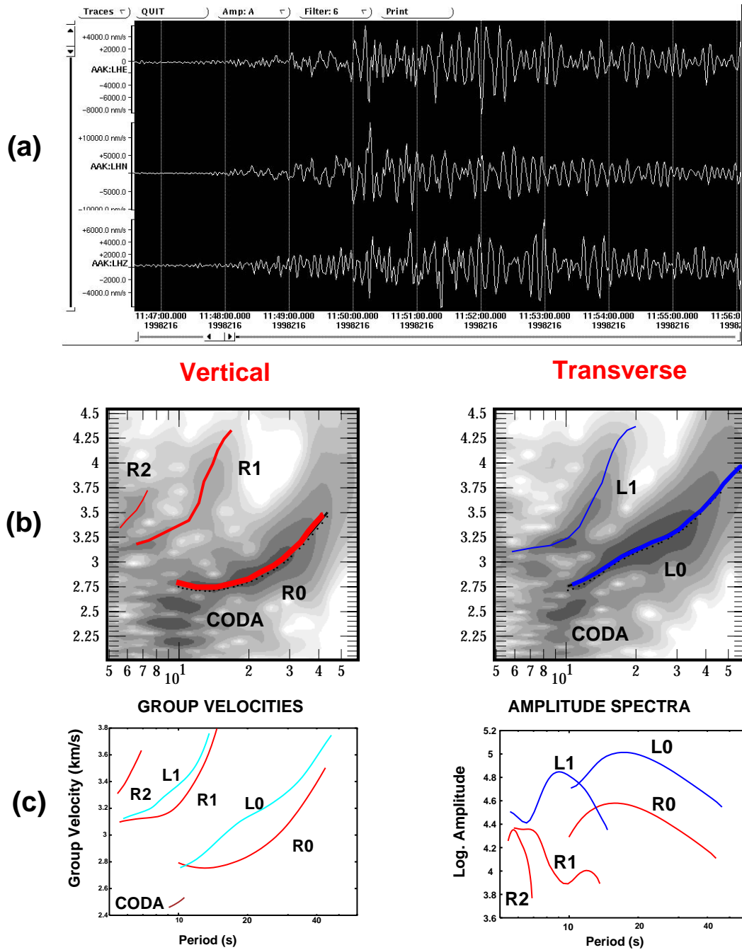
Figure 8. The earthquake at Iran-Turkmenistan border recorded at AAK (epicentral distance 1560 km): (a) records; (b) FTAN diagrams; (c) group velocities and amplitude spectra. Strong higher modes and fundamental modes of Rayleigh and Love waves are present.
