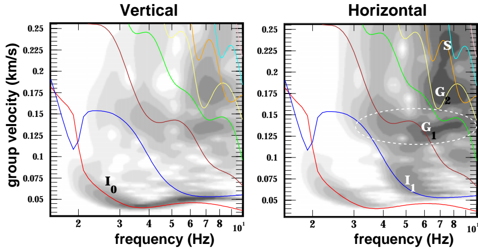
Figure 5. FTAN diagrams for two sea-bottom records.
