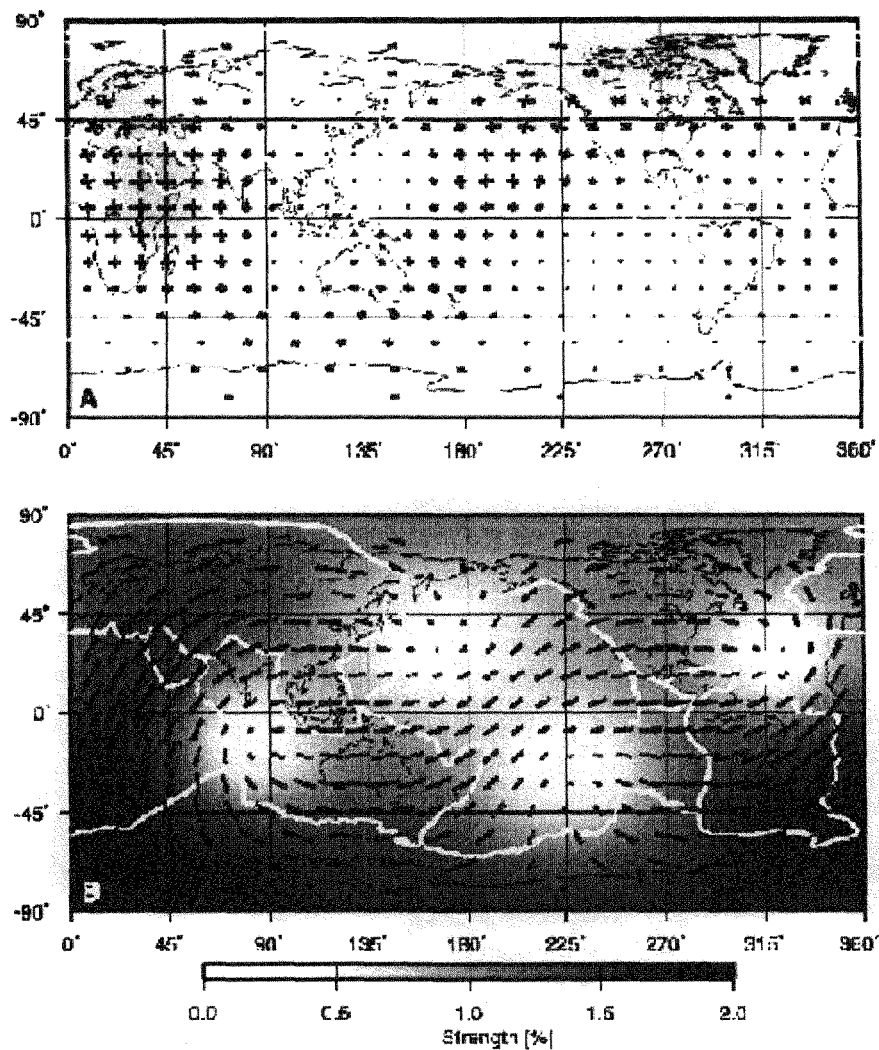
Figure 11: Transition zone Heterogeneities
