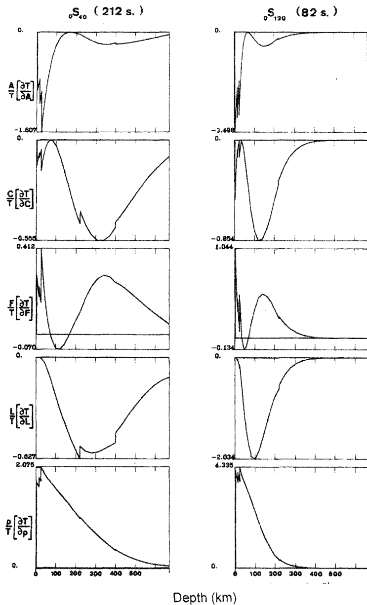
Figure A3 : kernels for Rayleigh waves. Same conventinos as for figure A1 in the same depth range. The partial derivative with respect to N has not been plotted since its amplitude is very small for fundamental modes. Note that 3 partials contribute to the 2Y -azimuthal terms , A-partial for B_c, B_s , F-partial for H_c, H_s and the largest one L-partial for G_c, G_s .
