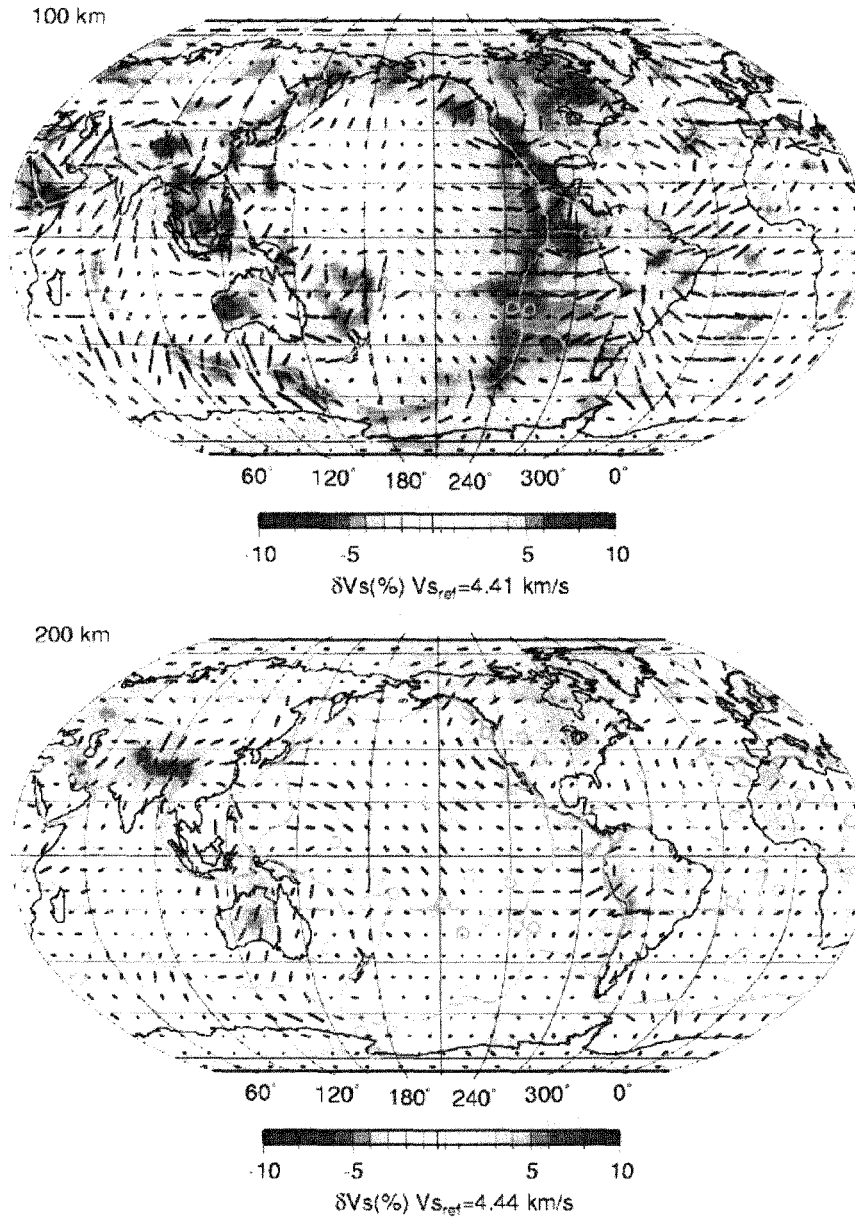
Figure 5 : 2 cross-sections at 100km (top) and 200km (bottom) depths of the global tomographic model of Debayle et al. (2005). Directions of azimuthal anisotropy are superimposed on S-wave velocity heterogeneities. The length of bars is proportional to its amplitude (<2%)
