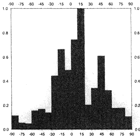
Figure 8 : Histogram of the difference between plate velocities directions and synthetic SKS anisotropy azimuths in the Pacific plate (After Montagner, 2002). It is calculated by summing the contributions of each grid point ( 5^{\circ} \times 5^{\circ} ) weighted by the latitude and the amplitude of anisotropy.
