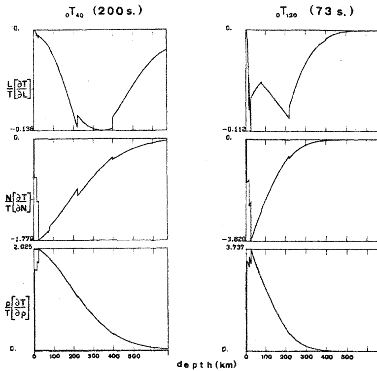
Figure A2 : Partial derivatives for Love waves of the period of fundamental normal modes 0T40 (left) and 0T120 (right) with respect to the elastic coefficients of a transversely isotropic earth L, N and density \rho , as a function of depth in the upper mantle (from Montagner and nataf, 1986). The partial derivatives with respect to A, C, F are null for these modes. The plots are normalized to their maximum amplitudes, given for a \Delta h=1000\text{km} thick perturbed layer. The combinations of elastic coefficients that have the same partial derivative as L are -G_c , -G_s for the azimuthal terms 2\Psi , and as N are E_c , E_s for the azimuthal term 4\Psi . Note that the amplitude of the L-partial is very small for the fundamental modes, which is not the case for higher modes.
