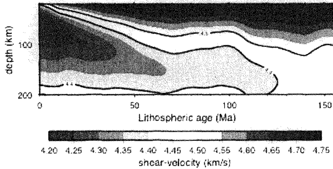
Fig. 9a Average shear velocity structure (After Ritzwoller et al., 2004)
