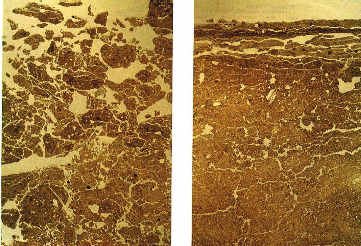
Fig. 3 – Macrophotographs of vertically oriented thin sections from the surface layer (0-5 cm) of the uncompacted (left) and compacted areas (right) of a loam soil. Plain polarized light. Pores appear white. The change of the subangular blocky structure of the uncompacted areas into a massive platy structure of the compacted areas is very evident. Frame length 3 cm.
