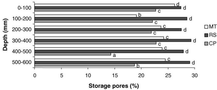
Fig. 1. Effects of tillage systems on storage pores inside the aggregates measured by mercury intrusion porosimetry along the soil profile (MT, minimum tillage; RS, ripper subsoiling; CP, conventional deep ploughing). Values differ significantly when followed by different letters at P \leq 0.05 employing the Duncan's multiple range test.
