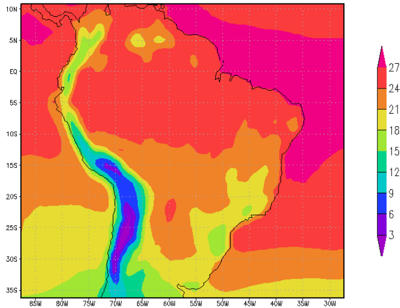
Temperature MAM 2008 ensemble mean
