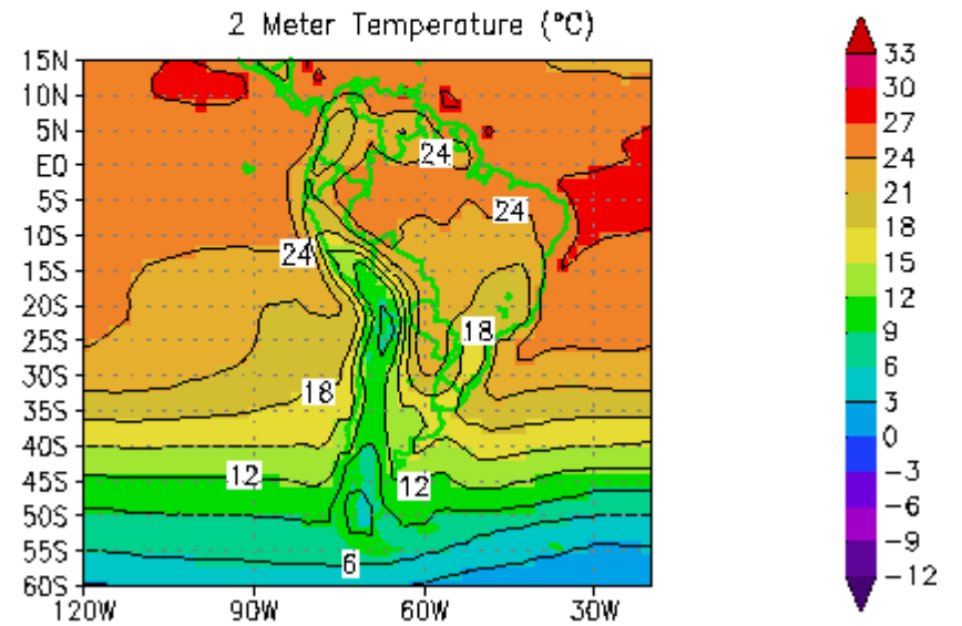
MAR-APR-MAY 2008 ECPC 2MT Ensemble Mean Trop. Ocean SSTa forecast (IRI Multi-Model Scenarios) from Jan 2008
