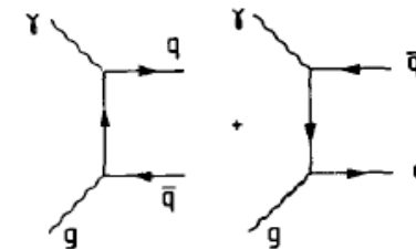
Fig. 1. Diagrams contributing to a finite mixing of order \alpha_s between g^p and the polarized gluon parton density.
