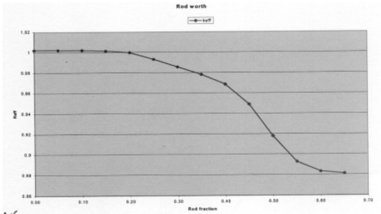
FIG. 4.25. Reactivity of the reactor as function of the control rod bank insertion for the critical core (core level at: 125.3 cm).
