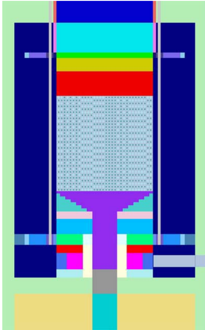
FIG. 4.38. Vertical cross section of HTR-10 reactor in SCALE4.4 model
