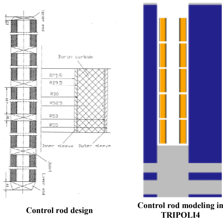
FIG. 4.44. Control Rods modeling in Monte-Carlo code TRIPOLI4.
