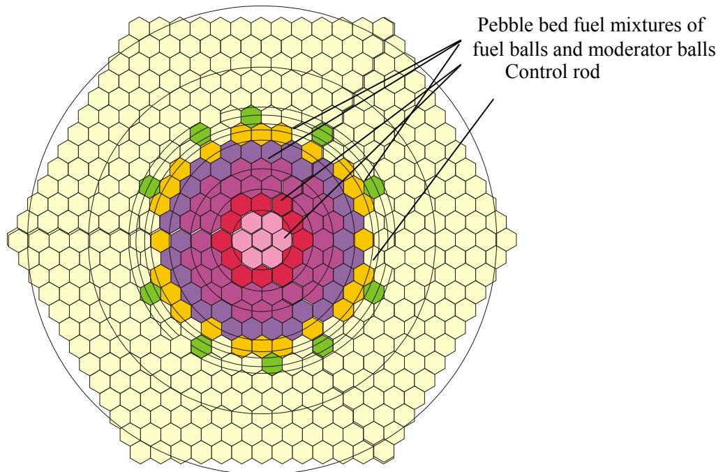
FIG. 4.20. HTR-10 Core Diffusion Calculation Model in R-Z geometry.
