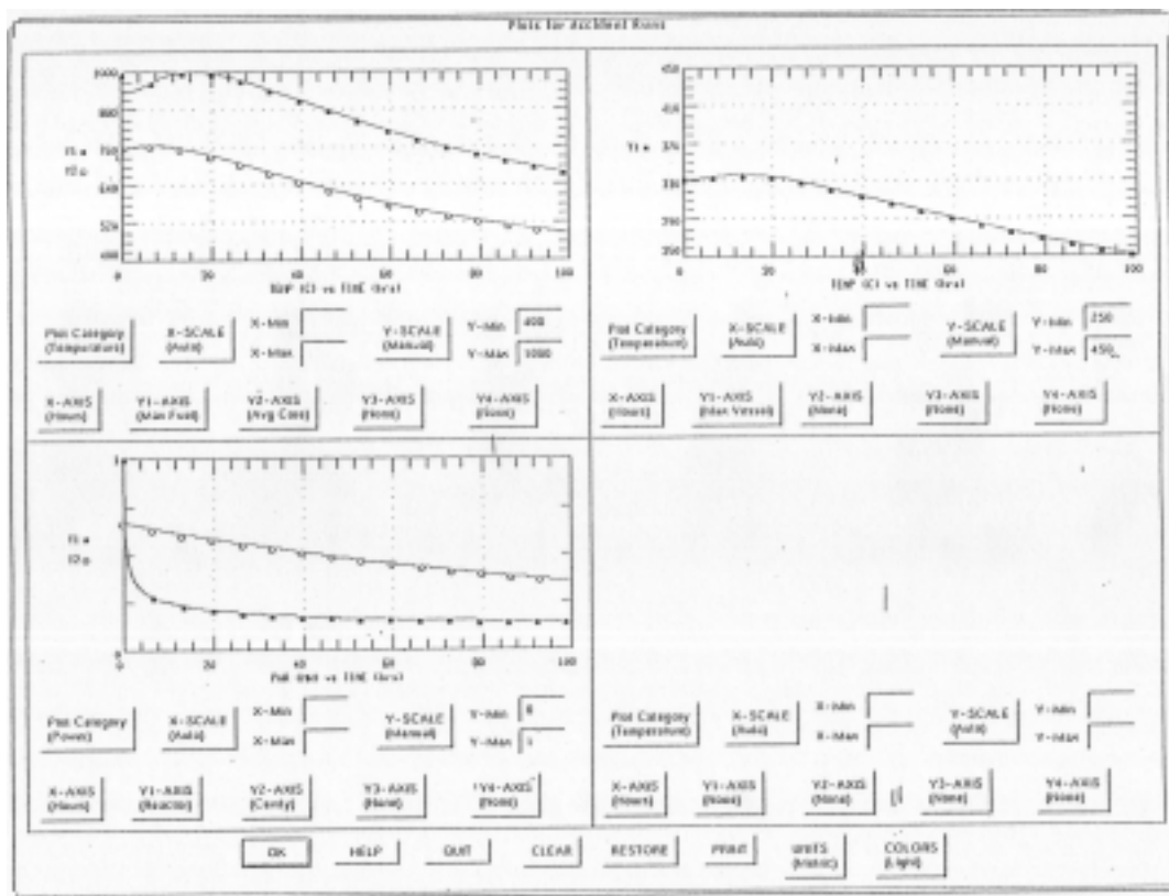
FIG. 3.55. HTTR LOSP with no auxiliary cooling flow (pressurized).
