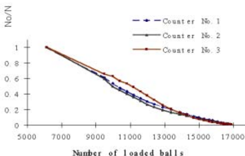
FIG 4.12. Extrapolation curve of the initial criticality approach
