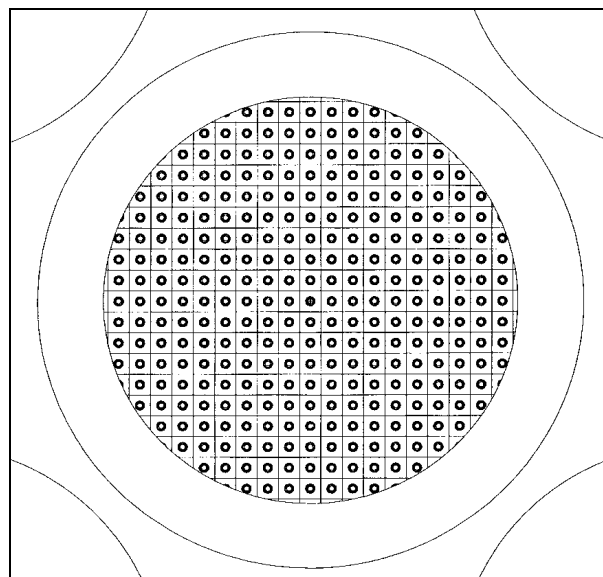
FIG. 4.35. MCNP Model of Fuel Pebble.
