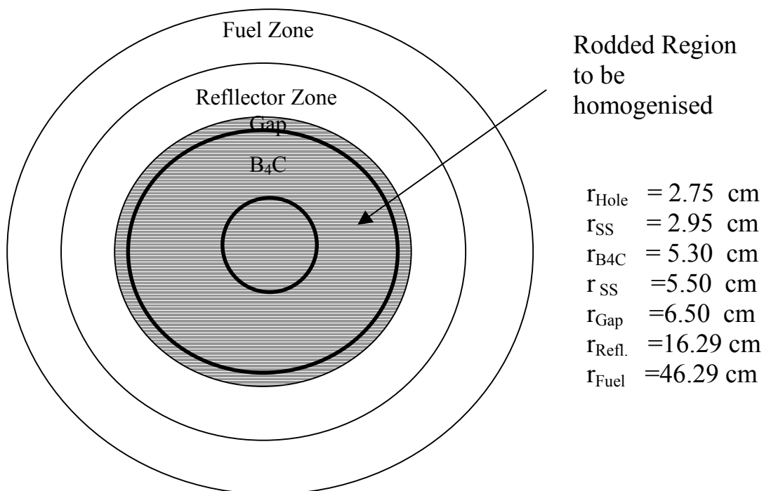
FIG. 4.47. 1-d Cylindrical Model of the CR-Cell for TOTMOS.
