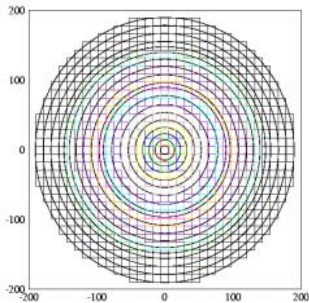
FIG. 4.24. Reactor channels and assigned rings to correspond with the 2D R-Z THERMIX model.
