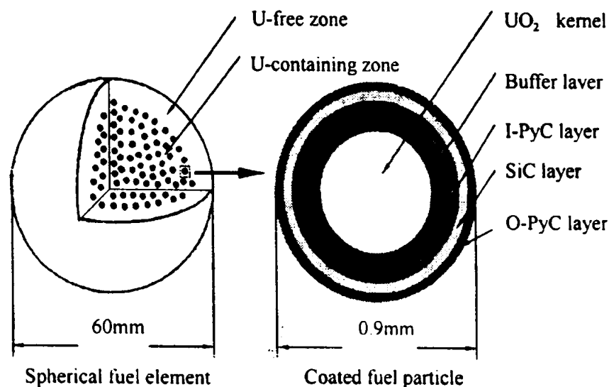
FIG. 4.8. HTR-10 spherical fuel element [4-6].
