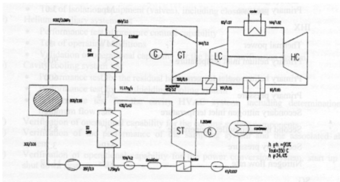
FIG. 4.5. Flow scheme for the steam turbine/gas turbine combined cycle.
