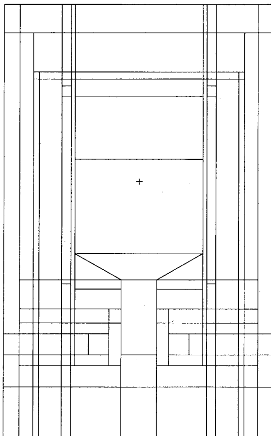
FIG. 4.32. Vertical Cross-sectional View of the MCNP Model of HTR-10.
