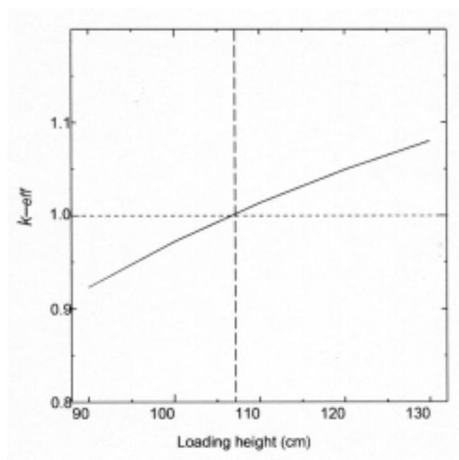
FIG. 4.16. Calculated K_{eff} vs. loading height for the HTR-10
