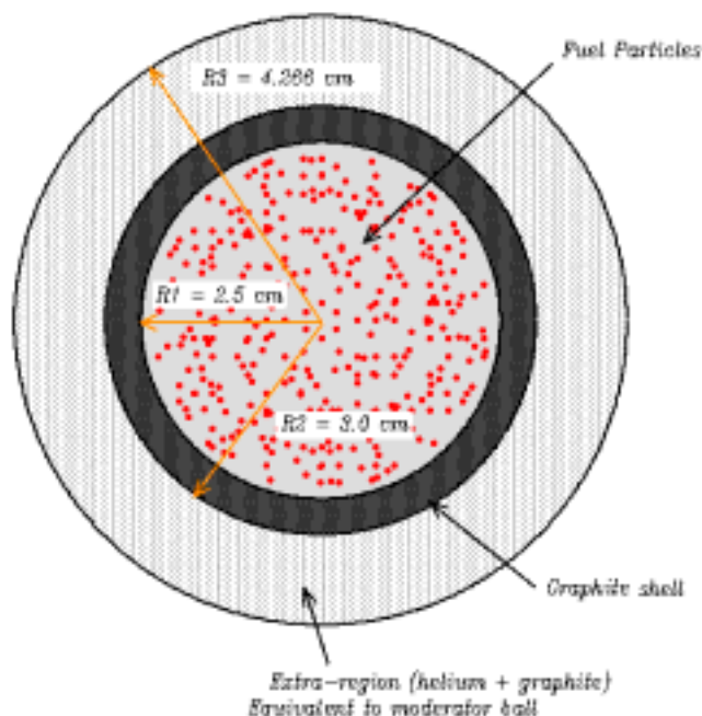
FIG.4.40. Spherical Fuel Pebble Model in APOLLO2.
