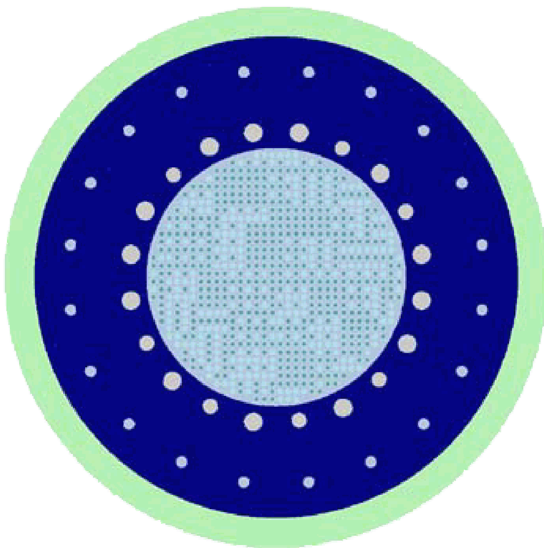
FIG. 4.37. Horizontal cross sectional view of HTR-10 in SCALE4.4 model
