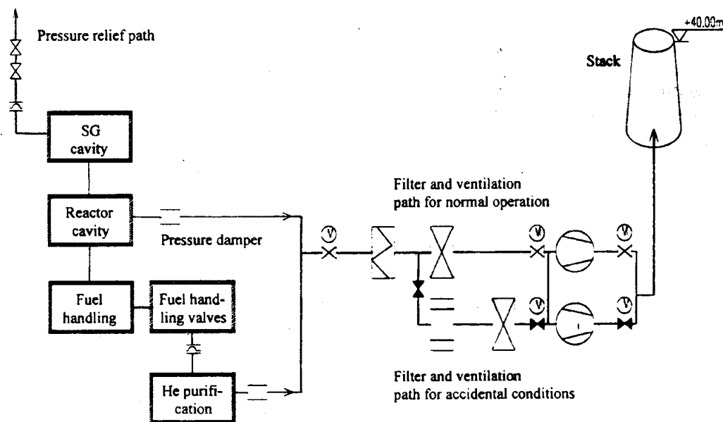
FIG. 4.3. Schematic of the HTR-10 confinement system [4-3].
