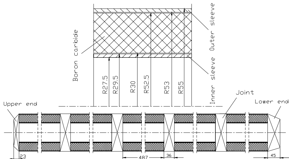
Fig.5 Simplified Structure of the HTR-10 Control Rod
