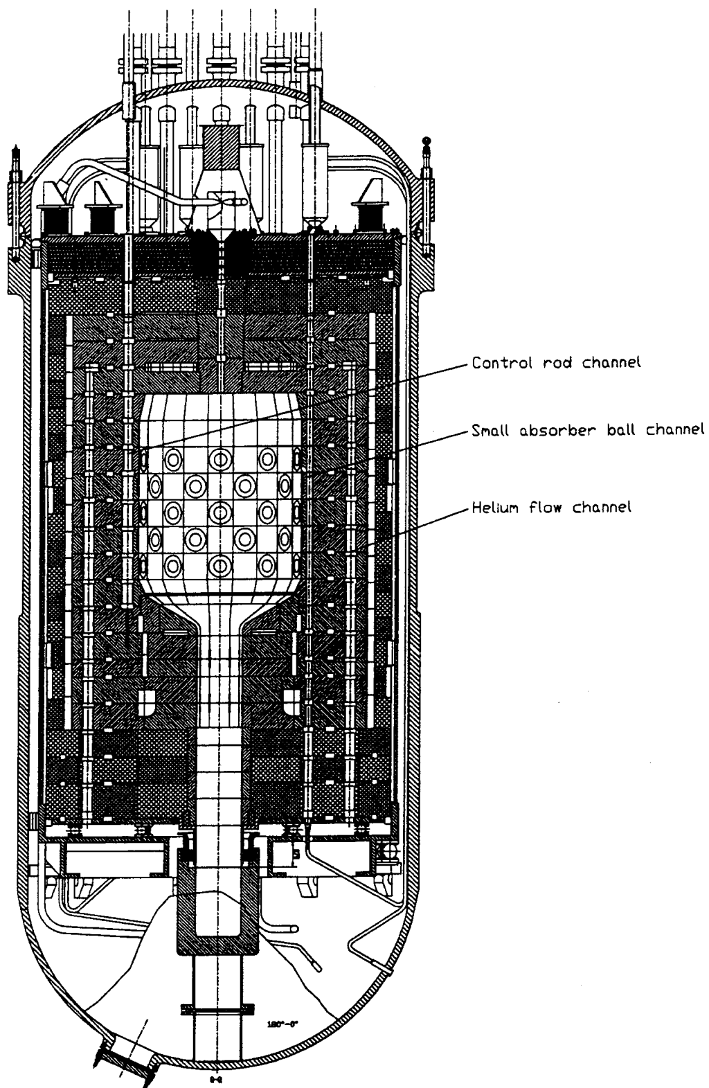
FIG. 4.6. HTR-10 reactor vertical cross-section.
