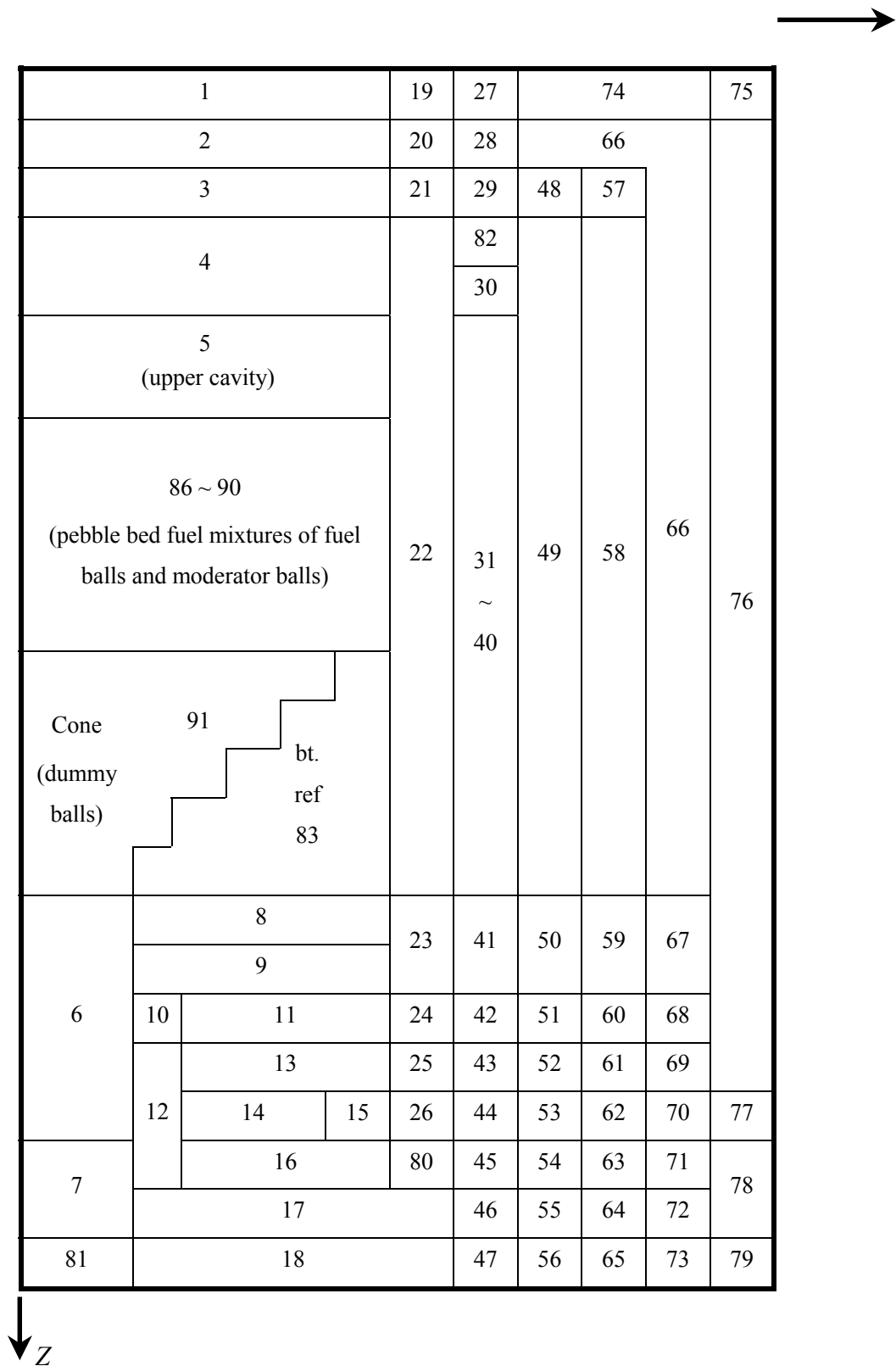
FIG. 4.15. HTR-10 Core calculation model in R-Z geometry.
