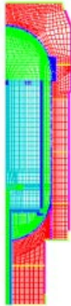
FIG. 3.57. 2D-reactor mesh.
