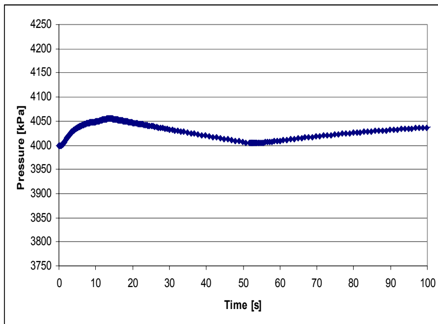
FIG. 3.47. HTTR system pressure (at PPWC circulator outlet).
