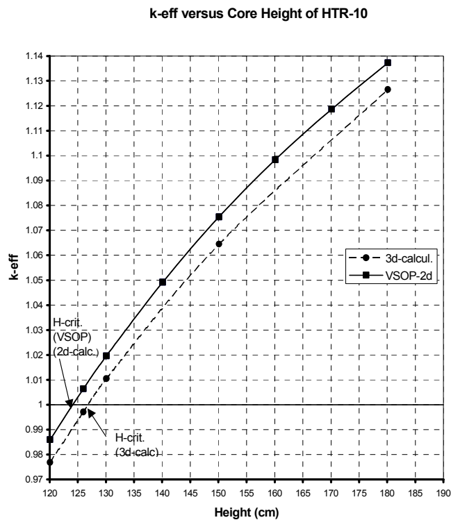
FIG. 4.48. k_{\text{eff}} versus Core Height of the HTR-10 (Original Benchmark Problem B1).
