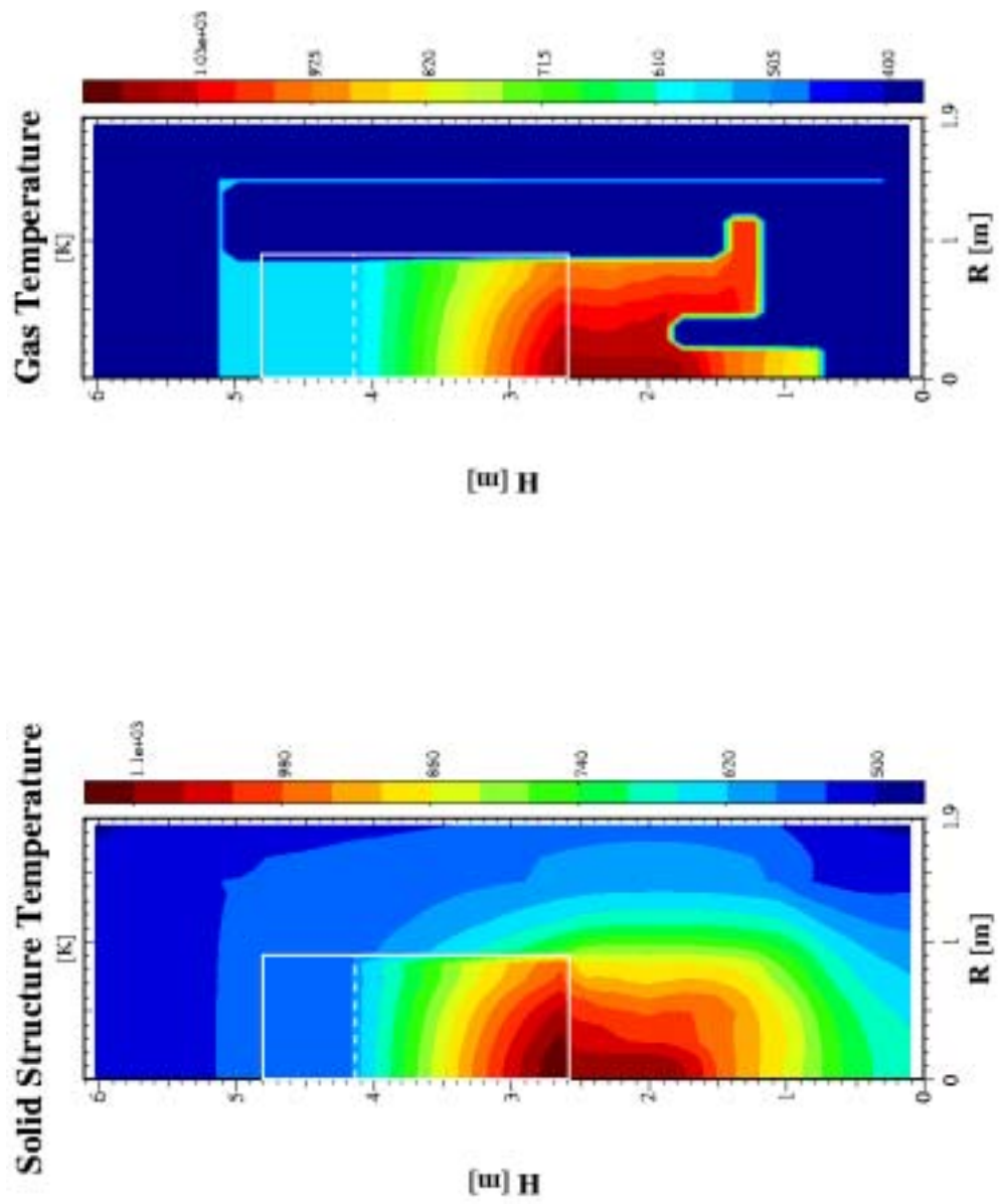
FIG. 4.28. and 4.29. Temperature distribution for the coolant and reactor structure in degrees Kelvin.
