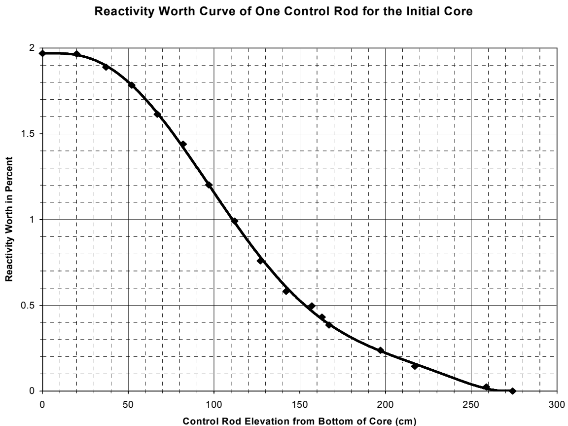
FIG. 4.49. Reactivity Worth Curve of One Control Rod (S1) for the HTR-10 Initial Core (Original Benchmark Problem B42).
