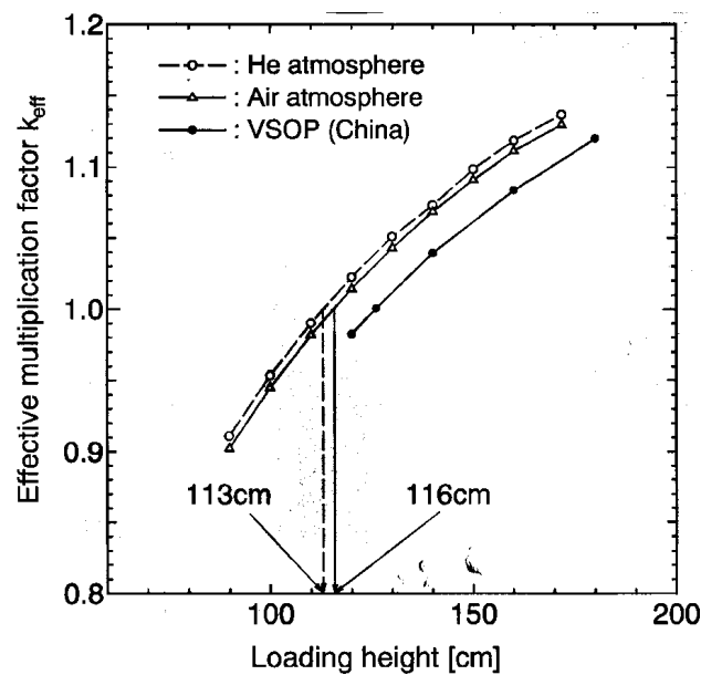
FIG. 4.18. Comparison with results from INET using VSOP.
