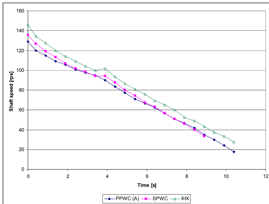
FIG. 3.36. Circulator shaft rotational speed – JAERI result used as input to Flownet Nuclear.
