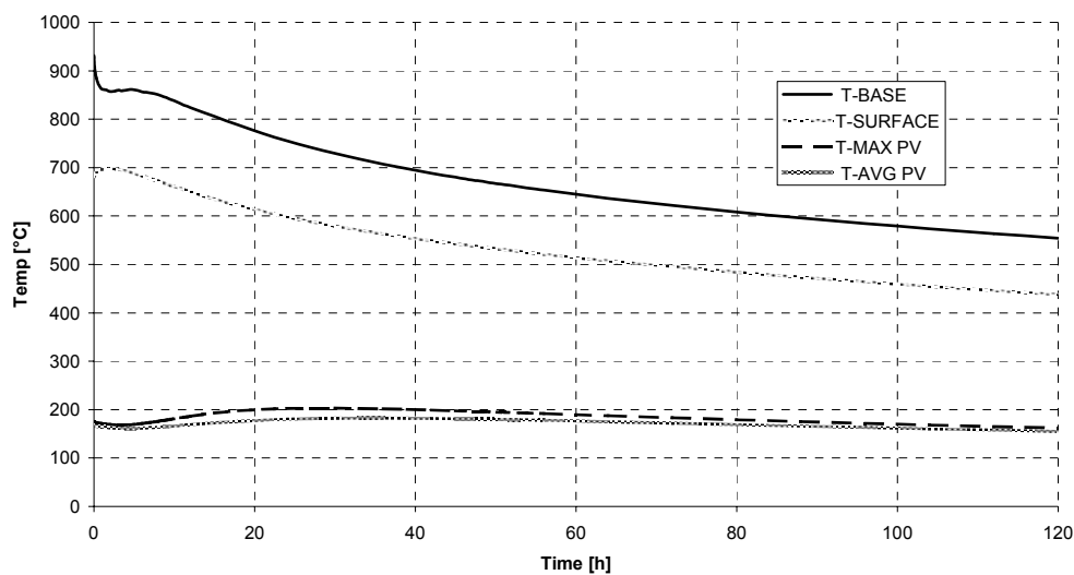
FIG. 4.53. Fuel and RPV temperature distribution following DLOFC.
