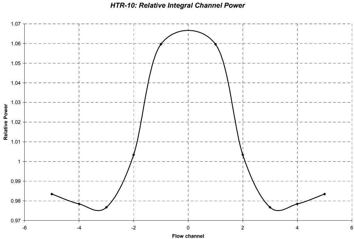
FIG. 4.52. Integral radial power distribution over the pebble flow channels.
