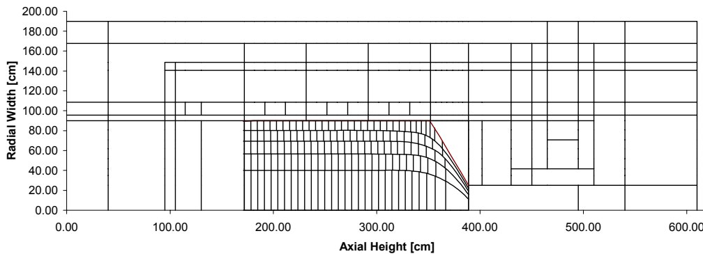
FIG. 4.55. HTR-10 loading to 1 st criticality.
