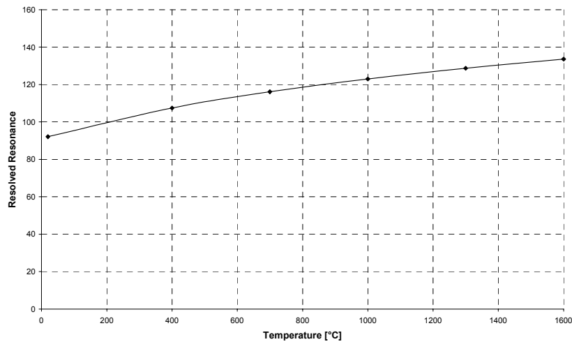
FIG. 4.51. Temperature-dependent resonance integral for 5g MH /FS and 18% enrichment.
