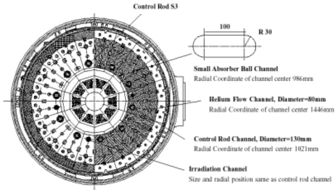
FIG. 4.7. HTR-10 reactor horizontal cross-section.
