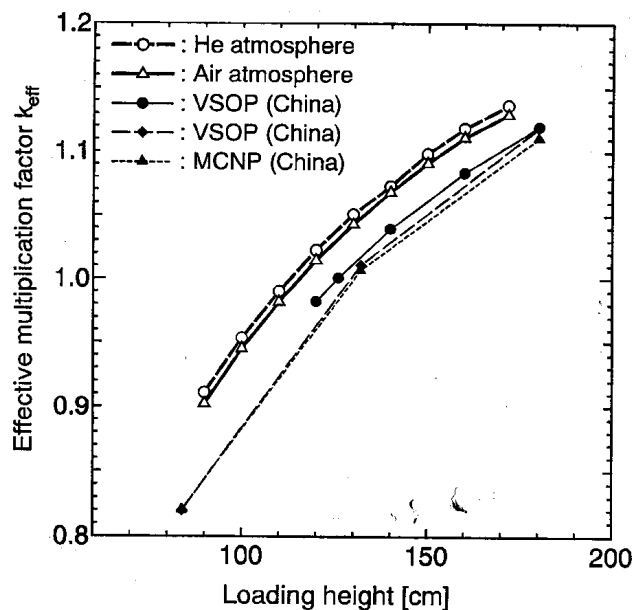
FIG. 4.19. Comparison with INET for K_{eff} vs. loading height (MCNP and VSOP).
