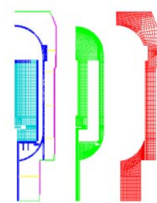
FIG. 3.58. Solid, helium and air related meshes.
