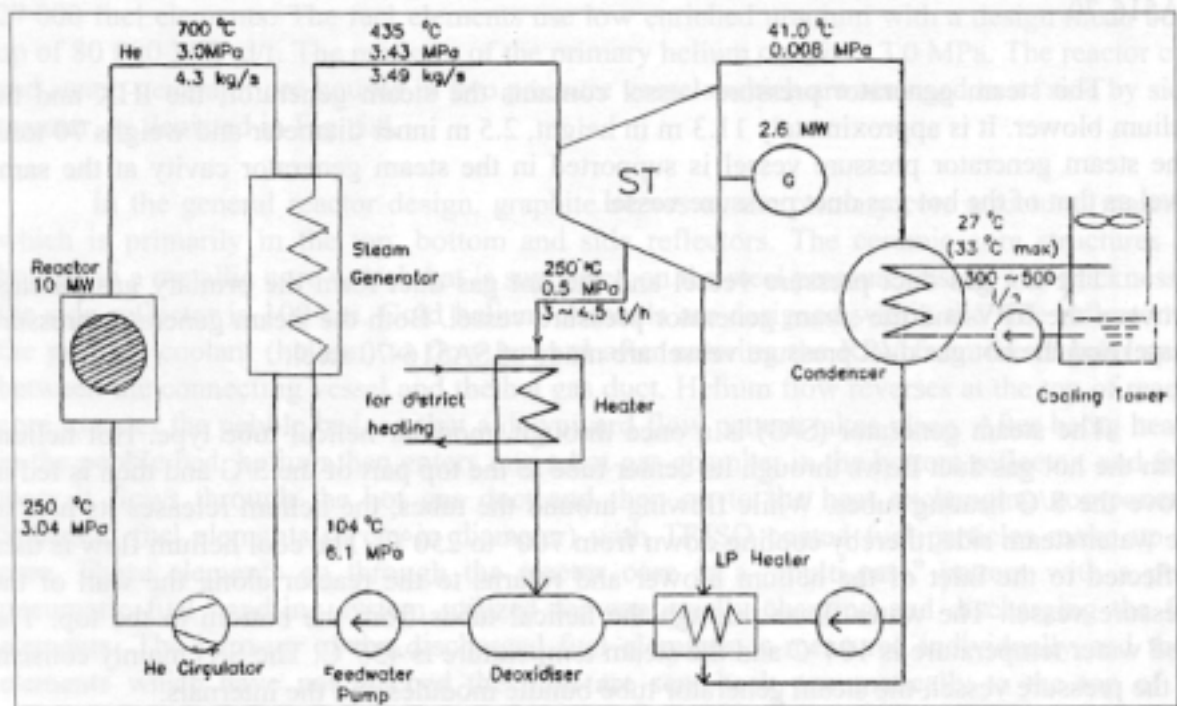
FIG. 4.4. Flow diagram for the first phase of HTR-10 operation.
