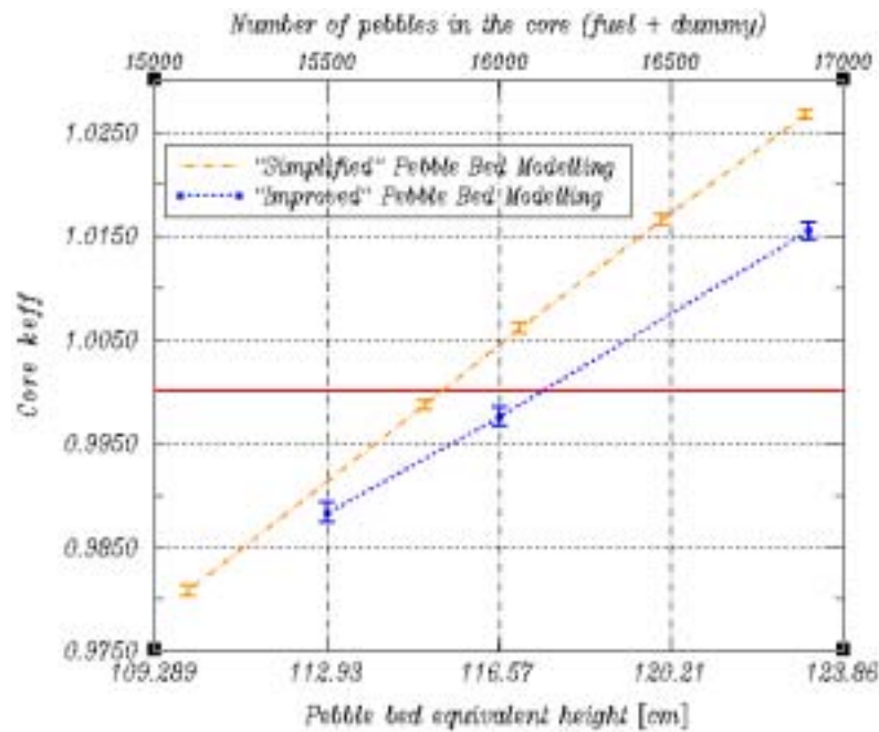
FIG. 4.45. Calculated k_{eff} vs loading height for HTR-10 initial criticality.
