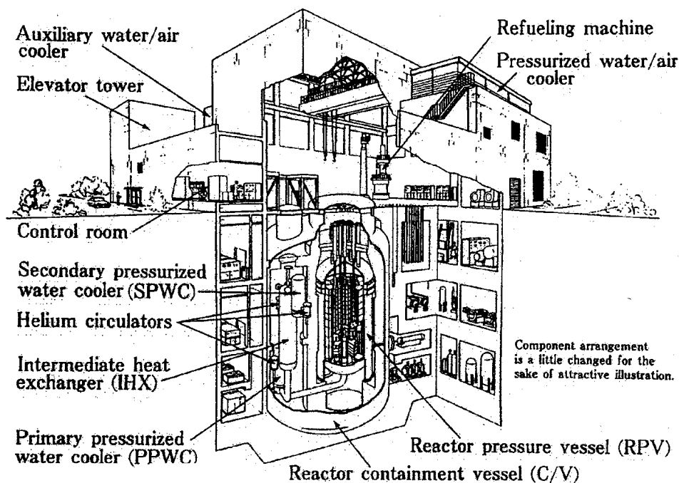
FIG. 2.2. HTTR reactor building.
