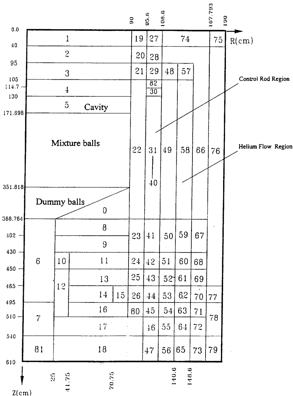
FIG. 4.10. HTR-10 core physics calculation model (see Table 4-3).
