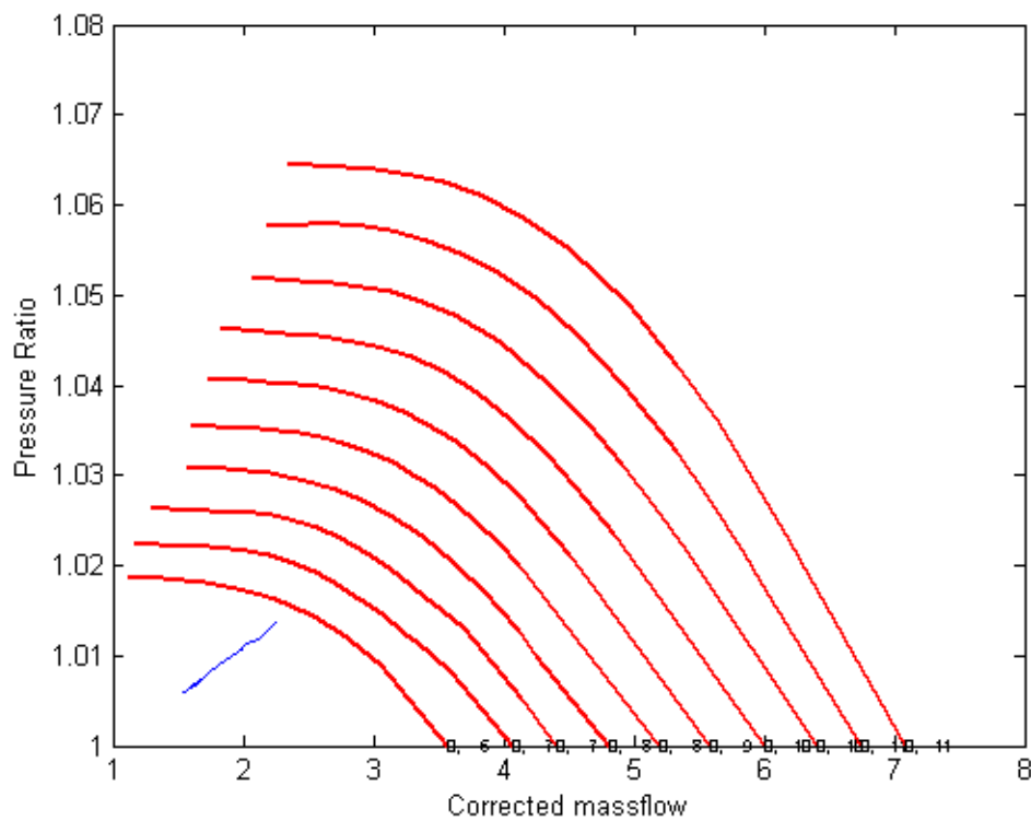
FIG. 3.37. Locus plot of circulator coast down on a Pressure ratio vs. corrected mass flow rate map.
