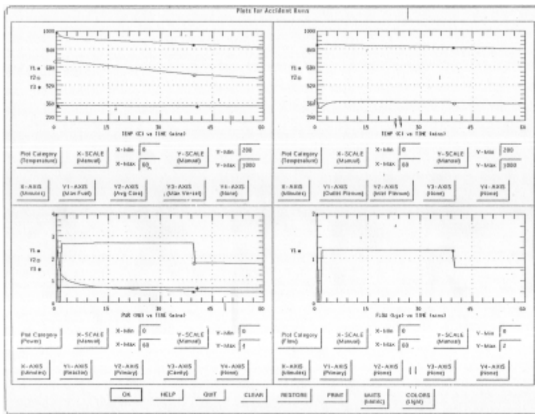
FIG. 3.51. HTTR-LC Benchmark: LOSP from 100% Power (1 hr).
