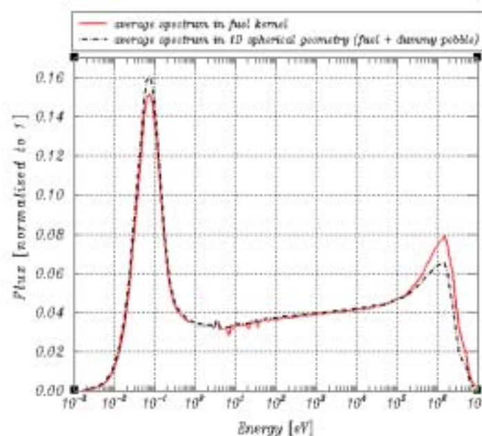
FIG. 4.41. Average neutron spectrum in fuel kernel and in fuel pebble surrounded by extra-region.
