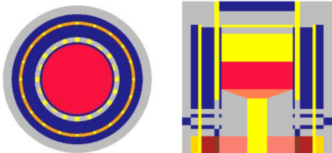
FIG. 4.42. Core modeling in Monte-Carlo code TRIPOLI4 (“Simplified PB modeling”).
