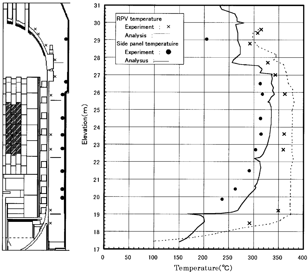
FIG. 3.6. Temperature Profiles on the RPV and Side Panel at 30 MW.
