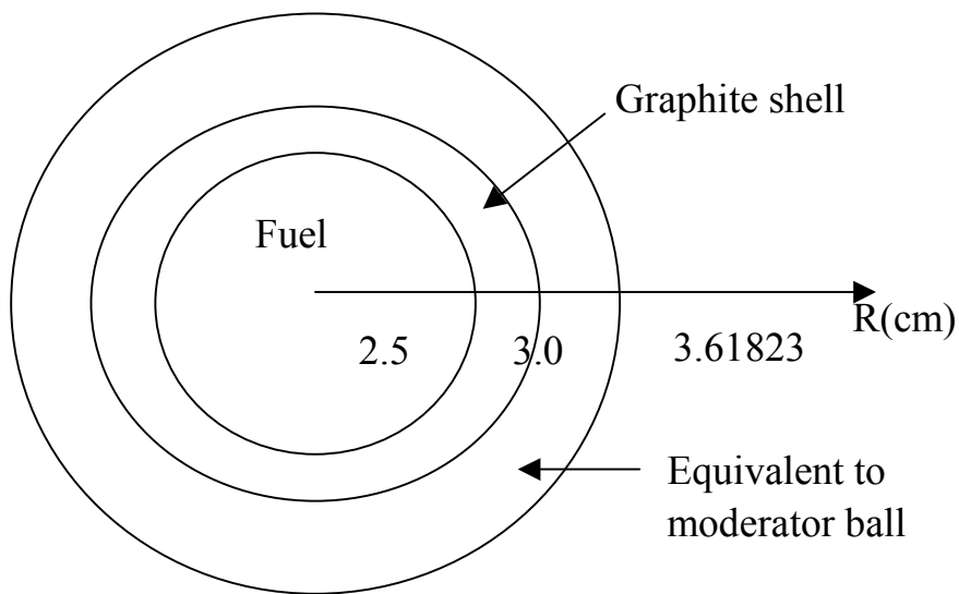
FIG. 4.11. Spherical cell model for calculation of thermal spectrum.
