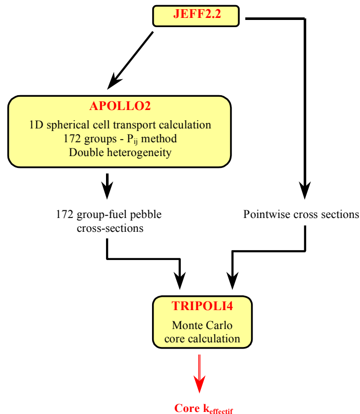
FIG. 4.39. Description of the Transport – Monte-Carlo calculation scheme.
