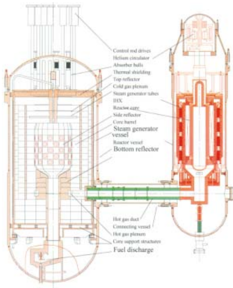
FIG. 4.1. HTR-10 primary system configuration [4-1].
