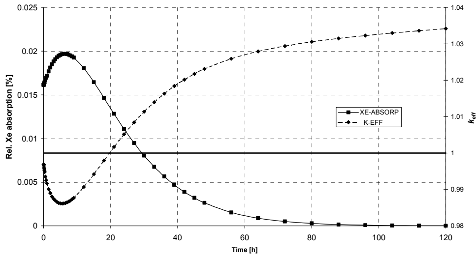
FIG. 4.54. Xenon absorption versus k_{eff} .
