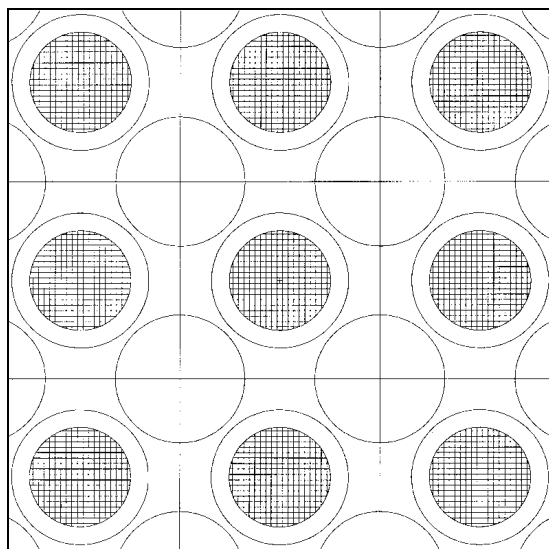
FIG. 4.36. A Horizontal Cross-section through the MCNP Model of the Pebble-Bed Core.
