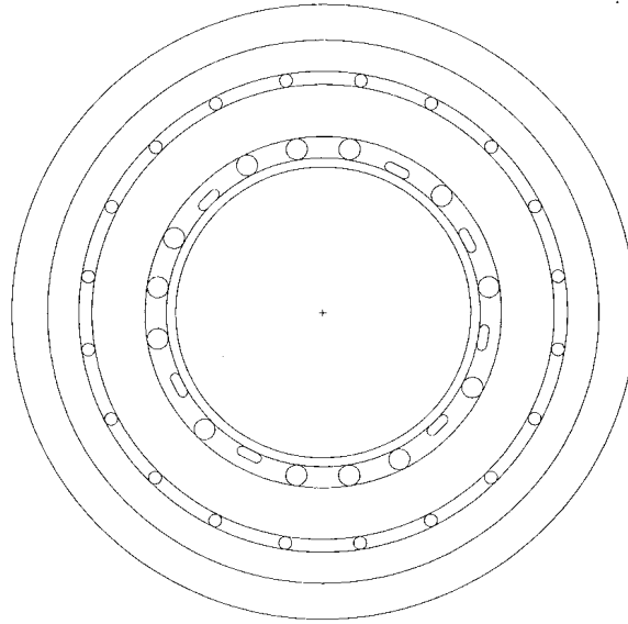
FIG. 4.33. Horizontal Cross-sectional View of the MCNP Model of HTR-10.
