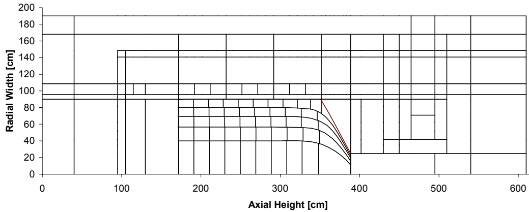
FIG. 4.50. VSOP Model for the HTR-10 in 2-D.
