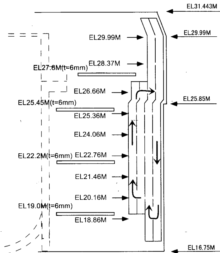
FIG. 3.3. Assumed flow passage in side panel
