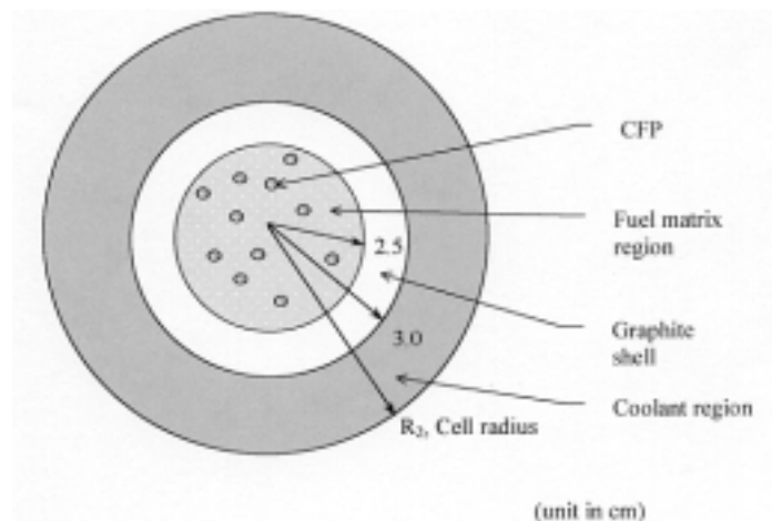
FIG. 4.14. The model of fuel cell used in WIMS/D4 and SRAC.
