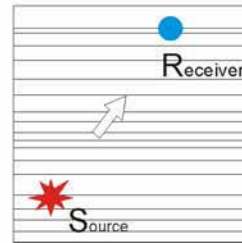
LAYERED HALF-SPACE
