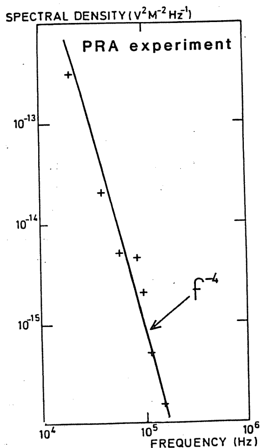
Fig. 2: Power spectrum detected by the Planetary Radio astronomy Instrument aboard Voyager 2 at Uranus ring plane crossing. This provided dust parameters (from [12]).
