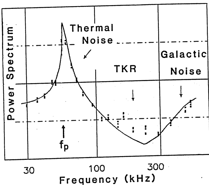
Fig. 1: Example of voltage power spectrum detected by the radio experiment aboard ICE in comet Giacobini-Zinner. A spectroscopy of all the spectra acquired gave the profile of electron density and temperature (and parameters of the hot electrons) (from [14]).
