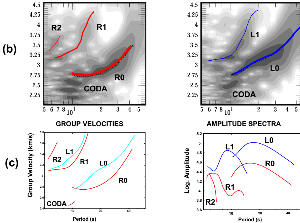
Figure 8. The earthquake at Iran-Turkmenistan border recorded at AAK (epicentral distance 1560 km): (a) records; (b) FTAN diagrams; (c) group velocities and amplitude spectra. Strong higher modes and fundamental modes of Rayleigh and Love waves are present.
