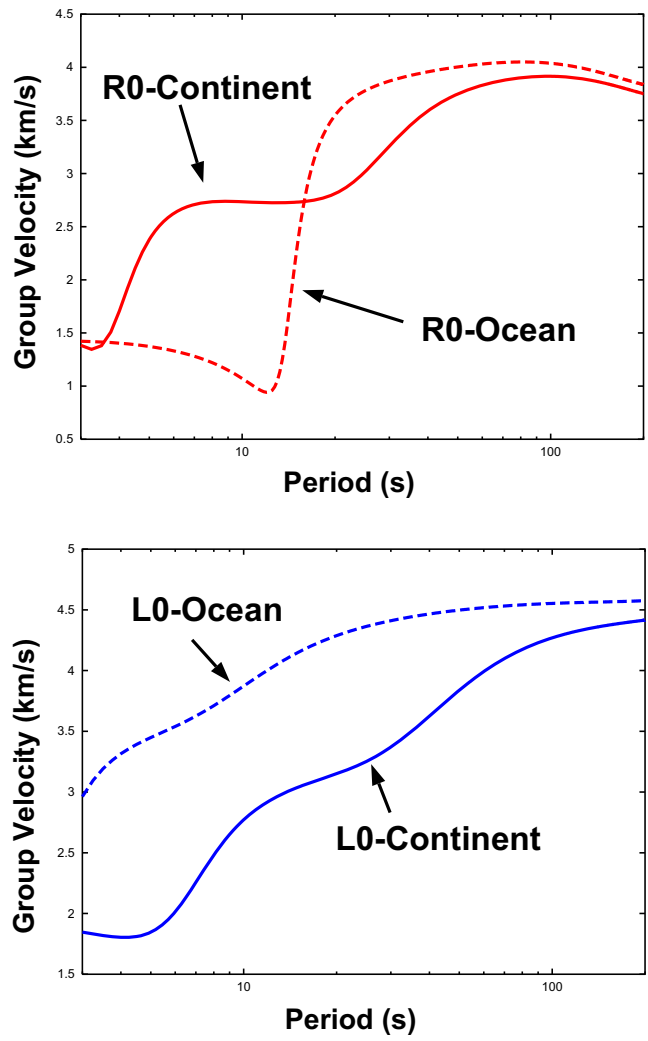
Figure 9. Group velocities of fundamental Rayleigh and Love waves along continental and oceanic paths.
