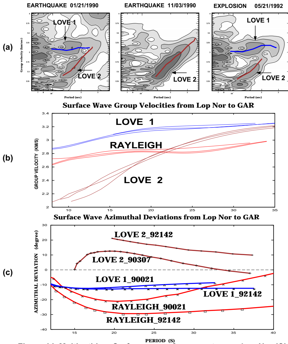
Figure 14. Multipathing. Surface waves from events near Lop Nor (China) recorded at GAR (Tadjikistan): (a) FTAN diagrams of the transverse component. (b) Group velocities of observed surface waves. (c) Azimuthal deviations of observed waves.
