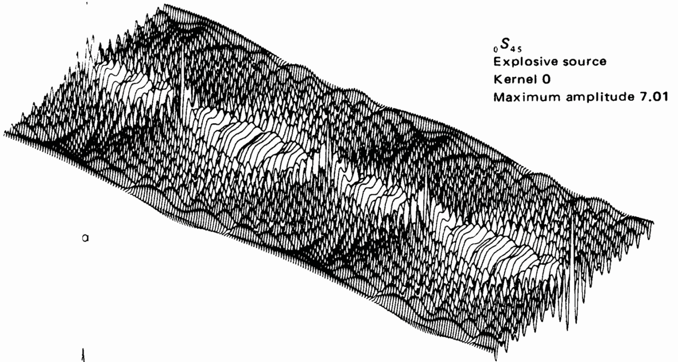
Figure 7b: Representations of the global sensitivity of the modes {}_0S_{10} and {}_0S_{45} (Woodhouse and Girnius, 1982)
