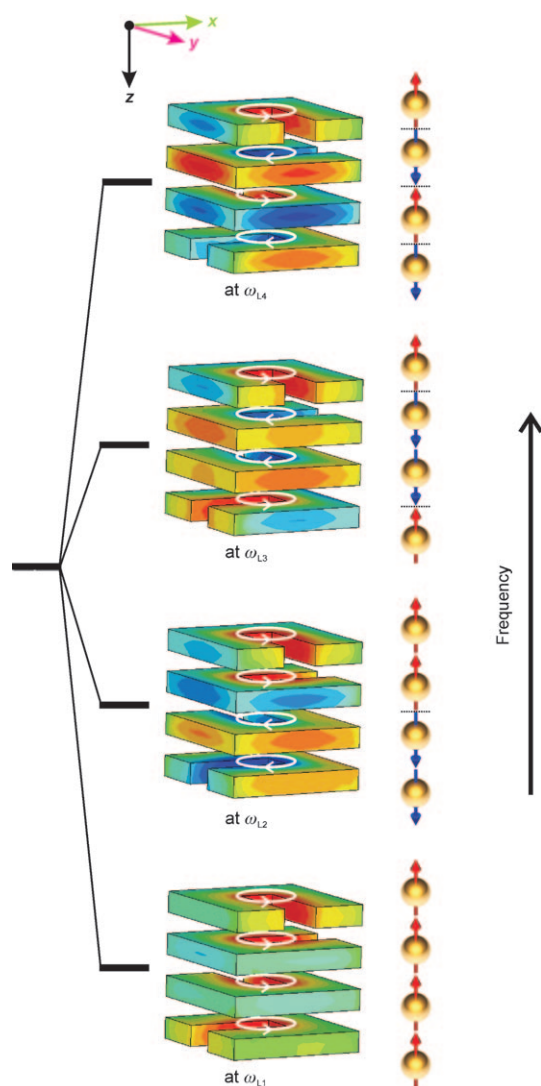
Figure 17. Resonance diagram depicting the hybridization of the modes for the four-layer twisted split-ring metamaterial and the simulated magnetic field distributions of H_z at the corresponding resonance frequencies. The light is incident along the z direction and linearly polarized along the x direction. Red denotes a positive H field, and blue denotes a negative H field. The “spin” symbols (right) represent the magnetic dipole moments for the respective modes. The number of magnetic field nodes (dotted lines) rises with increasing resonance frequencies. Reprinted from Ref. [42], with permission from the Optical Society of America.
