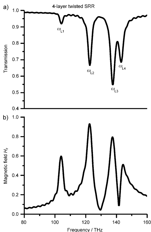
Figure 16. a) Simulated transmission spectrum (L1–L4 = longitudinally coupled split rings) and b) field strength of the H_z component of the four-layer twisted split-ring metamaterial. The probe for the H_z component is positioned at the center of the uppermost split ring. Reprinted from Ref. [42] with permission from the Optical Society of America.
