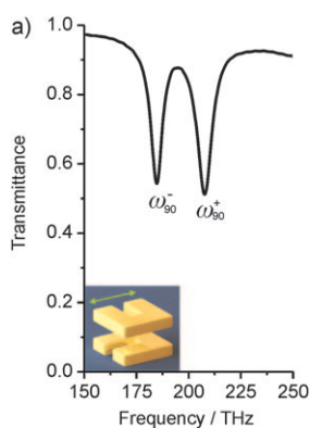
Figure 11. a) Simulated transmittance spectra for the 90°-twisted split-ring dimer metamaterial. The size of each split ring is 230×230 nm 2 . The arm width is 90 nm and the gold thickness is 50 nm. The vertical spacing between the two split rings is 50 nm. The structure is embedded in air. The normally incident light is polarized along the gap-bearing side of the top split ring. b) Schematic diagram of the alignment of the magnetic dipoles in the two split rings at the respective resonance frequencies. The solid arrows represent the magnetic dipole moments. Reprinted from Ref. [38], with permission from the Nature Publishing Group.
