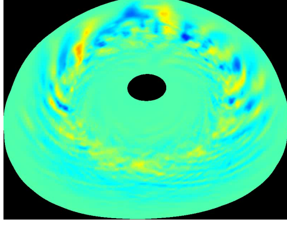
Full-torus gyrokinetic plasma turbulence simulation with GENE (TCV tokamak, Lausanne)
