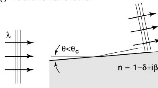
(f) Total external reflection
