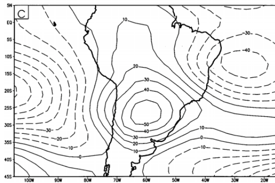
Eddy Geopotential height at 200hPa
