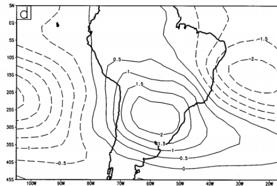
Eddy temperature at 300hPa
