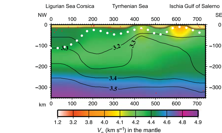
Fig. 5 Tyrrhenian I section: V_s and density model along a NW–SE profile from Ligurian Sea to Gulf of Salerno. The labelling is the same as Fig. 1. This profile samples the Tyrrhenian Sea along its supposed direction of opening. It is clearly characterized by a south-eastward emerging LVZ from about 100 km of depth beneath Ligurian Sea and northern Corsica to about 30 km in the Ischia volcanic zone. The V_s model, the seismicity distribution and the so inferred lid–LVZ boundary fairly agree with extensive ‘boudinage’, at different scales (Ramsay and Huber, 1983, and references therein) that characterized the evolution of the basin still going on in present days. The northern part of the basin is characterized by relatively low-density mantle, in contrast with the southern active part, where density increases, as seen in other sections. Again, a relatively low density mantle is found east of Ischia, in the vicinity of Apennines subduction.
