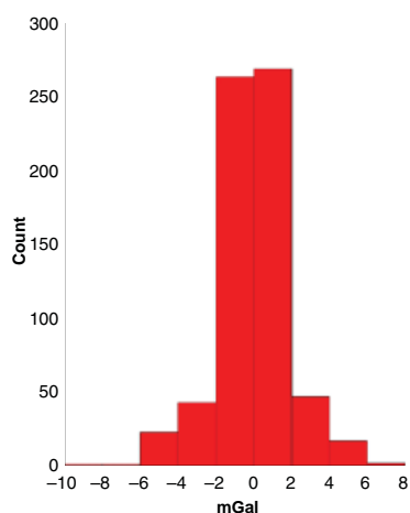
Fig. 4 Density model uncertainties: Histogram of the differences between observed and model predicted gravimetric anomalies. The maximum value is 8 mGal, consistent with the quality and the noise level of the data.
