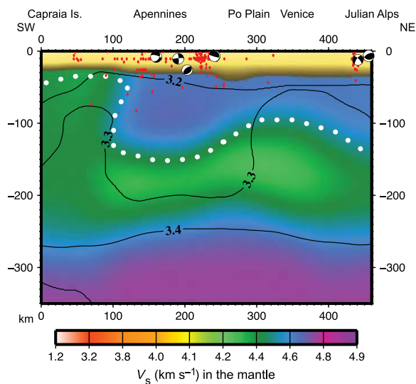
Fig. 7 Adria43-46 section: V_s and density model along a SW–NE profile from Capraia Island to Julian Alps. The labelling is the same as Fig. 1. The pronounced high-velocity, almost vertical, slab represents Apennines subduction consistent with significant seismicity at intermediate depth. To the West, a low-velocity asthenospheric mantle wedge, mainly aseismic, is present. To the East, a high velocity lid about 100 km thick extends towards the NE-dipping Alpine subduction, marked by the shallow to intermediate depth seismicity in the right part of the section. The bottom of the lid is well marked by a LVZ. Striking features of density model are the negative density anomaly beneath Apennines and Julian Alps, with the exception of the relatively high-density value found beneath Tuscany, probably related to mantle wedge. Po plain and Northern Adriatic are instead characterized by relatively high-density mantle at depths ranging from 60 to 200 km.
