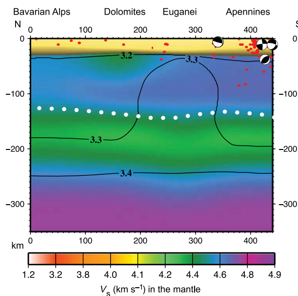
Fig. 9 Transalp section: V_S and density model along an N–S profile from Bavarian Alps to Northern Apennines. The labelling is the same as Fig. 1. The low-angle subduction of the European plate below the Adriatic plate is fairly well evidenced by gently N–S dipping high-velocity lid and in accordance with scarce shallow seismicity and almost absent intermediate depth seismicity, as seen in Ecors section. A relatively low velocity lid is found beneath Dolomites, just below the Moho. The bottom of the lid is found at about 120–140 km of depth and overlies a well-marked LVZ in the asthenosphere. In the southernmost part of the section, Apennines subduction is delineated by high seismicity that reaches intermediate depth. The prominent high-density body, as shallow as 40 km of depth, below Venetian plain, may be a signature of the Euganei Hills magmatic activity.
