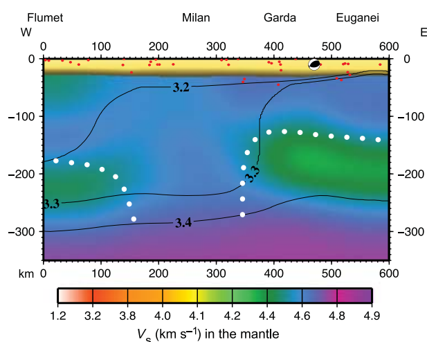
Fig. 6 Ecors section: V_s and density model along a W–E profile from Flumet (western Alps) to Euganei Hills. The labelling is the same as Fig. 1. Striking feature of the section is the subduction of the European plate below the Adriatic plate, with deep ‘lithospheric roots’ below Milan, represented by high-velocity lid, well in agreement with what was shown by Mueller and Panza (1986). In contrast to Apennines subduction, no intermediate depth seismicity is observed in western Alps. To the West the LVZ is found at a depth of about 180 km. To the East, a prominent LVZ marks the Euganei Hills magmatic zone below a depth of about 130 km. The subducting lid is characterized by negative density anomaly, whereas a positive density anomaly is seen beneath Euganei Hills, as shallow as 30 km.
