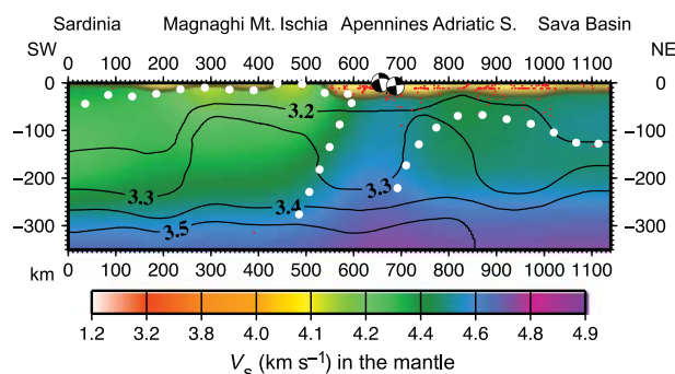
Fig. 1 Sardinia–Balkans section: V_S and density model along a SW–NE profile from southern Sardinia to Sava Basin. V_S distribution is given by the color scale while continuous contour lines refer to density ( \text{g cm}^{-3} ). Seismicity (red dots) and focal mechanisms of major events ('beach balls' plotted in map view) are shown as well. Dotted white lines delineate the lid-LVZ margin. Please refer to online version for interpretation of references to color. This profile samples the main geological and tectonic features of the central Mediterranean: (i) the southernmost part of the Corsica–Sardinia block characterized by scarce seismicity and rather low velocities in the lid, down to about 70 km of depth; (ii) the active part of Tyrrhenian basin, characterized by an asthenospheric LVZ emerging eastward from 70 km depth in the western part of the basin to 30 km depth below Ischia and well visible lithospheric 'boudinage'; (iii) the westward dipping Apennines, characterized by high seismicity even at intermediate depth and high velocities; (iv) a relatively low velocity and mostly aseismic lid beneath the Adriatic sea (as in section Adria42); (v) eastward dipping Dinaric slab, characterized by relatively high velocity and intermediate depth seismicity. Relatively low-density mantle is seen beneath Corsica–Sardinia block, Apennines and Dinarides, whereas a prominent positive density anomaly is found below Tyrrhenian and Adriatic seas.
