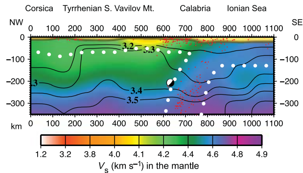
Fig. 2 Tyrrhenian II section: V_S and density model along a NW–SE profile from southern Corsica to Ionian Sea. The labelling is the same as Fig. 1. Prominent feature of the section is the high velocity body representing subducting lid beneath Calabrian Arc, seismically active at all depths. To the west, the active part of the Tyrrhenian is marked by a lid at about 60–70 km thick, with some very low velocity soft mantle lid beneath volcanic areas. Lid is slightly thicker beneath Sardinia–Corsica block and reaches about 90 km of thickness. To the east of the Calabrian Arc, the Ionian lid is about 130 km thick, and the underlying mantle is relatively faster than the Tyrrhenian one. Generally, the mantle velocity is higher in the Ionian plate than in the Tyrrhenian basin. A prominent negative density anomaly characterizes the subducting slab and the Sardinia–Corsica block, whereas a positive anomaly characterizes both the active Tyrrhenian, with a 3.3 \text{ g cm}^{-3} density of about 60–70 km of depth, and the Ionian mantle, with a 3.3 \text{ g cm}^{-3} density reaching about 80 km of depth and a 3.4 \text{ g cm}^{-3} density at about 170 km of depth.
