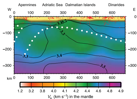
Fig. 8 Adria42 section: V_s and density model along a W–E profile from central Apennines to Dinarides. The labelling is the same as Fig. 1. In this section, as in section Crop03, Apennines slab is marked by a high velocity almost vertical body, with some intermediate depth seismicity reaching about 60 km of depth. To the West, the low velocity at a depth of about 50–100 km, just above the sinking slab, is probably related to mantle wedge dynamics (e.g. dehydration). To the east, a relative low velocity, mainly aseismic, mantle lid extends for about 100 km just beneath the Adriatic crust. In the easternmost portion of the section, an eastward thickening lid is well marked by high velocity and intense intermediate depth seismicity, in fair agreement with a low angle Dinaric slab. Prominent negative density anomalies characterize both the Apennines and Dinarides at depth between 100 and 200 km, whereas high-density material seems to be related to the Adriatic plate, both in the lid and in the asthenospheric LVZ.
