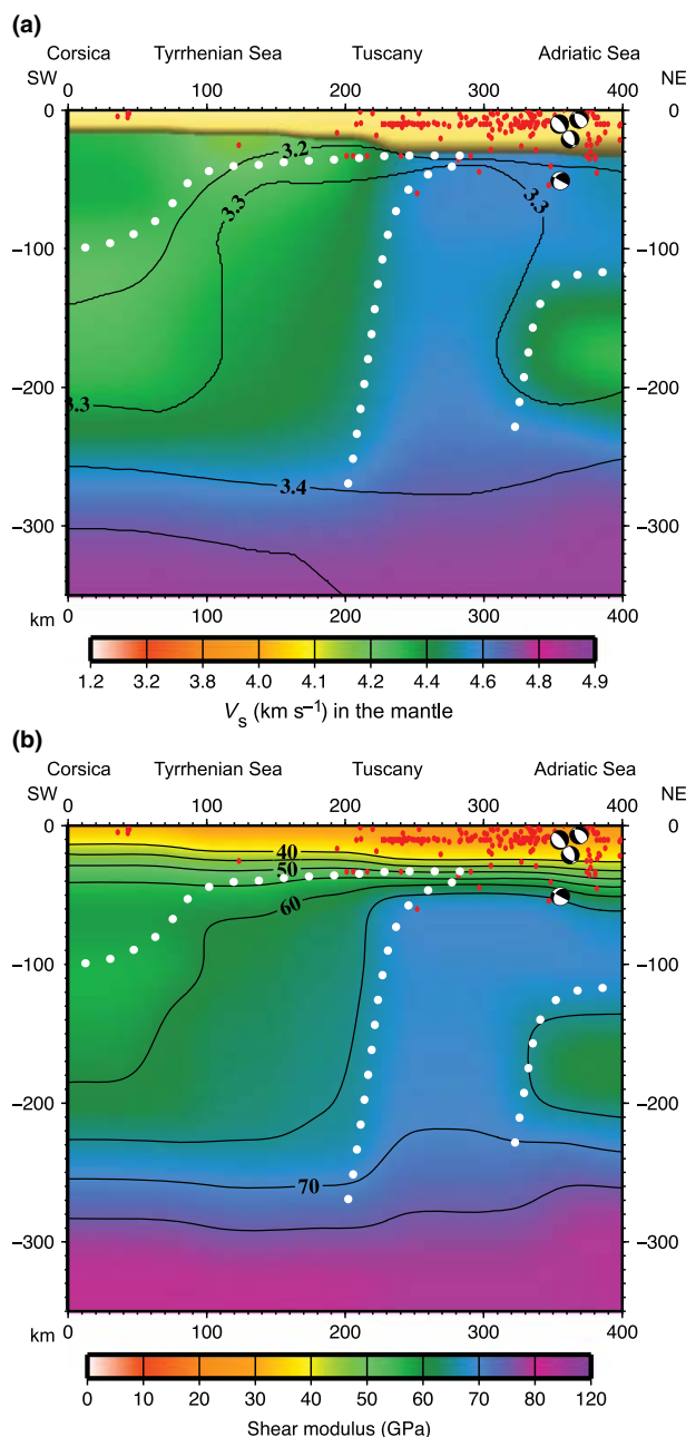
Fig. 10 Crop03 section: (a) V_s and density model along a SW–NE profile from northern Corsica to Adriatic Sea. The labelling is the same as Fig. 1. The pronounced high-velocity, almost vertical, slab represents Apennines subduction. To the West, an asthenospheric LVZ emerging from about 100 km depth beneath Corsica to about 40 km depth beneath Tuscany clearly marks the bottom of the lid. To the East of the subduction, a high-velocity lid extends beneath Adria down to about 120 km of depth, lying on a well marked LVZ. A high density body is seen below Tuscany and in the subducting slab, whereas lower density characterizes both Corsica block and Adriatic mantle. (b) The shear modulus ( \mu ), in GPa, along the same section, gives a more clear-cut picture of the subducting slab.
