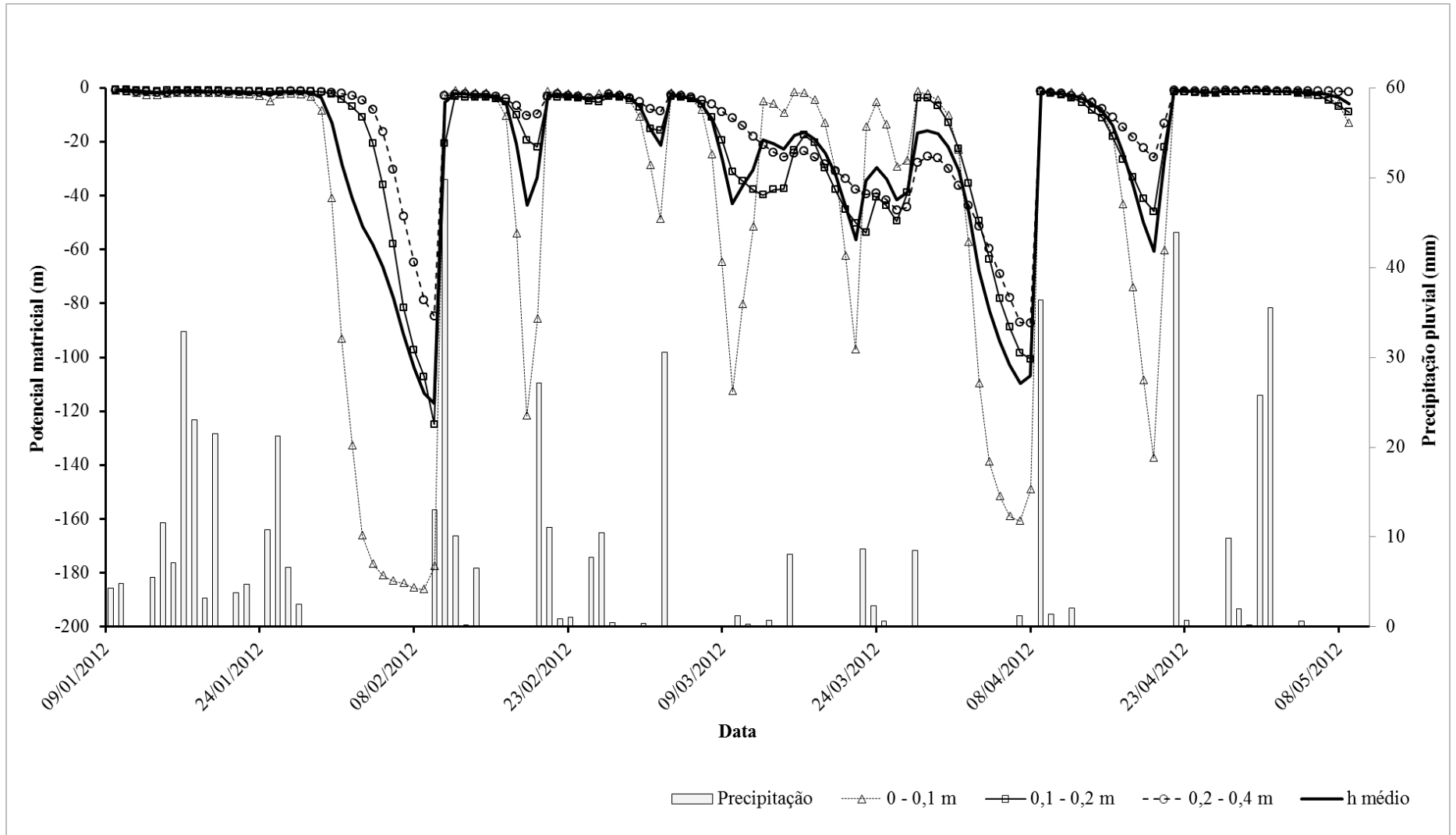
Figure 7. Matric potential h (m) measured by polymer tensiometers and rainfall (mm).
