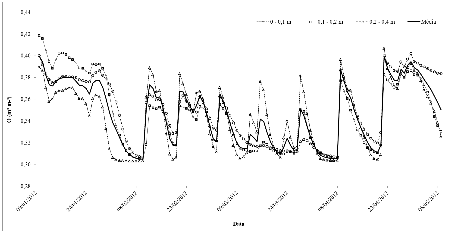
Figure 8. Soil water content for the layers 0-0.1 m; 0.1-0.2 m and 0.2-0.4 m and their average.
