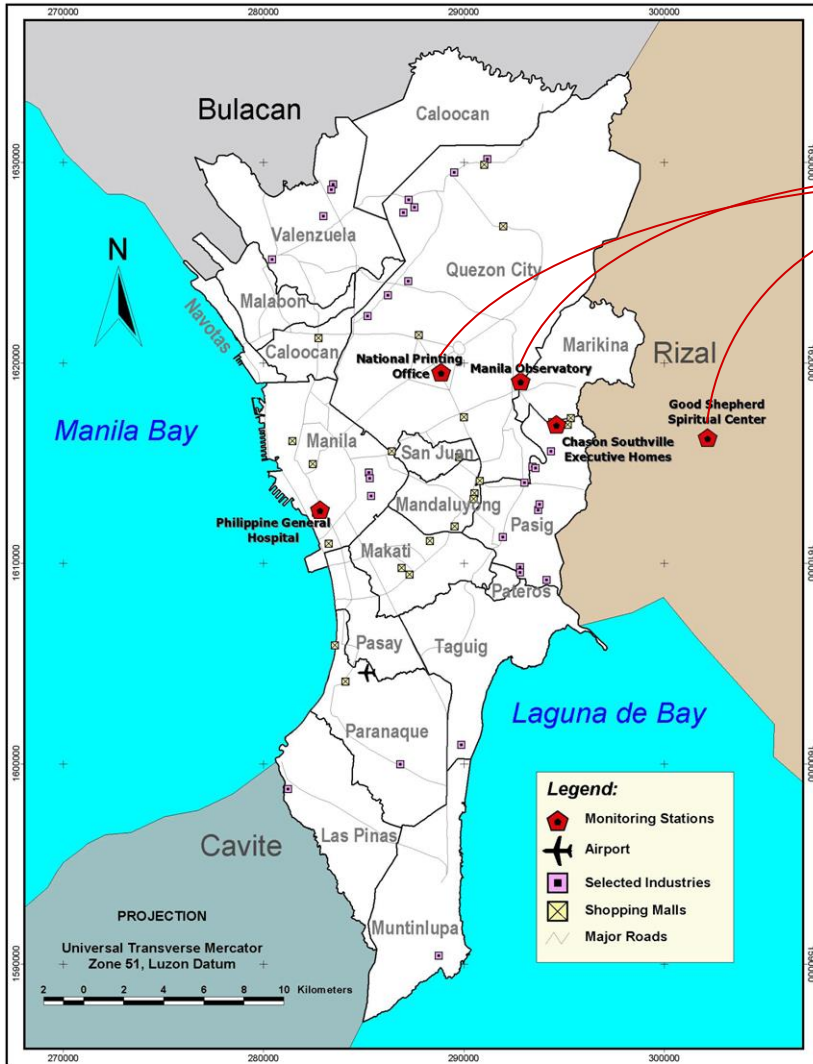
Manila Observatory Spatio Temporal Distribution of Fine Particulate Matter
