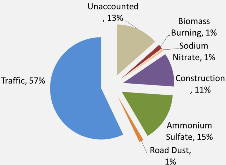
PMF Results (Manila Observatory) PM 2.5 , Dry Season
