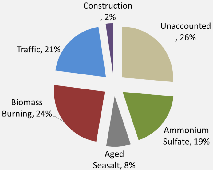
PMF Results (Manila Observatory) PM 2.5 , Wet Season
