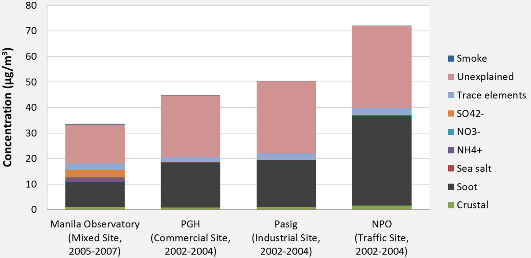
Reconstructed Mass of PM 2.5 Samples from 4 Metro Manila Sites
